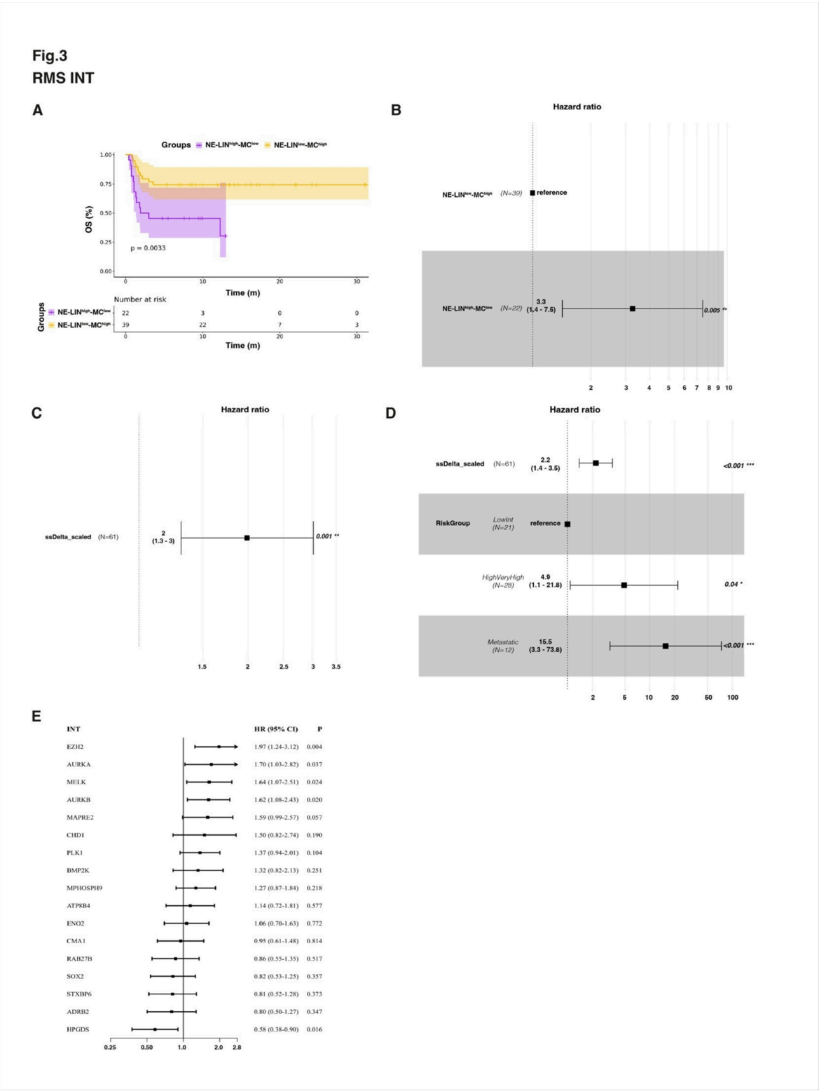
Figure 3 Prognostic association of the PAAS state in RMS. A. Kaplan-Meier curves for OS stratified by clusters in the INT dataset (n=61 patients). Log-rank test was used to evaluate statistical significance, and number
