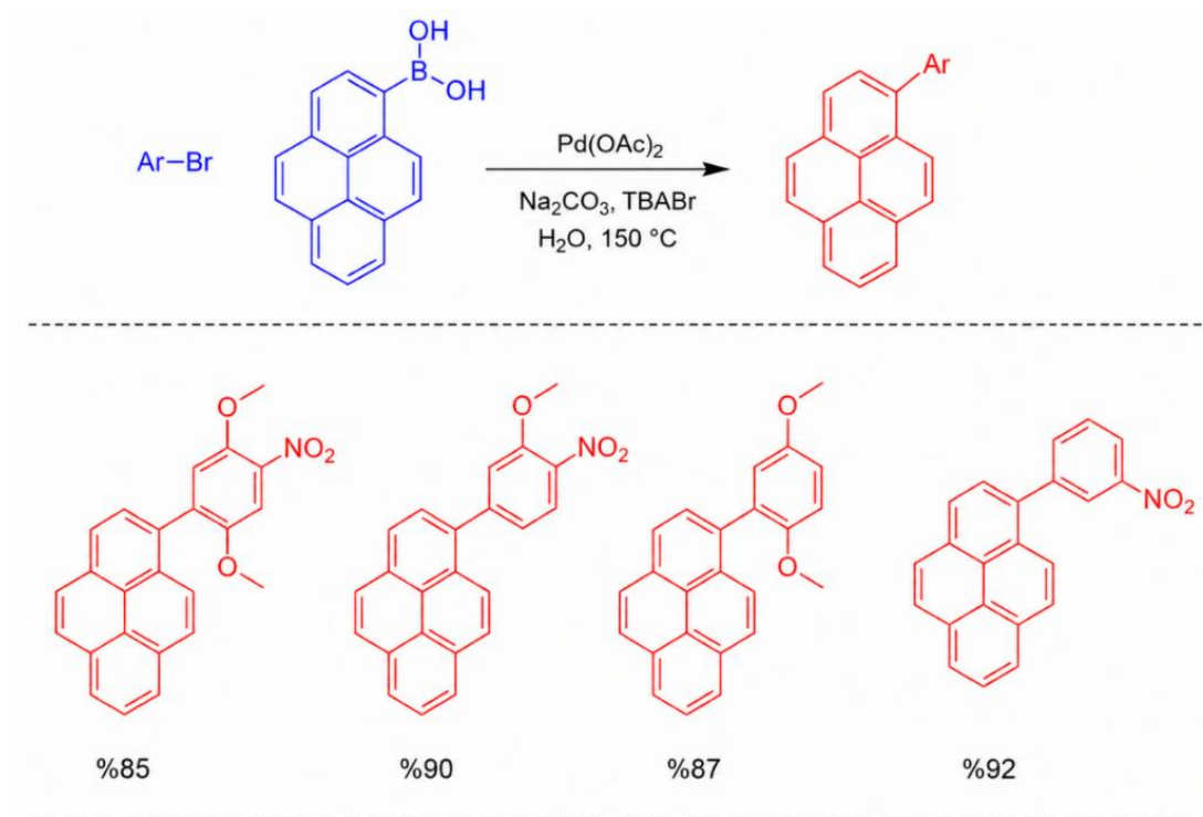
Scheme 2. Schematic illustration of the Suzuki cross-coupling synthesis route employed for the preparation of pyrene-based semiconductor derivatives. Pyren-1-ylboronic acid was reacted with different aryl bromide precursors in the presence of \text{Pd}(\text{OAc})_2 catalyst, \text{Na}_2\text{CO}_3 base, and TBABr additive in aqueous medium at 150\text{ }^\circ\text{C} , leading to the formation of conjugated pyrene derivatives with high isolated yields ranging from 85% to 92%. The synthesized molecular structures exhibit different substituent architectures designed to modulate intermolecular interaction, conjugation behavior, and optoelectronic properties of the resulting organic semiconductor systems.
