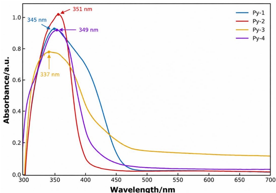
Figure 3. UV–Vis absorbance spectra of the synthesized pyrene-based semiconducting derivatives (Py-1, Py-2, Py-3, and Py-4) recorded in the 300–700 nm wavelength range. All samples exhibit pronounced near-UV absorption features associated with \pi – \pi^* electronic transitions within the conjugated pyrene framework. Variations in absorption maxima, spectral width, and low-energy absorption tails demonstrate clear substituent-dependent modulation of the optical response. Py-2 and Py-4 exhibit absorption maxima at approximately 351 and 349 nm, respectively, whereas Py-3 shows a comparatively blue-shifted maximum near 337 nm. These spectral differences indicate distinct electronic environments among the four derivatives and are considered together with the complementary PL and morphological analyses when evaluating substituent-dependent film organization.
