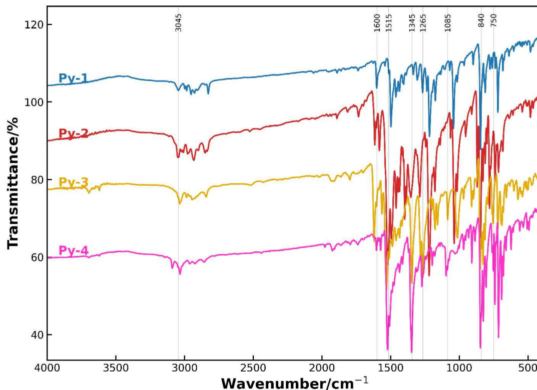
Figure 2. FTIR spectra of the synthesized pyrene-based derivatives (Py-1 to Py-4) recorded in the 4000–400 \text{cm}^{-1} region. The spectra exhibit the characteristic vibrational features of \pi -conjugated aromatic frameworks, including aromatic C–H stretching vibrations observed around \sim 3045 \text{ cm}^{-1} , aromatic C=C skeletal stretching modes near \sim 1600 \text{ cm}^{-1} , and prominent fingerprint-region bands between 1500–700 \text{cm}^{-1} associated with substituent-dependent ring vibrations, C–O/C–N stretching, and aromatic C–H out-of-plane deformation modes. The systematic variations in the fingerprint region confirm the successful structural modification of the pyrene backbone and the formation of distinct substituted pyrene architectures.
