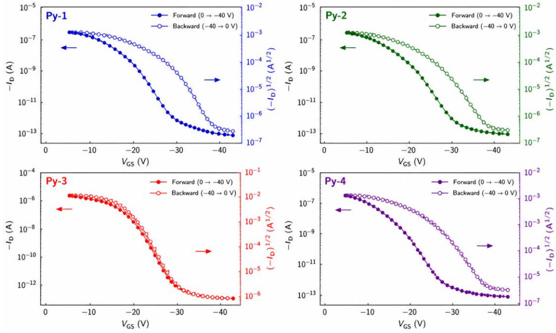
Figure 9. Transfer characteristics of the OFET devices based on Py-1, Py-2, Py-3, and Py-4 semiconductor layers measured at a constant drain voltage of V_{DS} = -30 V. The transfer curves were recorded during forward ( 0 \rightarrow -40 V) and backward ( -40 \rightarrow 0 V) gate-voltage sweeps to evaluate the p-channel switching behavior and gate-bias hysteresis of the devices. Filled and open symbols represent the forward and backward sweeps, respectively. The left axes show the drain current ( -I_D ) on a logarithmic scale, while the corresponding square-root current representation, (-I_D)^{1/2} , is indicated on the right axes.
