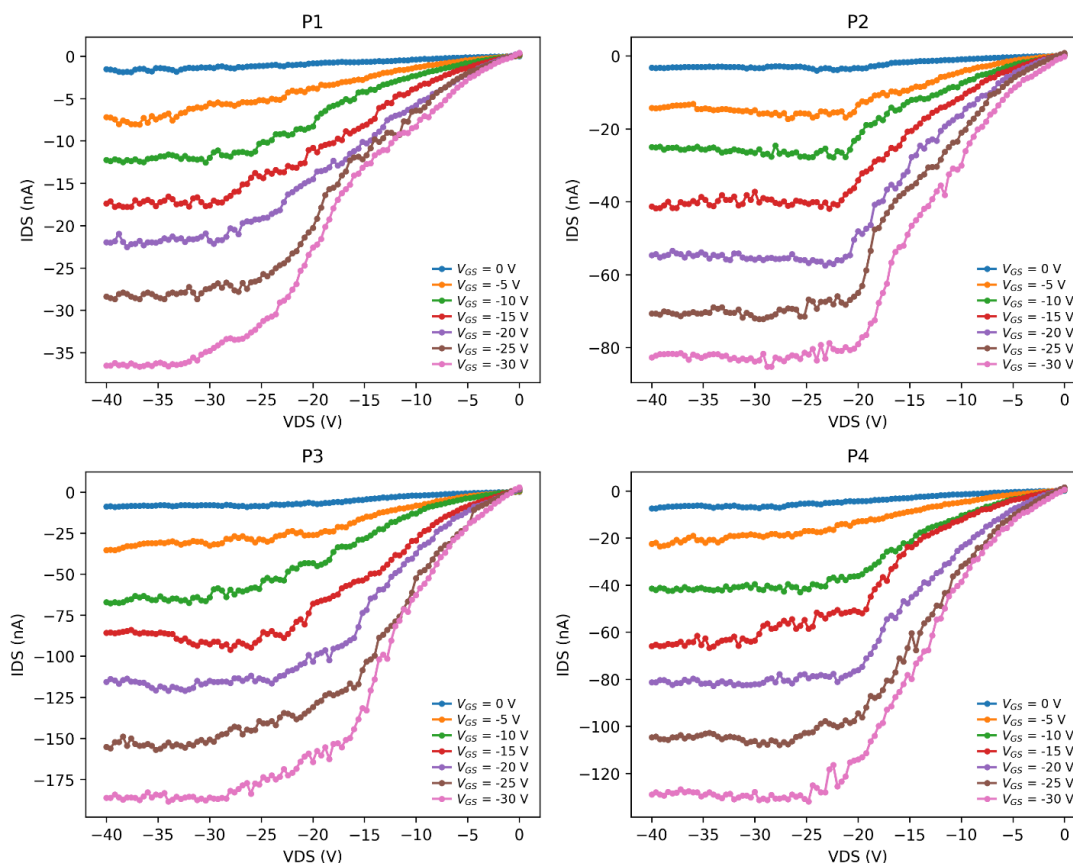
Figure 8. Output characteristics of OFET devices fabricated using Py-1, Py-2, Py-3, and Py-4 as active semiconductor layers. The output curves were recorded in the negative-bias region by sweeping the drain voltage over the negative-bias range while varying the gate bias from 0 to -30 V in 5 V intervals (as labeled in the plotted traces). All devices exhibited p-channel OFET behavior, characterized by a gradual increase in drain-current magnitude as the gate bias became more negative. Distinct differences in output current levels were observed among the pyrene derivatives, following the general order: \text{Py-3} > \text{Py-4} > \text{Py-2} > \text{Py-1} . The enhanced current response of Py-3 is consistent with its more interconnected fibrillar film morphology, whereas the lower responses of Py-1 and Py-4 coincide with comparatively limited domain connectivity and more heterogeneous aggregation, respectively.
