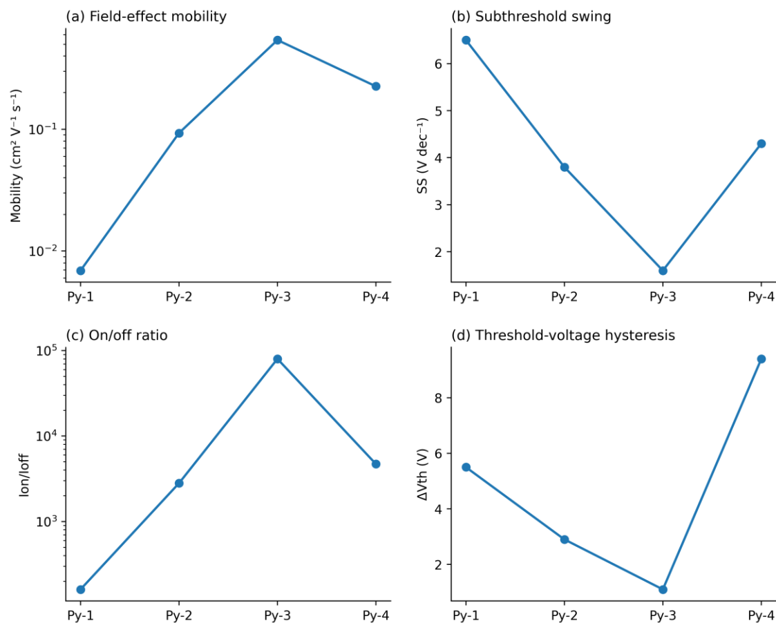
Figure 10. Comparative evolution of the extracted OFET parameters for the Py-1–Py-4 semiconductor series: (a) field-effect mobility ( \mu_{FE} ), (b) subthreshold swing (SS), (c) current on/off ratio ( I_{on}/I_{off} ), and (d) threshold-voltage hysteresis ( \Delta V_{th} ). The parameter evolution illustrates the substituent-dependent variation in charge-transport and switching characteristics across the pyrene derivative series. The values shown correspond to the representative devices discussed in Section 3.9; statistical mean \pm standard deviation values obtained from three independently characterized devices are reported separately in Table 3.4. Panel (a) reflects the corrected W/L = 20 geometry; panels (b–d) retain the reported non-mobility metrics.
