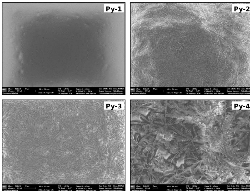
Figure 6. SEM surface morphologies of the synthesized pyrene derivatives: (a) Py-1, (b) Py-2, (c) Py-3, and (d) Py-4. Distinct substituent-dependent morphological evolution was observed across the pyrene-based semiconductor series, ranging from relatively smooth, compact surface organization to interconnected, fibrillar, and aggregated microstructures. The observed evolution demonstrates that molecular substitution strongly influences the mesoscale organization, connectivity, and aggregation characteristics of the semiconductor films.
