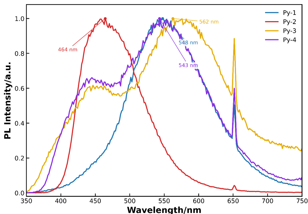
Figure 4. Photoluminescence (PL) spectra of the synthesized pyrene-based semiconducting derivatives (Py-1, Py-2, Py-3, and Py-4) were measured under 325 nm laser excitation. Distinct emission behaviors were observed as a function of the molecular substituent structure, indicating significant variations in intermolecular electronic interactions and excited-state relaxation dynamics. Py-2 exhibited a pronounced blue-shifted emission centered at approximately 464 nm, suggesting relatively reduced intermolecular aggregation and more localized excited-state recombination. In contrast, Py-1, Py-3, and Py-4 displayed broader green-yellow emission bands centered near 548, 562, and 543 nm, respectively, consistent with more pronounced intermolecular excited-state
