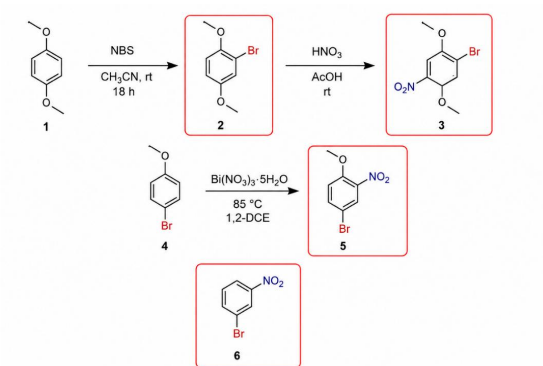
Scheme 1. Synthetic pathway for the preparation of aryl bromide precursor compounds used in the fabrication of pyrene-based semiconductor derivatives. Bromination and nitration reactions were employed to synthesize the intermediate monobromide structures via controlled substitution under varying reaction conditions. The resulting precursor molecules bearing methoxy and nitro functional groups were subsequently used in Suzuki cross-coupling reactions to construct extended pyrene-conjugated semiconductor architectures.
