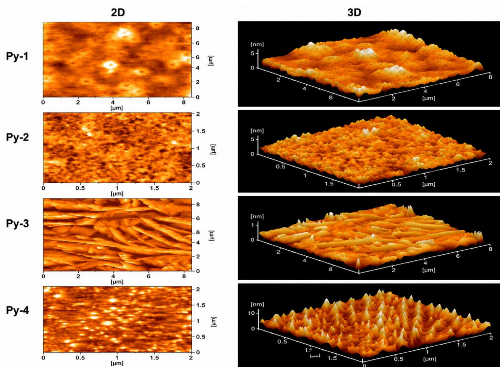
Figure 7. Two-dimensional (2D) and three-dimensional (3D) AFM surface morphologies of the synthesized pyrene-based semiconductor derivatives: Py-1, Py-2, Py-3, and Py-4. The AFM analyses reveal clear substituent-dependent differences in nanoscale surface organization. Py-1 exhibits comparatively homogeneous topography, whereas Py-2 displays interconnected granular domains. Py-3 exhibits pronounced fibrillar features and enhanced lateral connectivity across the film surface. In contrast, Py-4 shows densely distributed aggregated nanodomains and pronounced topographical protrusions, indicating increased morphological heterogeneity. These observations demonstrate that molecular substitution strongly influences nanoscale film organization and surface topology. The AFM results are interpreted as complementary morphological evidence and are not used independently to assign specific \pi - \pi stacking geometries; molecular-scale structural organization is considered separately on the basis of the XRD analysis presented in Section 3.6.
