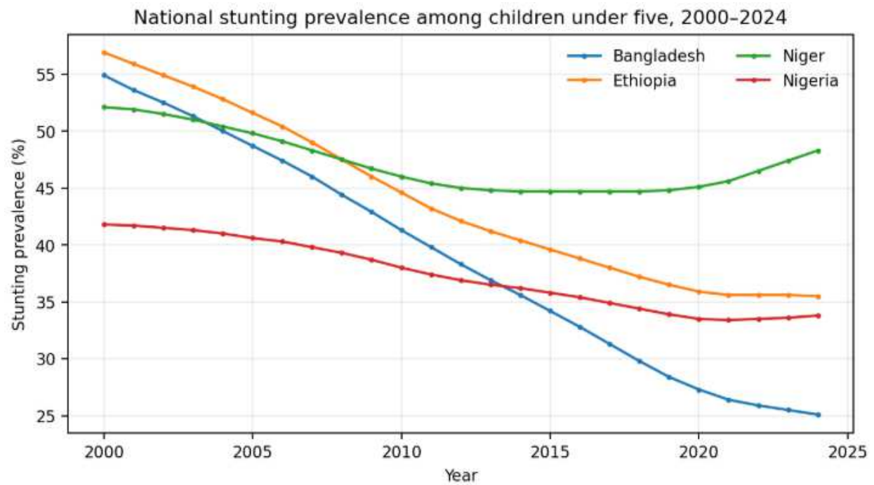
Figure 1. Estimated national stunting prevalence among children under five in Bangladesh, Ethiopia, Niger, and Nigeria, 2000–2024. Lines show annual JME point estimates.
