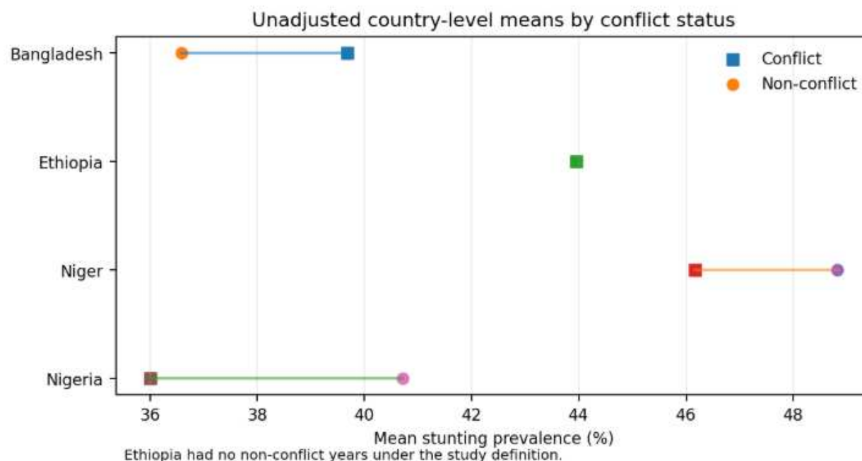
Figure 2. Unadjusted mean stunting prevalence in conflict and non-conflict years by country. Ethiopia has no non-conflict observations under the study definition.
