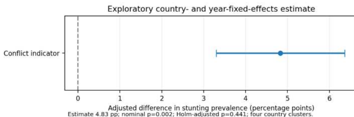
Figure 3. Exploratory fixed-effects estimate for the conflict indicator. Estimate = 4.83 percentage points; p = 0.002 . Only four country clusters were available.
