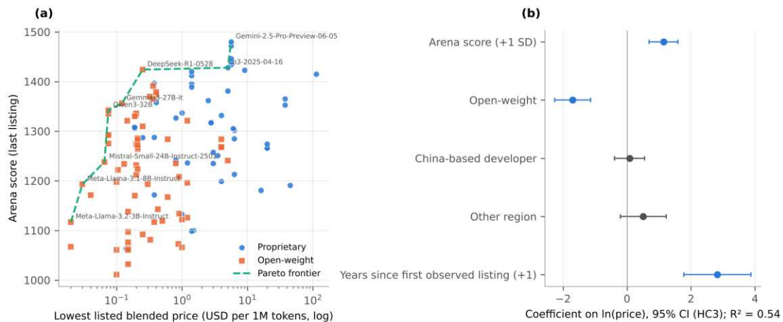
Fig. 10 (a) Arena score at last listing against lowest listed price with the Pareto frontier. (b) Hedonic coefficients with 95% HC3 intervals (grey = not significant)
