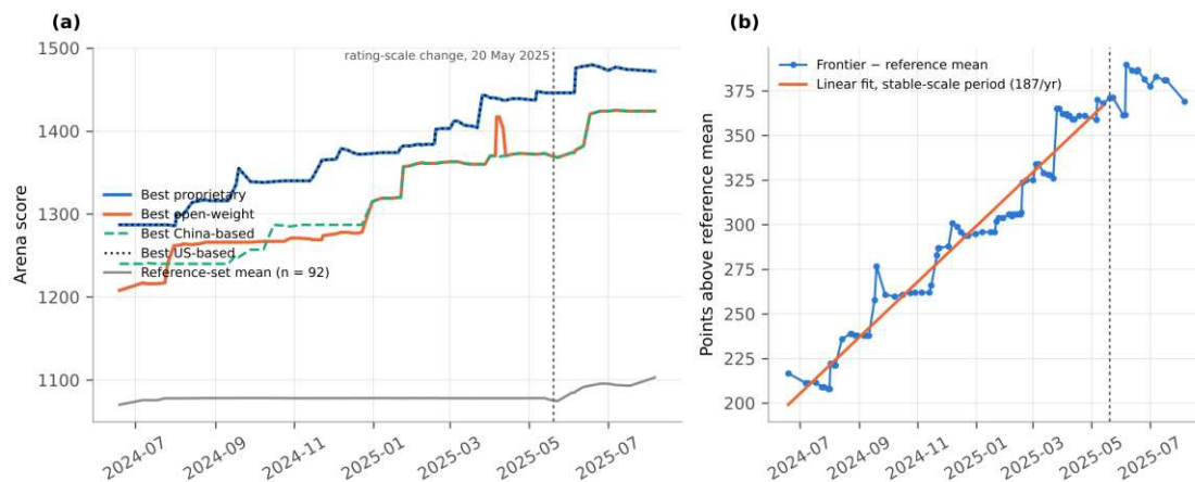
Fig. 5 (a) Best arena score by licensing regime and by developer country over time, with the mean of the 92-model reference set (grey) and the rating-scale change of 20 May 2025 (dotted line); from January 2025 the best open-weight and best China-based lines coincide on all but three snapshot dates. (b) Frontier minus reference mean, with a linear fit over the stable-scale period
