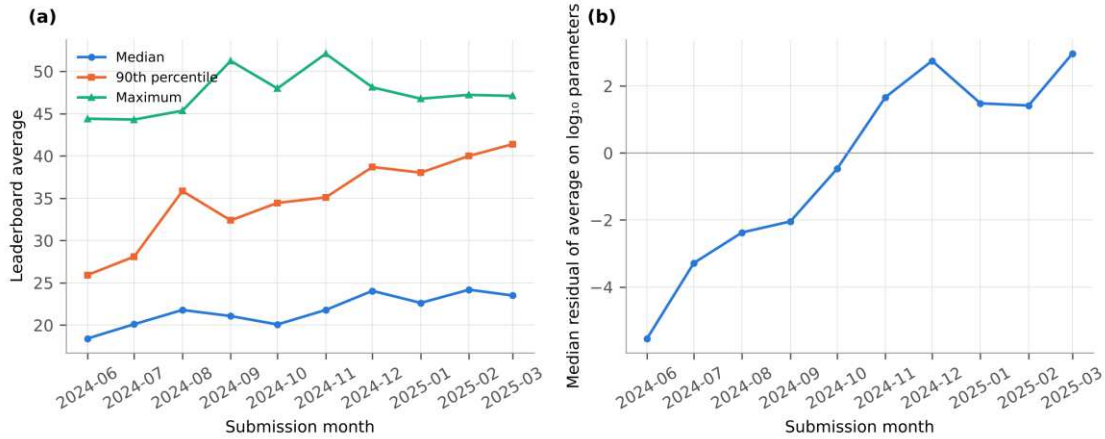
Fig. 4 (a) Median, 90th percentile, and maximum leaderboard average by submission month (months with at least 20 records). (b) Median residual by submission month from an OLS regression of the leaderboard average on \log_{10} parameters over all dated records
