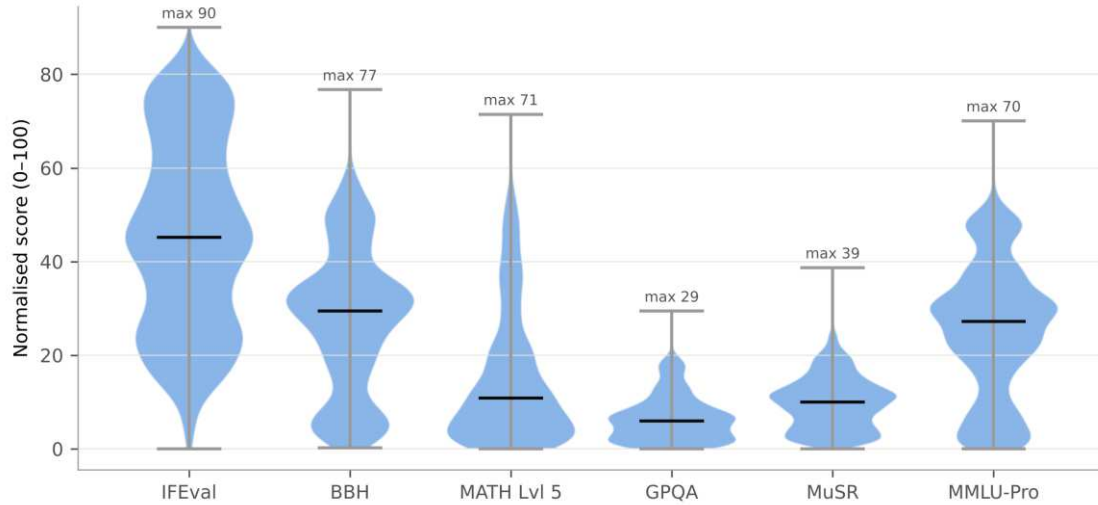
Fig. 1 Score distributions (violin plots with medians) for the six Open LLM Leaderboard v2 benchmarks ( n = 4,565 records)
