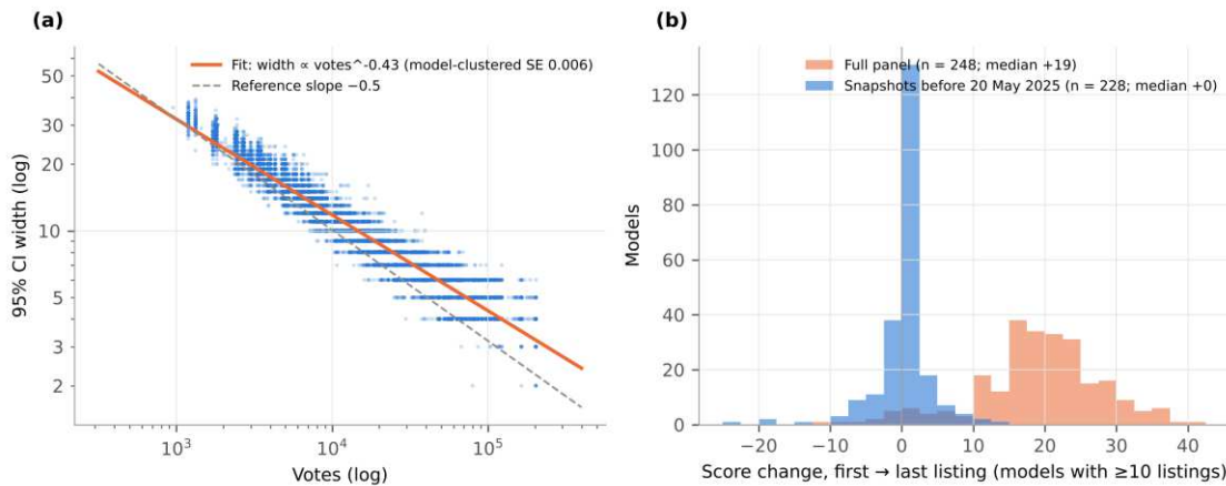
Fig. 7 (a) Confidence-interval width against votes (log–log) with the fitted power law (model-clustered standard error) and the -0.5 reference slope. (b) Score change from first to last listing for models with at least ten listings: full panel versus snapshots before the rating-scale change of 20 May 2025
