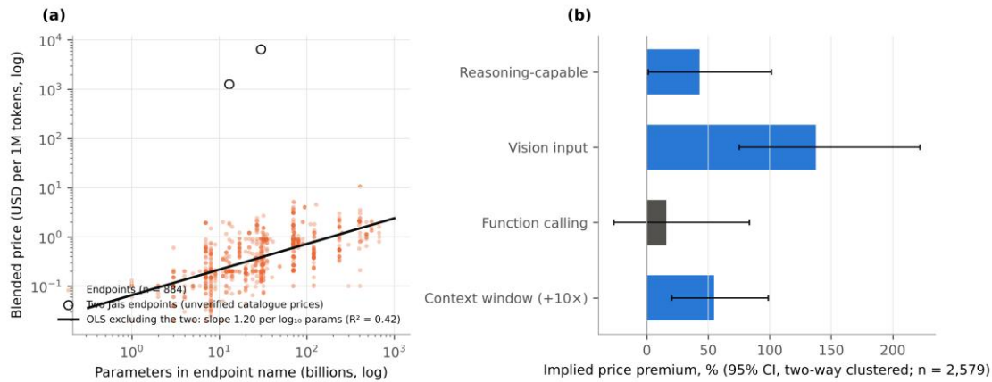
Fig. 8 (a) Blended price against the parameter count disclosed in the endpoint name ( n = 884 ), with the two unverified Jais endpoints marked and the OLS fit excluding them. (b) Implied price premiums for feature flags and context window with 95% intervals from standard errors clustered two-way by model and provider category (grey = not significant at the 5% level)
