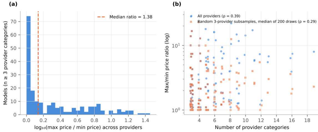
Fig. 9 Cross-provider price dispersion for the 201 models with three or more provider categories. (a) Distribution of the max/min price ratio. (b) Ratio against number of provider categories: all providers (circles) and the per-model median over 200 random three-provider subsamples (squares), with the respective Spearman correlations
