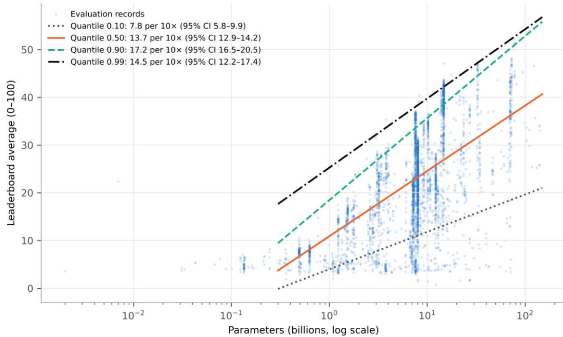
Fig. 3 Leaderboard average against parameter count (log scale) for 4,565 evaluation records, with quantile-regression lines at the 10th, 50th, 90th, and 99th percentiles; intervals are percentile bootstraps with model families resampled (2,000 resamples)
