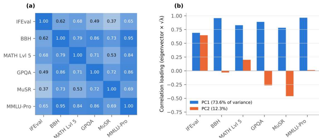
Fig. 2 (a) Spearman correlations among the six benchmark scores. (b) Correlation loadings (eigenvector elements scaled by the square root of the eigenvalue) of the first two components of the Pearson correlation matrix; first-component loadings range from 0.69 (IFEval) to 0.96 (BBH, MMLU-Pro)
