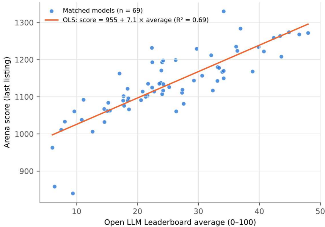
Fig. 11 Arena score at last listing against the Open LLM Leaderboard average for the 69 models present in both sources, with the OLS line; the Spearman correlation reported in the text is a separate rank-based statistic
