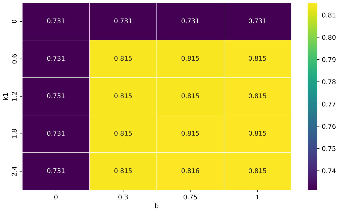
BM25 Mean MRR Surface (Overall)
