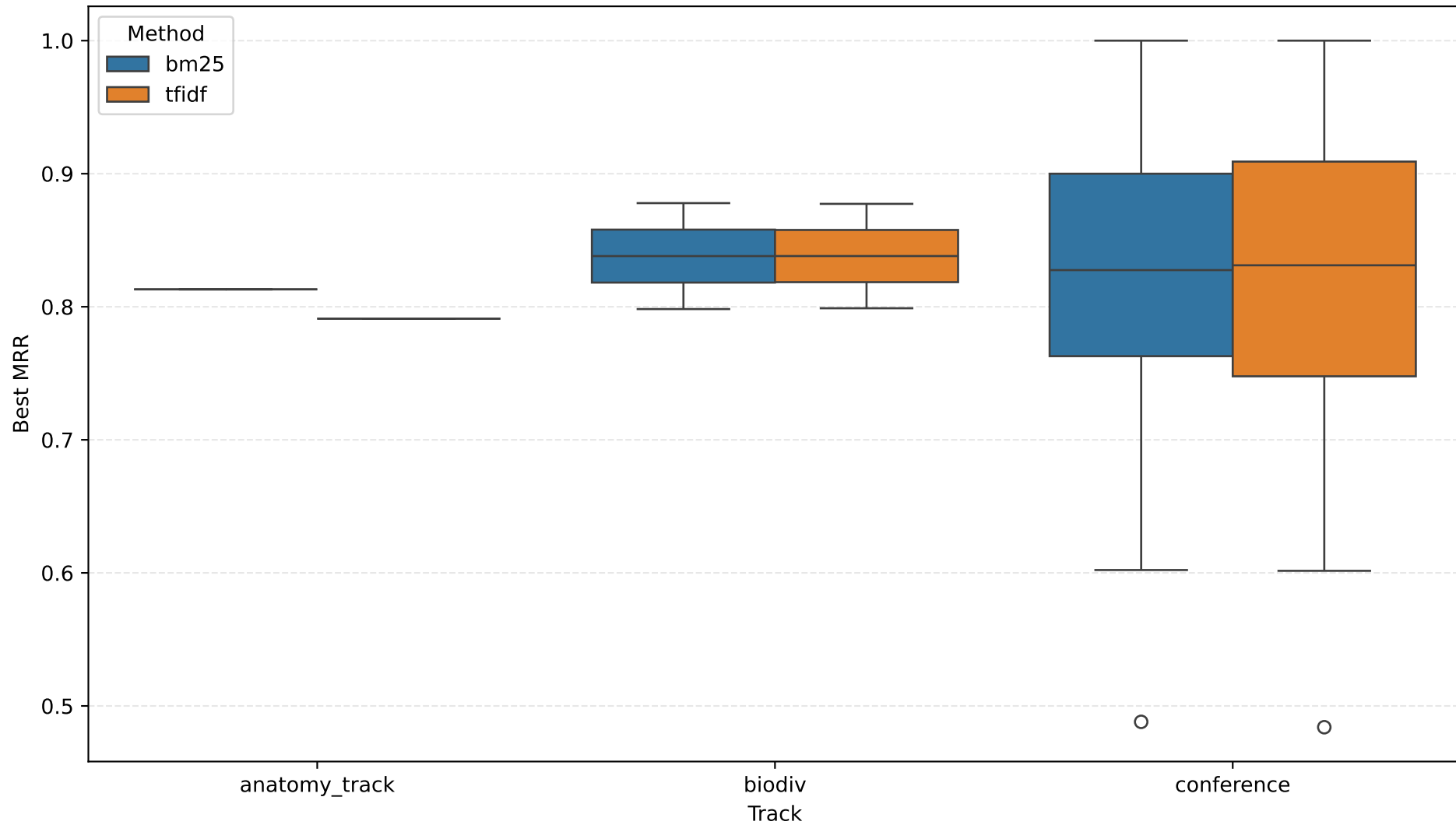
Track-wise Best-of-Grid MRR by Method (Box)
