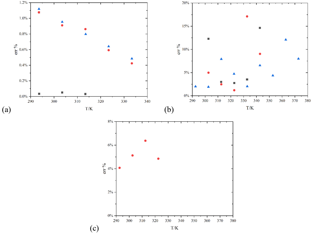
Fig. 1 Relative differences from available literature data: (a) density, 2-HEAA ( \blacktriangle ), HEAPe ( \bullet ), CPAc ( \blacksquare ); (b) viscosity, same symbols; (c) surface tension, HEAPe ( \bullet )
