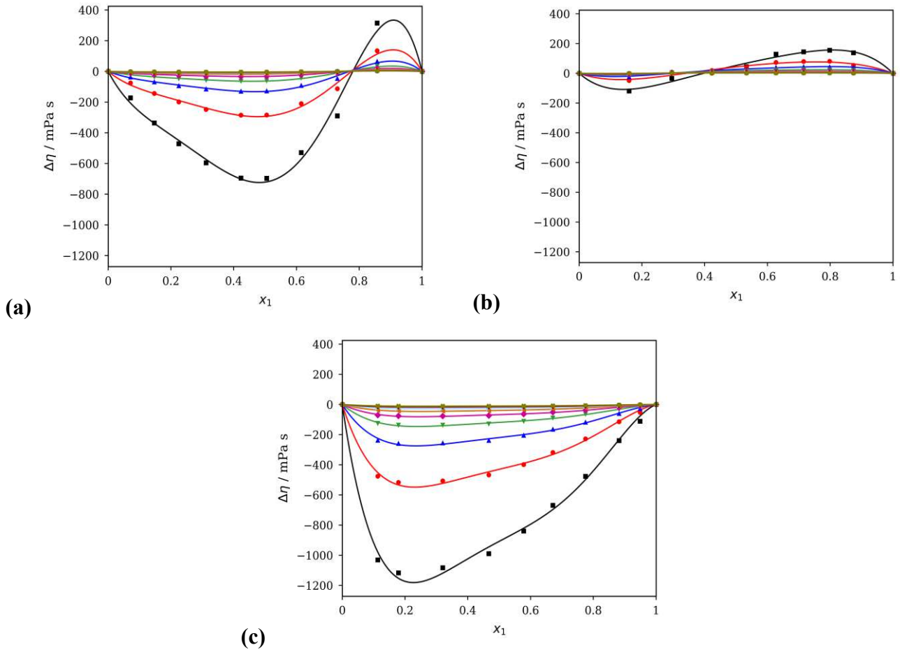
Fig. 5 Influence of temperature on the viscosity deviation of binary mixture: (a) 2-HEAA (1) + CPAc (2); (b) 2-HEAA (1) + HEAPe (2); (c) CPAc (1) + HEAPe (2). Temperatures: (■) 293.15 K, (●) 303.15 K, (▲) 313.15 K, (▼) 323.15 K, (◆) 333.15 K, (◄) 343.15 K, (►) 353.15 K, (○) 363.15 K, and (□) 373.15 K. All lines were obtained by polynomial adjustment of Redlich–Kister equation.
