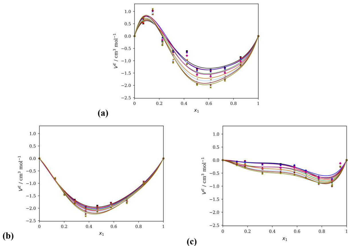
Fig. 3 Influence of temperature on the excess molar volume of binary mixture: (a) 2-HEAA (1) + CPAC (2); (b) 2-HEAA (1) + HEAPe (2); (c) CPAC (1) + HEAPe (2). Temperatures: (■) 293.15 K, (●) 303.15 K, (▲) 313.15 K, (▼) 323.15 K, (◆) 333.15 K,
