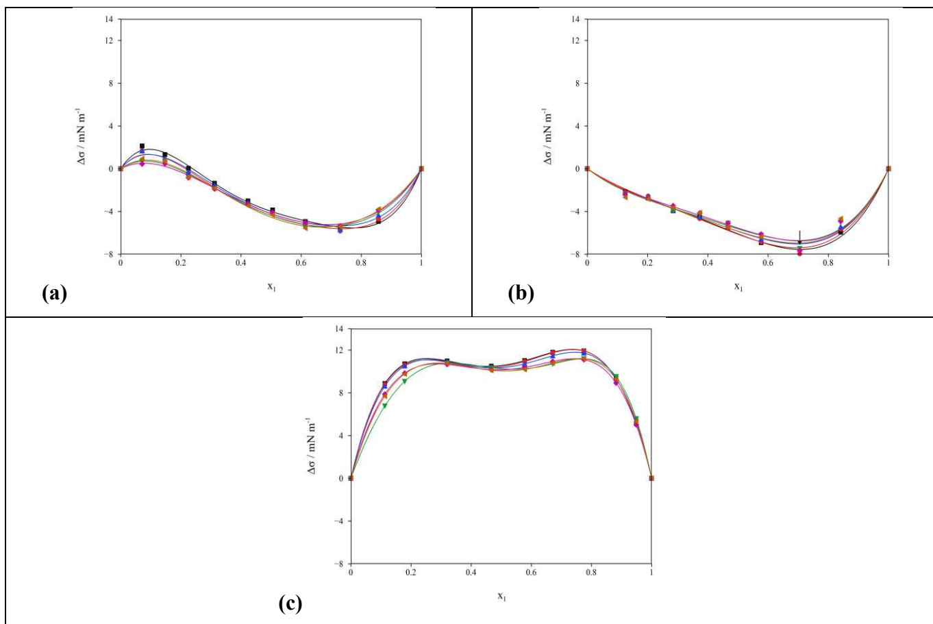
Fig. 7 Surface-tension deviations of (a) 2-HEAA (1) + CPAc (2), (b) 2-HEAA (1) + HEAPe (2), and (c) CPAc (1) + HEAPe (2). Temperatures: (■) 293.15 K, (●) 303.15 K, (▲) 313.15 K, (▼) 323.15 K, (◆) 333.15 K, (◄) 343.15 K. All lines were obtained by polynomial adjustment of Redlich–Kister equation
