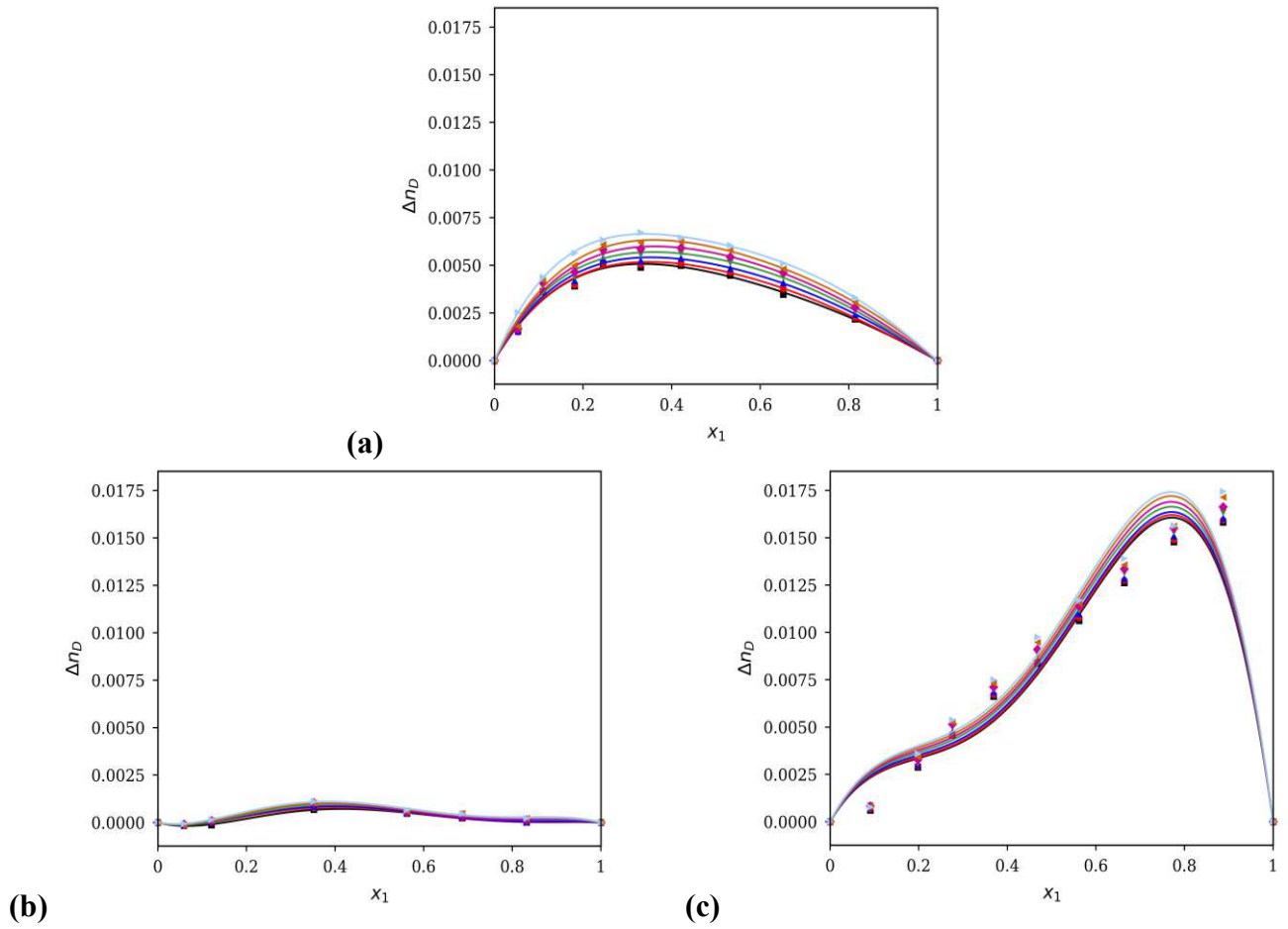
Fig. 8 Influence of temperature on the refractive index deviation of binary mixture: (a) 2-HEAA (1) + CPAc (2); (b) 2-HEAA (1) + HEAPe (2); (c) CPAc (1) + HEAPe (2). Temperatures: (■) 293.15 K, (●) 303.15 K, (▲) 313.15 K, (▼) 323.15 K, (◆) 333.15 K, (◄) 343.15 K, (►) 353.15 K. All lines were obtained from the Redlich-Kister polynomial fit
