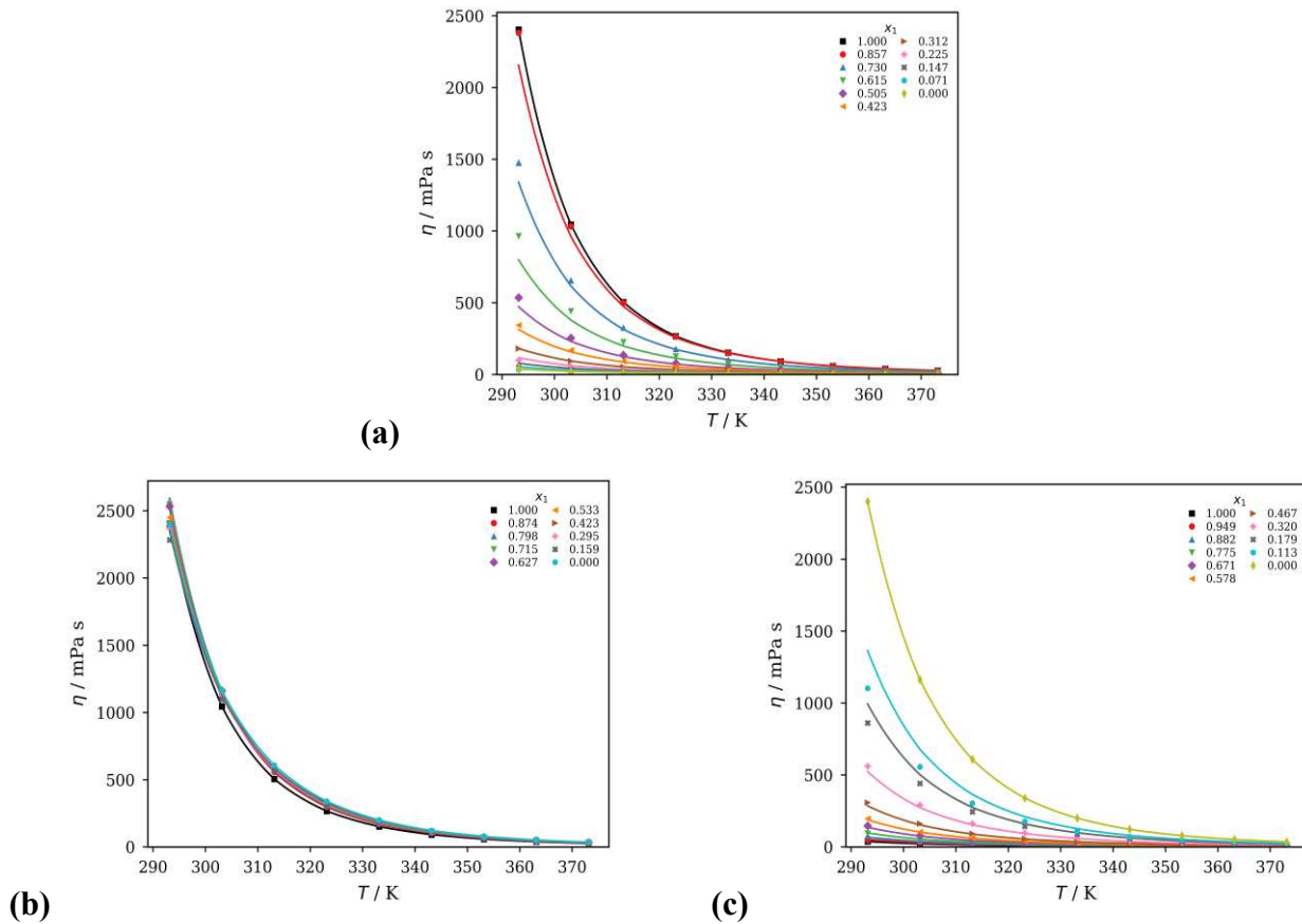
Fig. 6 Measured dynamic viscosities (symbols) and Eyring–NRTL calculated values (lines) for (a) 2-HEAA (1) + CPAc (2), (b) 2-HEAA (1) + HEAPe (2), and (c) CPAc (1) + HEAPe (2). Each panel identifies its measured mole fractions x_1 ; symbols and curves use a matching symbol–curve pair for each composition.
