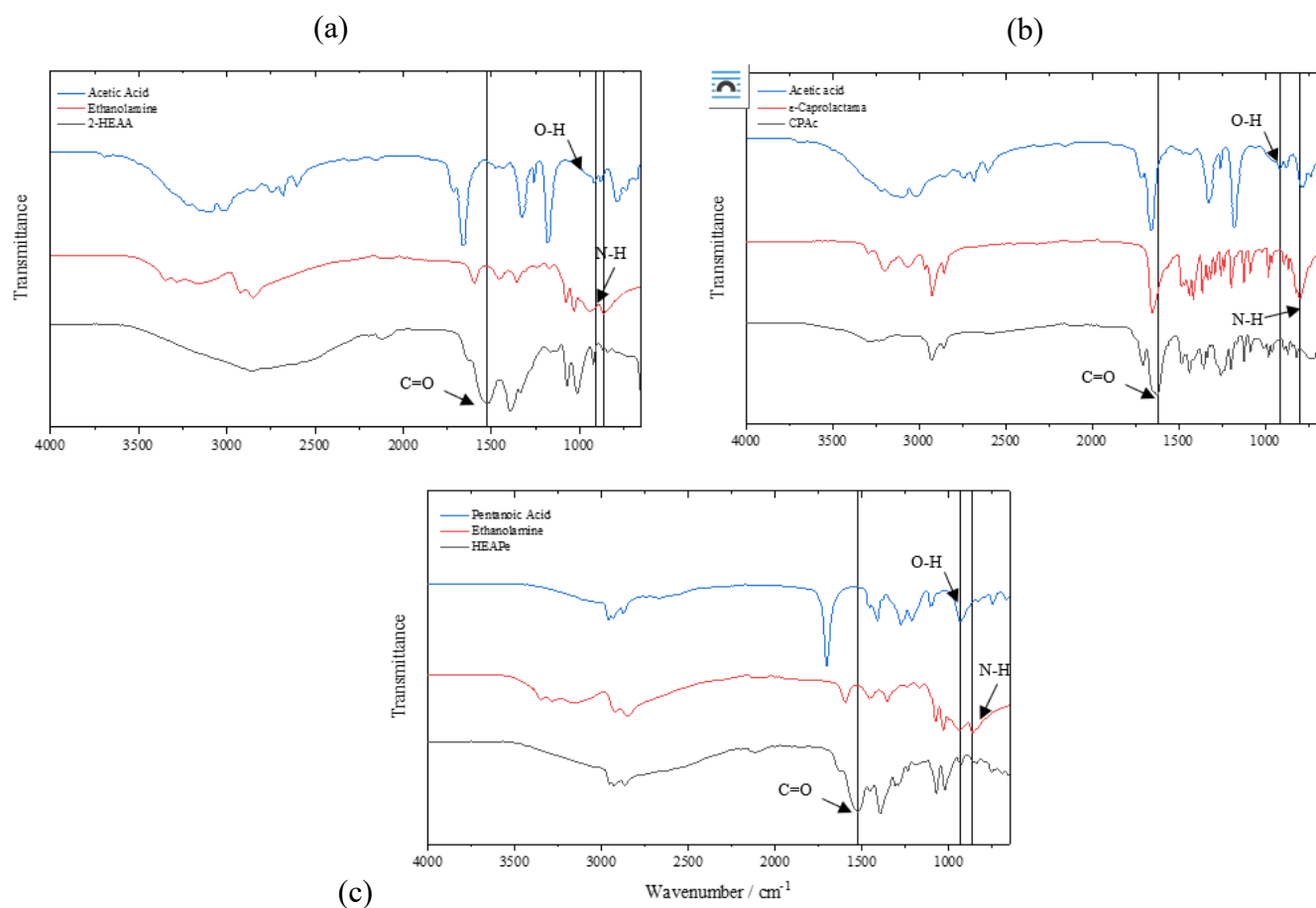
Fig. 2 FTIR transmittance spectra of the reactants and isolated products: (a) acetic acid, ethanolamine, and 2-HEAA; (b) acetic acid, \epsilon -caprolactam, and CPAC; (c) pentanoic acid, ethanolamine, and HEAPe. The arrows near 1524 \text{cm}^{-1} in panels (a) and (c) identify the product carboxylate band region
