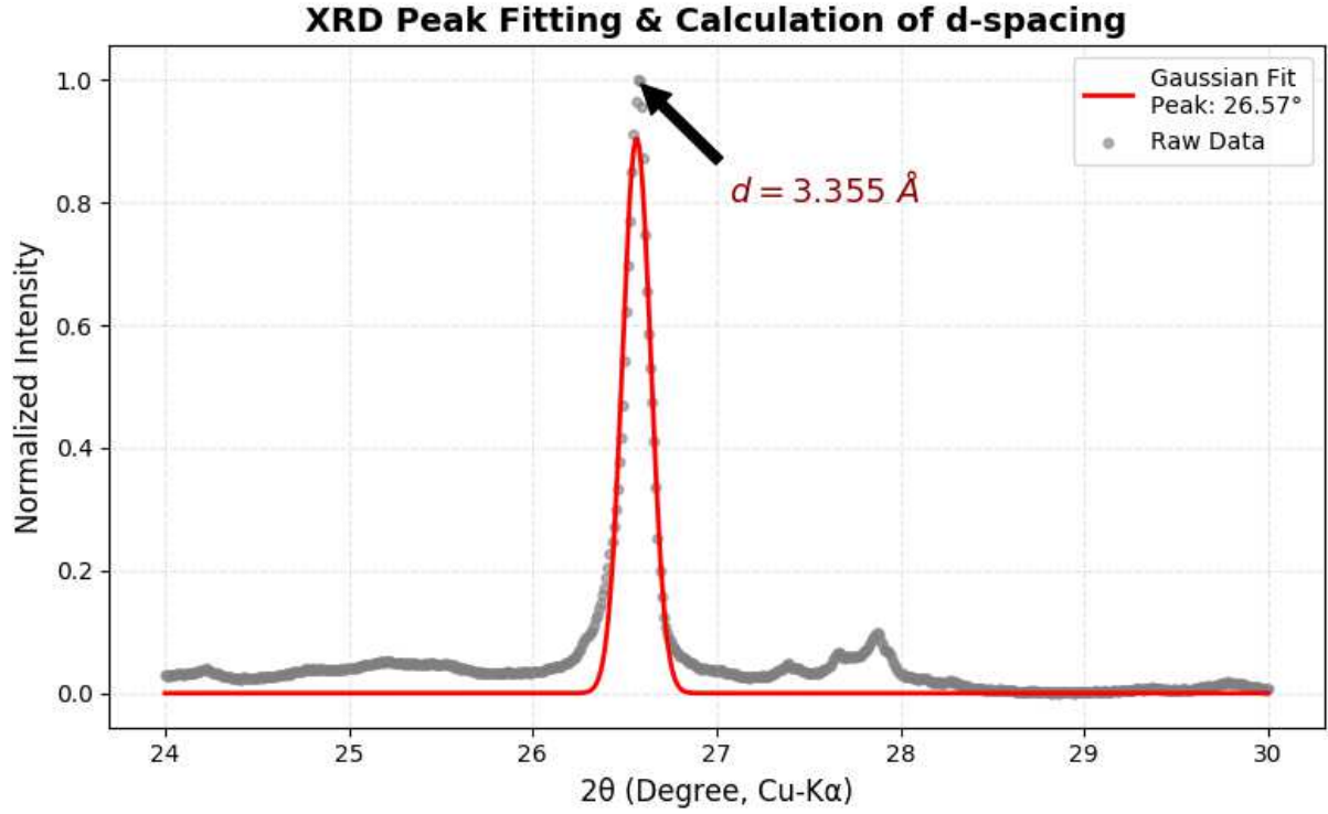
Figure 4: XRD peak fitting of the mechanically milled powder. A Gaussian fit to the sharp reflection at 2\theta = 26.57^\circ yields a calculated interlayer spacing of d = 3.355 \text{ \AA} , indicating turbostratic medium-range-ordered carbon domains.
