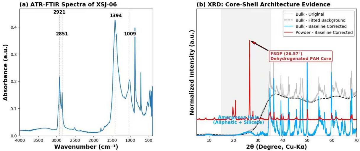
Figure 2: Molecular and structural characterization of the XSJ-06 sample. (a) ATR-FTIR spectrum showing the prominent aliphatic C-H stretching doublet (2921/2851 \text{cm}^{-1} ) and the \text{sp}^2 carbon skeletal ring vibration (1394 \text{cm}^{-1} ). (b) XRD patterns. The unground bulk sample (blue) exhibits a broad amorphous halo indicative of the aliphatic/silicate shell. In contrast, the mechanically milled powder (red) exhibits a sharp FSDP at 2\theta = 26.57^\circ , proving that grinding induces preferred orientation and exposes the highly ordered turbostratic PAH cores.
