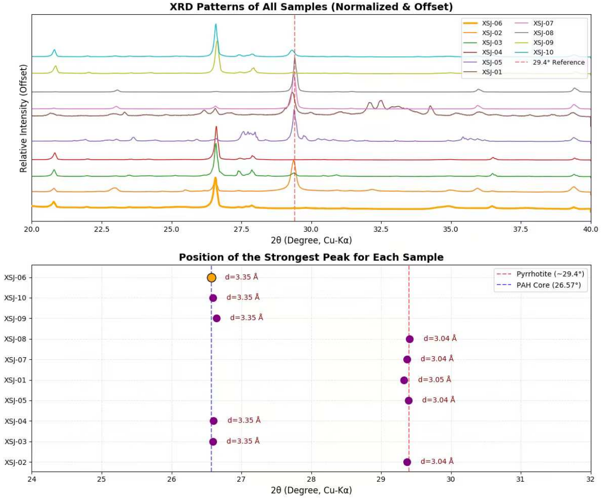
Figure 3: XRD patterns and phase identification. (Top) Normalized and offset XRD patterns for all bulk samples. (Bottom) Position of the strongest peak for each sample, distinguishing between the PAH core ( 2\theta \approx 26.57^\circ ) and nanoscale pyrrhotite/troilite ( 2\theta \approx 29.4^\circ ).
