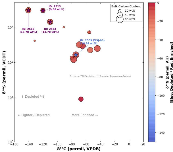
Figure 5: Multi-dimensional isotope correlation of C, N, and S in nebular matrix fractions. Extreme mass-independent sulfur anomalies ( \delta^{34}\text{S} > 3000\text{‰} ) and extreme ^{15}\text{N} depletion confirm the presolar origin of specific microspheres.
