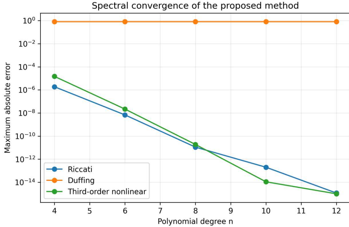
Figure 1. Maximum error versus polynomial degree for the three nonlinear verification problems.
