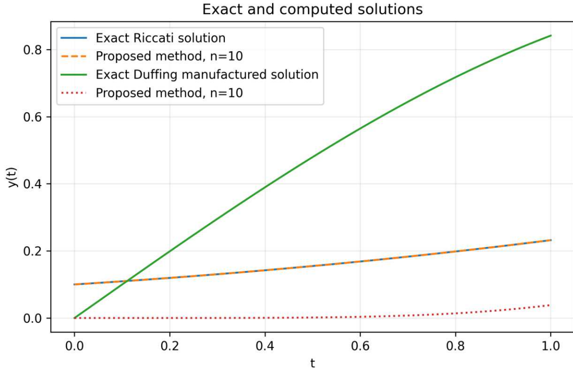
Figure 2. Exact and computed solutions for the Riccati and Duffing-type tests at n=10 .
