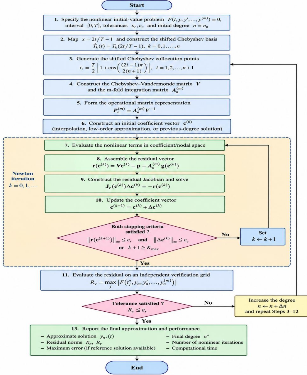
Algorithm 1 summarizes the proposed procedure.
