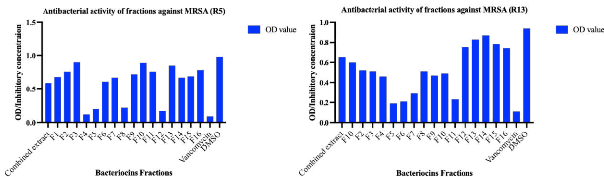
Figure 6. Antibacterial activity analysis of fraction F1-F16 against clinically isolated MRSA R13 and R5.
