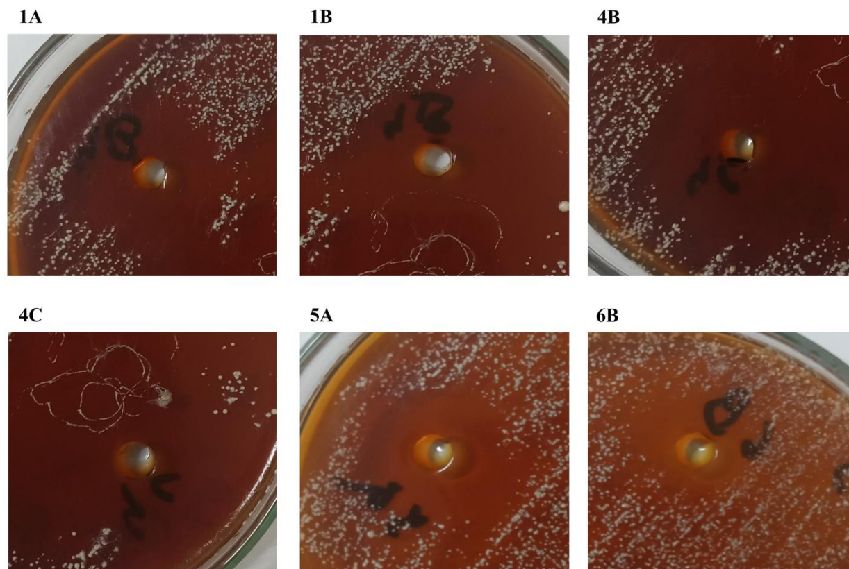
Figure 3. Zones of inhibition of bacteriocin-producing microbiota isolates against MRSA clinical isolates. The cell-free supernatant of bacteriocin-producing human microbiota S. aureus isolates 1A, 1B, 4B, and 4C inhibited the growth of the clinical isolate MRSA-13 and the bacteriocin-producing S. aureus isolates 5A and 6B inhibited the growth of the clinical isolate MRSA-5.
