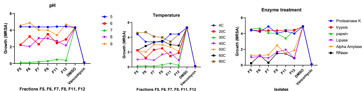
Figure 7. Stability assessment of fractionated bacteriocins to validate their resistance and characterization using pH, temperature, and enzymatic treatments. The bacteriocin extracts were mixed with DMSO (negative control) and vancomycin (positive control) in each assay. The pH stability of bacteriocins at different pH levels ranging from 5 to 9. The temperature steadiness of bacteriocins at different temperature intervals from 4 °C to 80 °C. The effect of treatment with various enzymes on bacteriocins.
