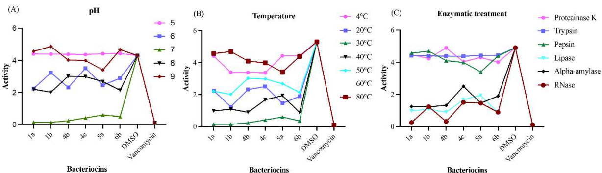
Figure 4. Stability assessment of bacteriocins to validate their resistance and characterization using pH, temperature, and enzymatic treatments. The bacteriocin extracts were mixed with DMSO (negative control) and vancomycin (positive control) in each assay. (A) The pH stability of bacteriocins at different pH levels ranging from 5 to 9. (B) The temperature steadiness of bacteriocins at different temperature intervals from 4 °C to 80 °C. (C) The effect of treatment with various enzymes on bacteriocins.
