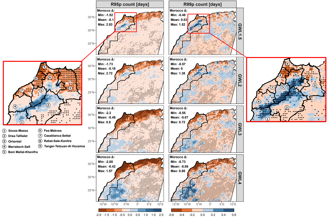
Figure 8: Ensemble-mean change in the annual count of days exceeding the 95th (R95p) and 99th (R99p) wet-day percentiles relative to the 1995–2014 reference period at fixed global warming levels (GWL1.5–GWL4°C). Only members available at each GWL are averaged; scenarios are first averaged within each model to avoid double-counting model effects. Stippling (black dots) marks pixels where all models agree on the sign of change. Annotated statistics are computed over Morocco only. Zoomed insets at GWL1.5°C show the regional detail within Morocco, with numbered labels corresponding to the administrative regions listed in the legend.
