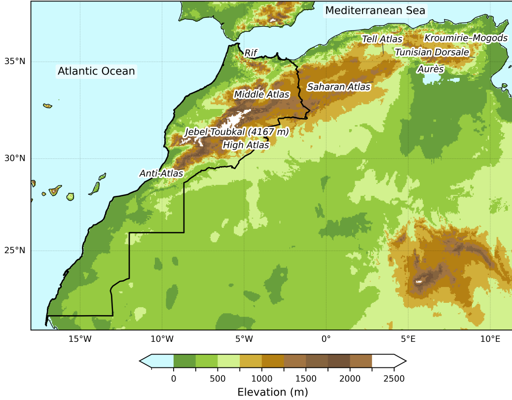
Figure 2: Topography of the study area (Northwest Africa), highlighting Morocco and the Atlas ranges that shape regional climate and elevation gradients.
