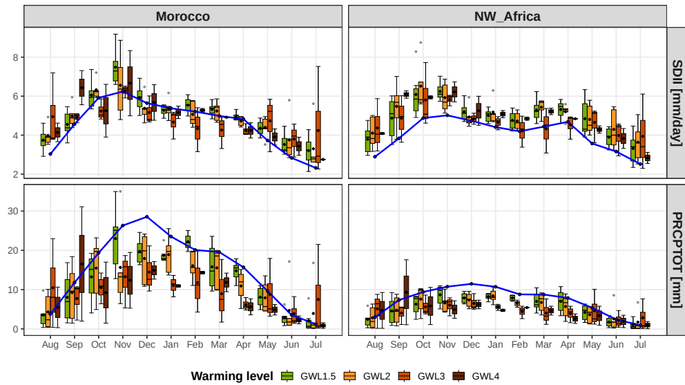
Figure 11: As in Figure 9, but for wet days intensity—SDII and PRCPTOT.
