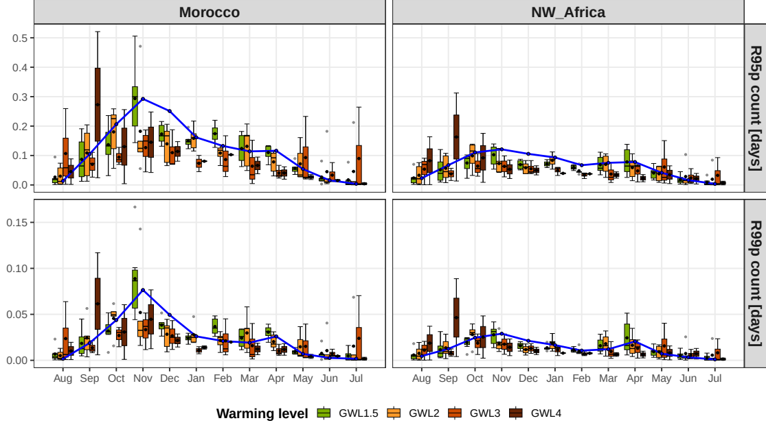
Figure 9: Ensemble spread of the mean seasonal cycle for each downscaled member of the frequency of EP events—R95p and R99p—across Northwest Africa and Morocco at fixed global warming levels (GWLs). The blue line denotes the 1995–2014 reference seasonal cycle (MSWEP); boxes show the interquartile range across members (model–scenario combinations), and black dots indicate the ensemble mean.
