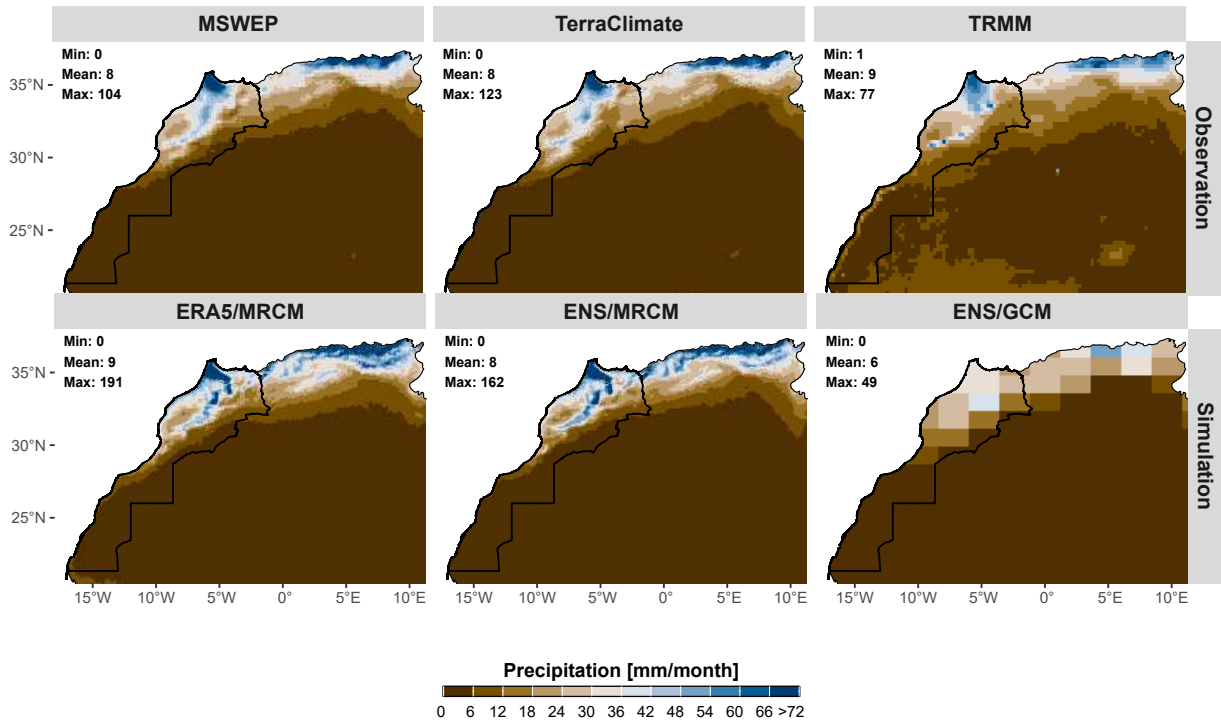
Figure 3: Climatological mean precipitation (1983–2012) across Morocco and Northwest Africa from observation-based datasets (MSWEP, TRMM, TerraClimate), ERA5-forced simulation (ERA5/MRCM), ensemble mean of the 3 GCM-forced simulations (ENS/MRCM), and ensemble mean of 11 GCMs (ENS/GCM).
