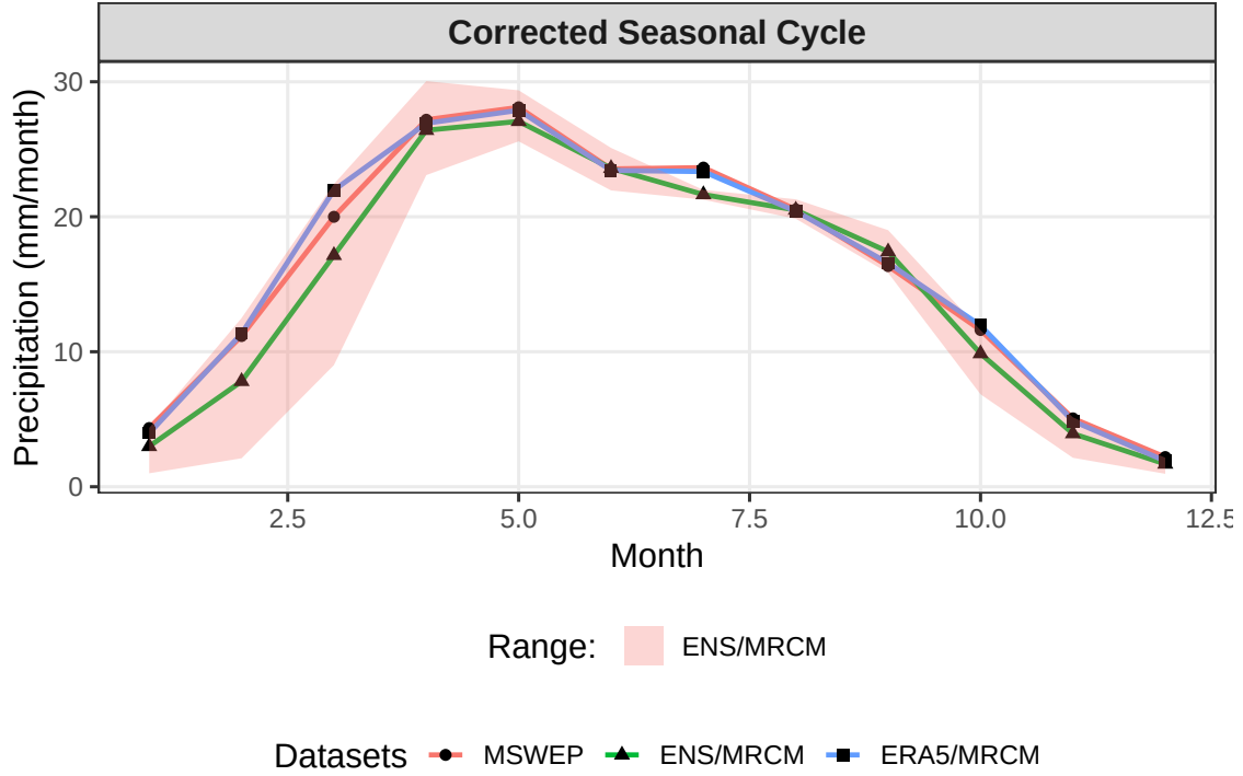
Figure 6: Morocco-mean seasonal cycle (1983–2012) from MSWEP, ERA5/MRCM, and the GCM-forced ensemble mean (ENS/MRCM); model series are shown after EQM correction.
