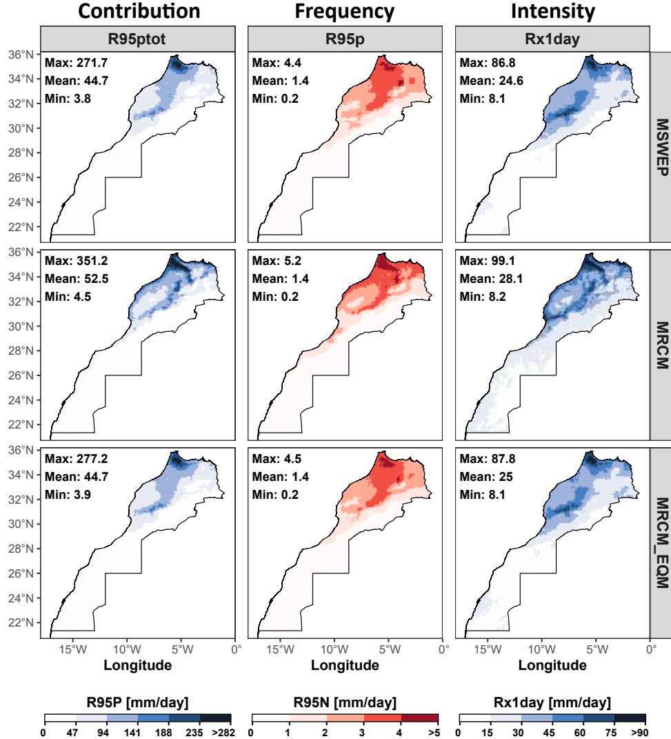
Figure 5: Climatological means of extreme-precipitation indices—R95p, R95pTOT, and Rx1day—computed annually from MSWEP, ERA5/MRCM, and EQM-corrected ERA5/MRCM over the training period (1983–2012).
