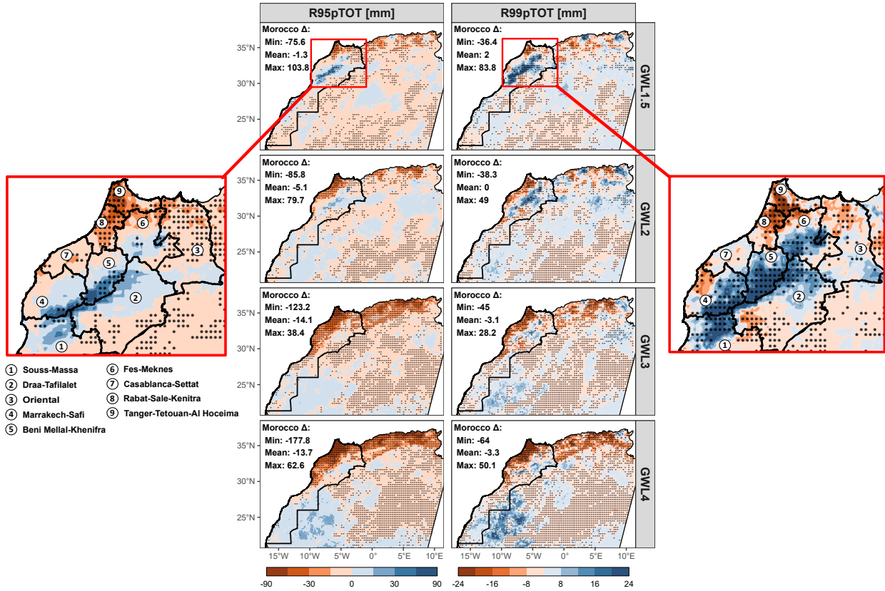
Figure 12: As in Figure 8, but for EP events contribution—R95pTOT and R99pTOT.
