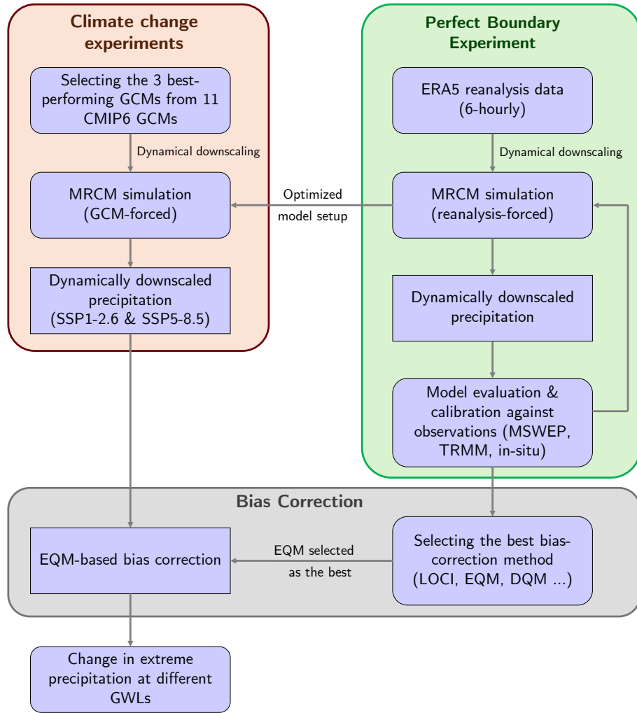
Figure 1: Flowchart of data and methodology
