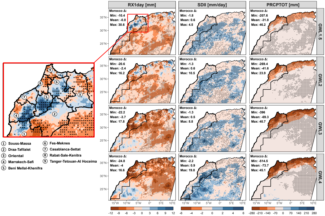
Figure 10: As in Figure 8, but for EP events intensity—SDII, RX1day, and PRCPTOT.
