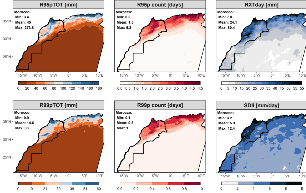
Figure 7: Spatial climatology (1979–2014) of extreme-precipitation indices from MSWEP: intensity/accumulation (RX1day, SDII); frequency (R95p, R99p); and tail contribution (R95pTOT, R99pTOT). Annotated statistics are computed over Morocco only.
