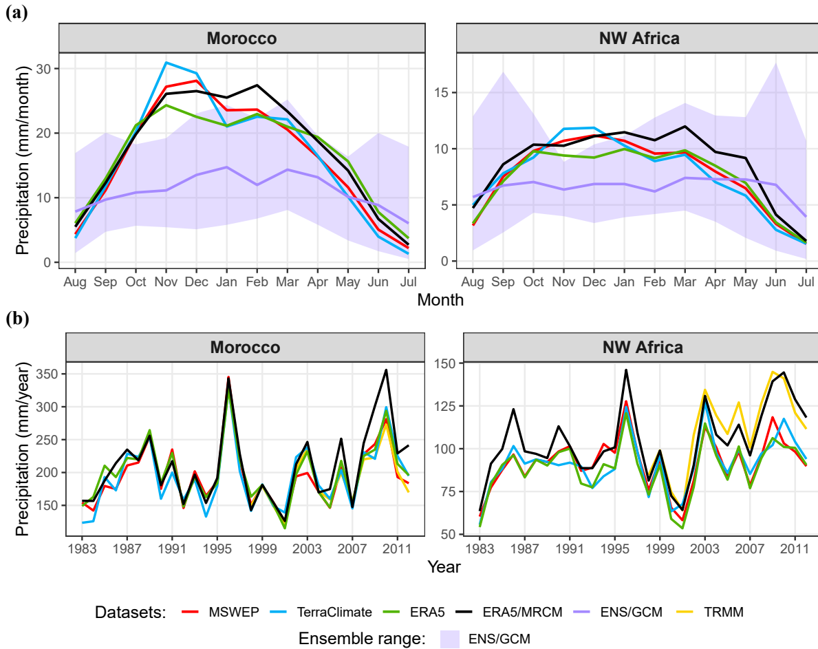
Figure 4: Monthly precipitation climatology (a) and Interannual precipitation totals (b) for the period 1983–2012 and spatially averaged over Morocco and Northwest Africa from observation-based datasets (MSWEP, TRMM, TerraClimate, raw ERA5), ERA5-forced simulation (ERA5/MRCM), and ensemble mean of 11 GCMs (ENS/GCM).
