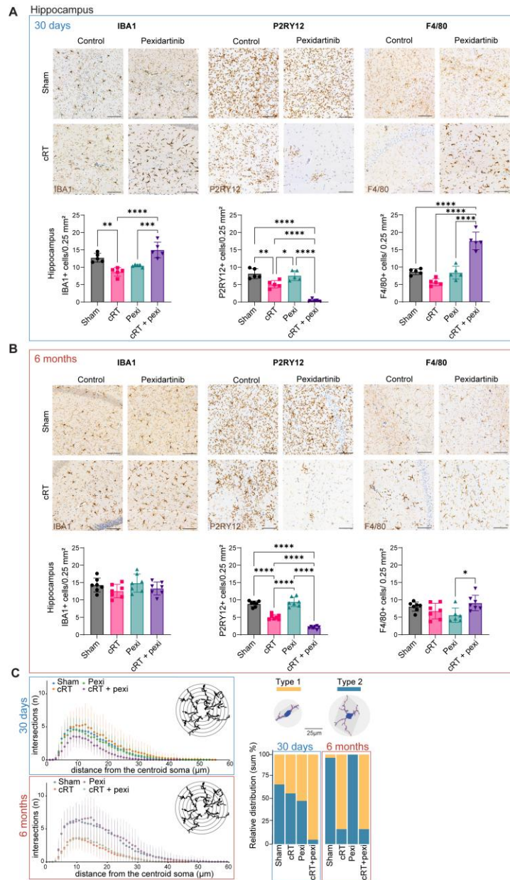
Figure 2. Quantification and morphological assessment IBA1 cells A. IHC of IBA1, P2RY12 and F4/80 in the hippocampus at 30 days post cRT. B. IHC of IBA1, P2RY12 and F4/80 in the hippocampus at 6 months post cRT. Each dot represents one animal, error bars represent standard deviation. * p < 0.05 , ** p < 0.01 , *** p < 0.001 , **** p < 0.0001 . C. Morphometric analysis using mGlia showing a sholl plot and relative cluster distribution plot.
