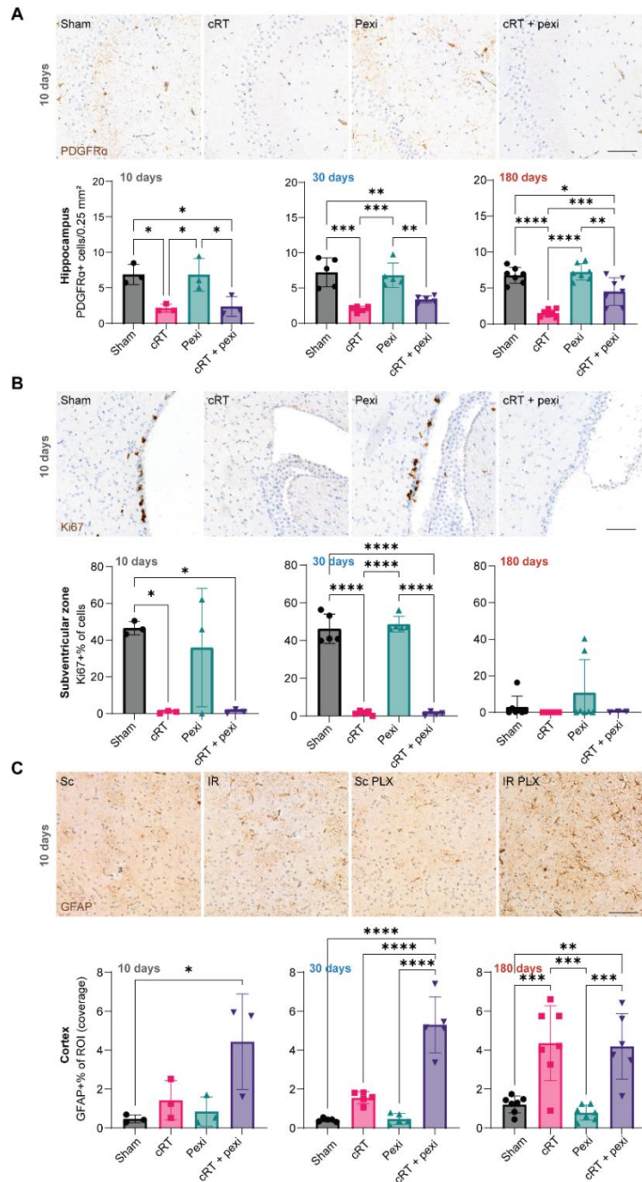
Figure 3. IHC analysis of OPCs, neurogenesis and astrocytes A. IHC of PDGFRα labelling OPCs in the hippocampus at 10 days post cRT and quantification of PDGFRα+ cells on all three time points. B. IHC of Ki67 labelling proliferation in the sub-ventricular zone (neurogenic site) at 10 days post cRT and quantification of Ki67+ cells normalized to total cells on all three time points. C. IHC of GFAP labelling astrocytes in the cortex at 10 days post cRT and quantification of GFAP+ pixel coverage normalized to total region area on all three time points. Each dot represents one animal, error bars represent standard deviation. * p < 0.05 , ** p < 0.01 , *** p < 0.001 , **** p < 0.0001 .
