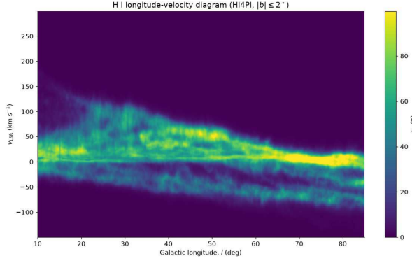
Figure 1: H I longitude-velocity diagram from the supplied HI4PI run, averaged over |b| \leq 2^\circ . The bright emission ridge and
