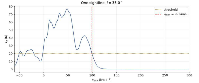
Figure 3: Single-sightline edge measurement at l = 35.0^\circ . The dotted line marks the 20 K threshold and the dashed line marks the
