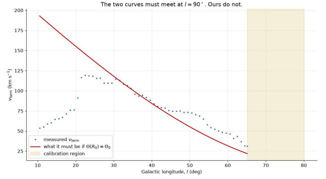
Figure 6: Comparison of measured terminal velocities with the ideal high-longitude behaviour. The shaded calibration region begins
