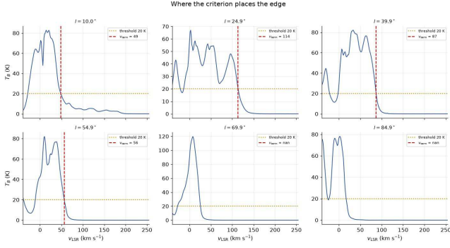
Figure 4: Threshold diagnostic for six representative sightlines. Valid 20 K terminal velocities are found at l = 10.0^\circ , 24.9^\circ , 39.9^\circ and
