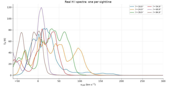
Figure 2: Representative H I spectra for six sightlines from l = 10.0^\circ to 84.9^\circ . Multiple peaks, shoulders and broad wings show why the
