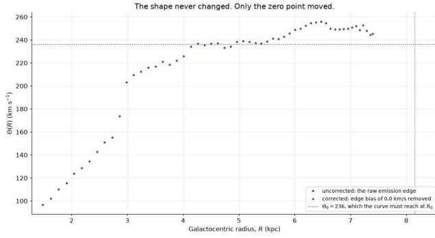
Figure 8: Before-and-after edge-bias diagnostic. The two point sets coincide because the run applied a correction of 0.0 \text{ km s}^{-1} . This
