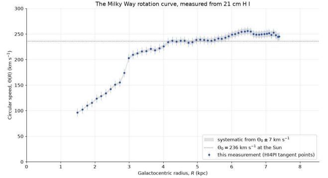
Figure 7: Rotation curve obtained from the accepted tangent-point measurements in the supplied 20 K, |b| \leq 2^\circ run. The curve rises
