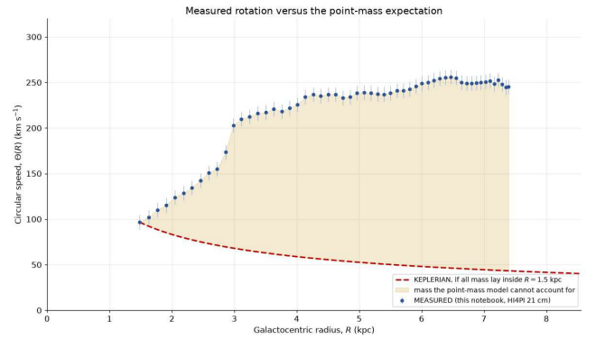
Figure 10: Measured circular speed compared with a Keplerian point-mass expectation anchored at the innermost plotted radius. The
