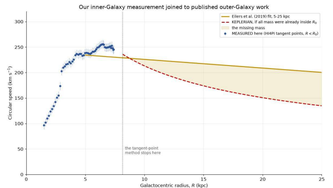
Figure 11: Inner-Galaxy H I result joined to the published Eilers et al. (2019) outer-Galaxy fit. The vertical line marks R_0 and the
