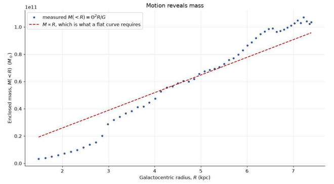
Figure 9: Spherical-equivalent enclosed mass derived from the displayed rotation curve. The inferred mass increases with
