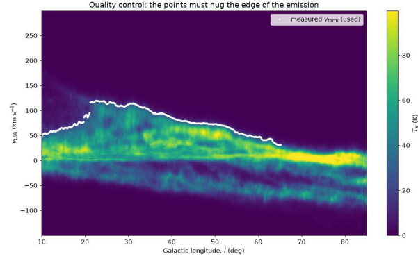
Figure 5: Quality-control overlay of accepted terminal velocities on the l - v diagram. The white trace follows much of the outer
