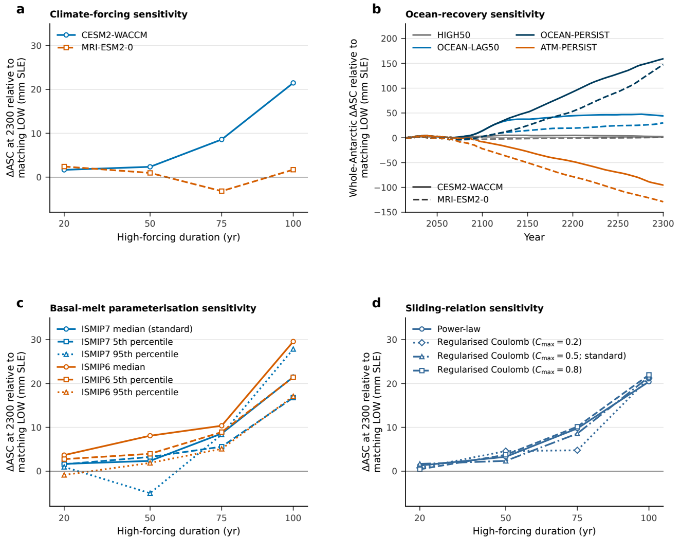
Figure 5. Sensitivity of Antarctic additional sea-level contribution to climate forcing and model configuration. a , Additional Antarctic sea-level contribution ( \Delta\text{ASC} ) at 2300 versus high-forcing duration under CESM2-WACCM and MRI-ESM2-0 climate forcing. b , Time series of whole-Antarctic \Delta\text{ASC} under synchronous atmospheric and ocean recovery (HIGH50), a 50-year delay in ocean recovery (OCEAN-LAG50), persistent high ocean forcing (OCEAN-PERSIST), and persistent high atmospheric forcing (ATM-PERSIST). Colours identify the recovery experiments; solid and dashed lines denote CESM2-WACCM and MRI-ESM2-0 forcing, respectively. c , \Delta\text{ASC} at 2300 versus high-forcing duration across the median, 5th-percentile and 95th-percentile calibrations of the ISMIP7 and ISMIP6 basal-melt parameterisations. The ISMIP7 median calibration is the standard configuration. d , \Delta\text{ASC} at 2300 versus high-forcing duration under the power-law sliding relation and regularised Coulomb relations with C_{\max} = 0.2, 0.5 and 0.8 ; C_{\max} = 0.5 is the standard configuration. All contributions are relative to the corresponding continuously low-forcing simulation and expressed in millimetres of sea-level equivalent (mm SLE). Lines in a , c and d connect discrete experiments as visual guides. These panels share the same y-axis range; b uses a wider range.
