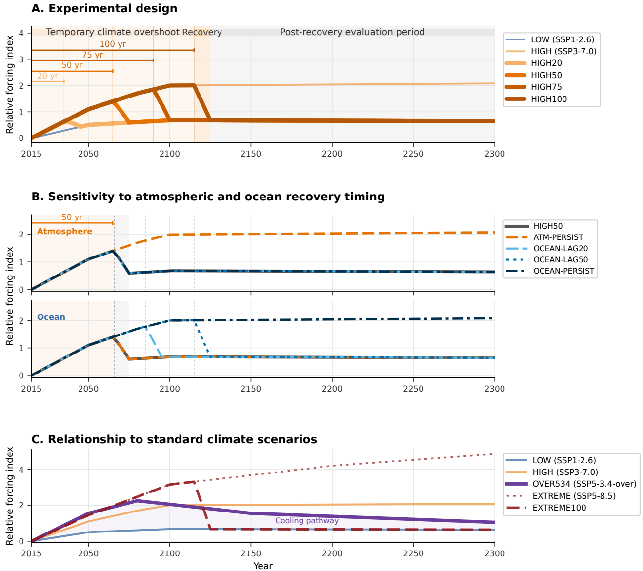
Figure 1. Schematic overview of the climate overshoot experiments. a , Schematic forcing pathways for the controlled climate overshoot experiments. The duration of elevated forcing (20, 50, 75 and 100 years) is systematically varied while maintaining an identical recovery pathway to isolate the effect of forcing duration on Antarctic sea-level contribution (ASC). LOW and HIGH denote the low- and sustained high-forcing reference experiments, respectively. b , Sensitivity experiments that isolate the effects of atmospheric and ocean recovery timing using HIGH50 as the control experiment. Atmospheric and ocean forcing are modified independently while all other aspects of the forcing remain unchanged. c , Relationship between the idealised experiments and the SSP5-3.4-over overshoot pathway (OVER534), together with the sustained high-forcing SSP3-7.0 (HIGH) and SSP5-8.5 (EXTREME) reference scenarios. Curves schematically illustrate the prescribed forcing histories; the experiments use spatially resolved climate fields. The relative forcing index is a schematic representation of the prescribed pathways, not a temperature scale or model output. In particular, the labelled durations indicate years of high forcing before recovery begins, not years above a 1.5 °C global-warming threshold.
