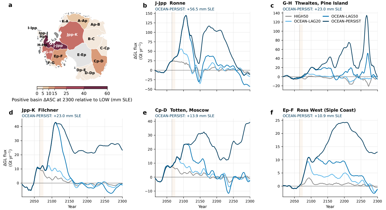
Figure 4. Basin-scale sea-level contribution and grounding-line-flux response to delayed ocean recovery. a , Basin \Delta ASC at 2300 under OCEAN-PERSIST relative to LOW. Warm colours show positive contributions using discrete intervals, and nonpositive values are shown in grey. b–f , Grounding-line-flux diagnostic relative to LOW for the five basins with the largest positive \Delta ASC: b , J–Jpp; c , G–H; d , Jpp–K; e , Cp–D; and f , Ep–F. Curves show centred 11-year running means for HIGH50, OCEAN-LAG20, OCEAN-LAG50 and OCEAN-PERSIST. The vertical dotted line marks the end of the common 50-year high-forcing period in 2065, and shading marks the subsequent 10-year transition. Positive values indicate greater grounding-line flux than under LOW. The grounding-line-flux diagnostic is not a closed basin mass budget.
