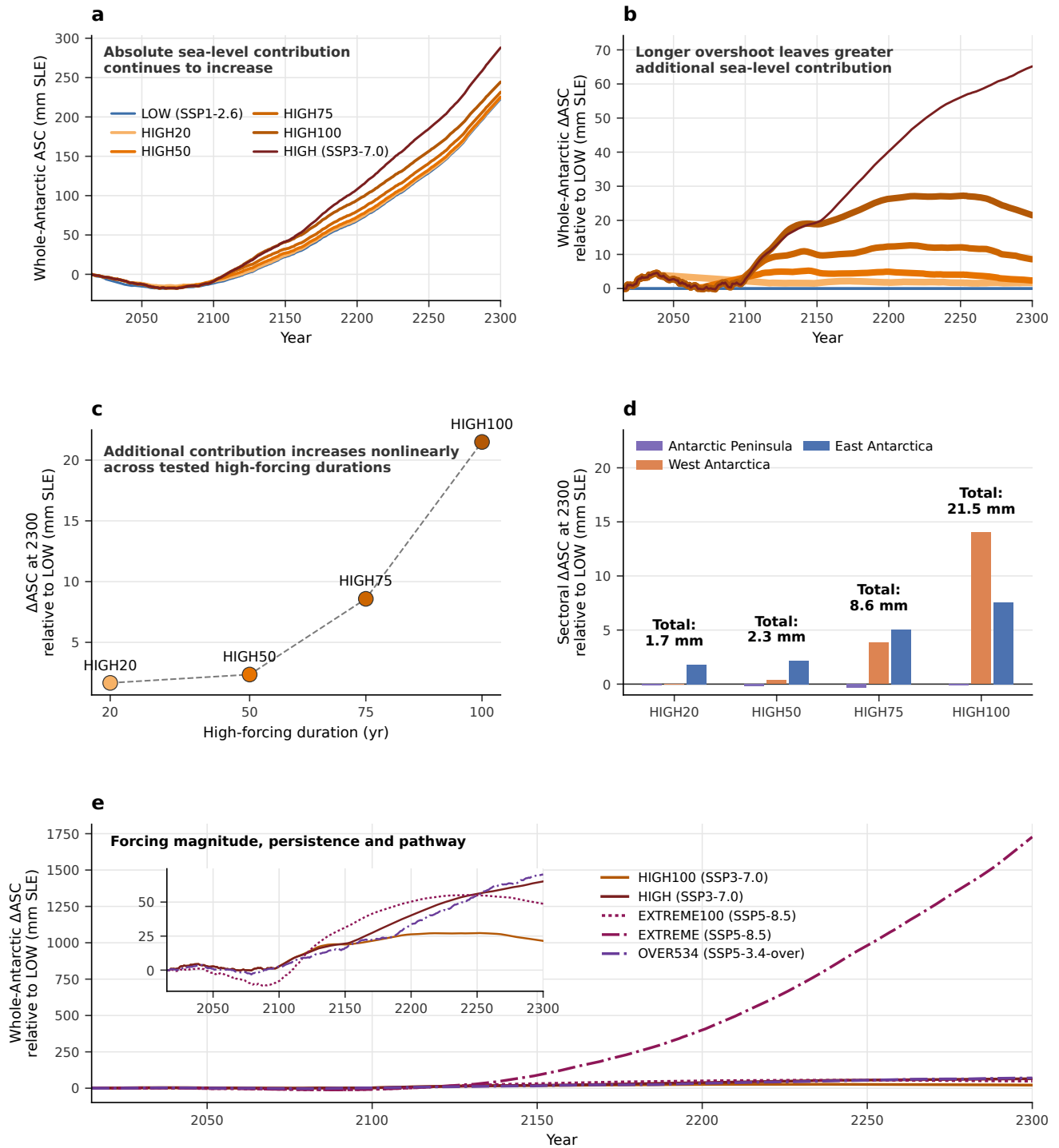
Figure 2. Antarctic sea-level contribution depends on high-forcing duration, magnitude and recovery pathway. a , Time series of cumulative whole-Antarctic sea-level contribution (ASC) under LOW (SSP1-2.6), the four temporary overshoot experiments (HIGH20, HIGH50, HIGH75 and HIGH100), and sustained HIGH (SSP3-7.0). b , Additional Antarctic sea-level contribution relative to LOW ( \Delta ASC) for the same experiments. c , \Delta ASC at 2300 versus high-forcing duration. The dashed line connects discrete experiments as a visual guide. d , Contributions from East Antarctica (EAIS), West Antarctica (WAIS), and the Antarctic Peninsula (AP) to \Delta ASC at 2300. Labels show whole-Antarctic totals. e , \Delta ASC under HIGH100, sustained HIGH, EXTREME100, sustained EXTREME and OVER534. HIGH100 and EXTREME100 apply SSP3-7.0- and SSP5-8.5-derived forcing, respectively, for 100 years before a 10-year transition towards LOW; HIGH and EXTREME maintain their respective forcing pathways through 2300. OVER534 uses SSP5-3.4-over-derived climate forcing. The inset enlarges the four trajectories excluding sustained EXTREME. All sea-level contributions are expressed in millimetres of sea-level equivalent (mm SLE).
