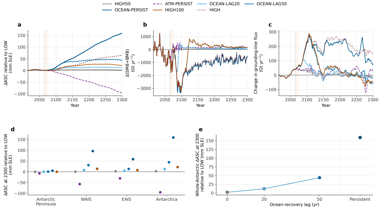
Figure 3. Ocean-forcing persistence and additional Antarctic sea-level contribution. a , Whole-Antarctic sea-level contribution relative to LOW ( \Delta\text{ASC} ) for HIGH50, ATM-PERSIST, OCEAN-LAG20, OCEAN-LAG50, OCEAN-PERSIST, HIGH100 and sustained HIGH. Experiment definitions are given in Table 1. b , Whole-Antarctic anomaly in the sum of surface and basal mass balance (SMB+BMB) relative to LOW. c , Whole-Antarctic anomaly in the area-integrated, model-exported grounding-line flux diagnostic relative to LOW. The diagnostics in b and c provide process context but do not include all terms governing changes in grounded ice above flotation and should not be summed to reconstruct \Delta\text{ASC} . d , \Delta\text{ASC} in 2300 for the Antarctic Peninsula, West Antarctic Ice Sheet (WAIS), East Antarctic Ice Sheet (EAIS) and total Antarctica; sustained HIGH is not shown. e , Whole-Antarctic \Delta\text{ASC} in 2300 by ocean-recovery lag. The line joining the finite-lag experiments (0, 20 and 50 years) is a visual guide; persistent ocean forcing is shown as a separate categorical endpoint. In the time-series panels, the vertical dotted line marks the start of recovery in HIGH50 in 2065, and shading marks its 10-year recovery period. Sea-level contributions are in mm sea-level equivalent (SLE), and fluxes are in \text{Gt yr}^{-1} .
