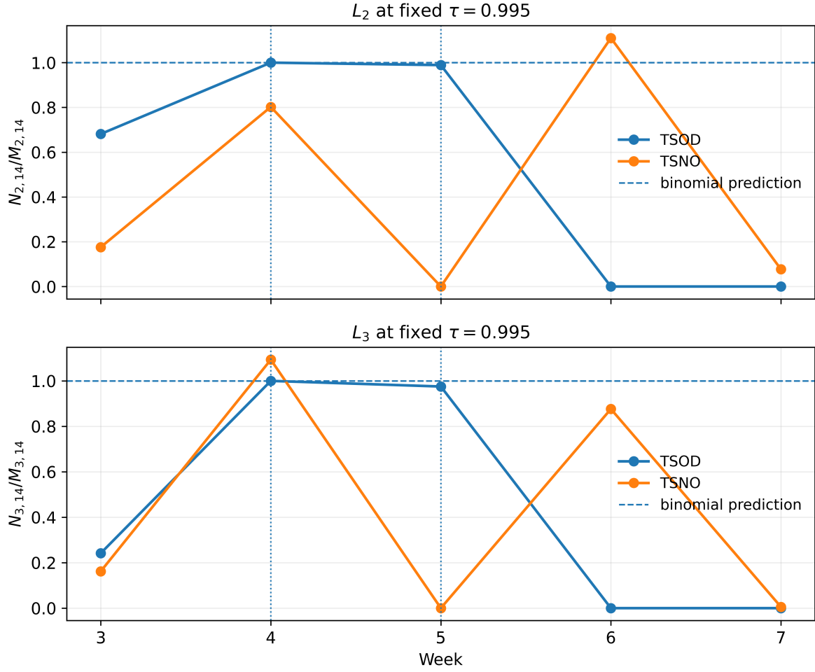
Fixed- q spectral fingerprint across TSOD/TSNO and weeks 3--7
