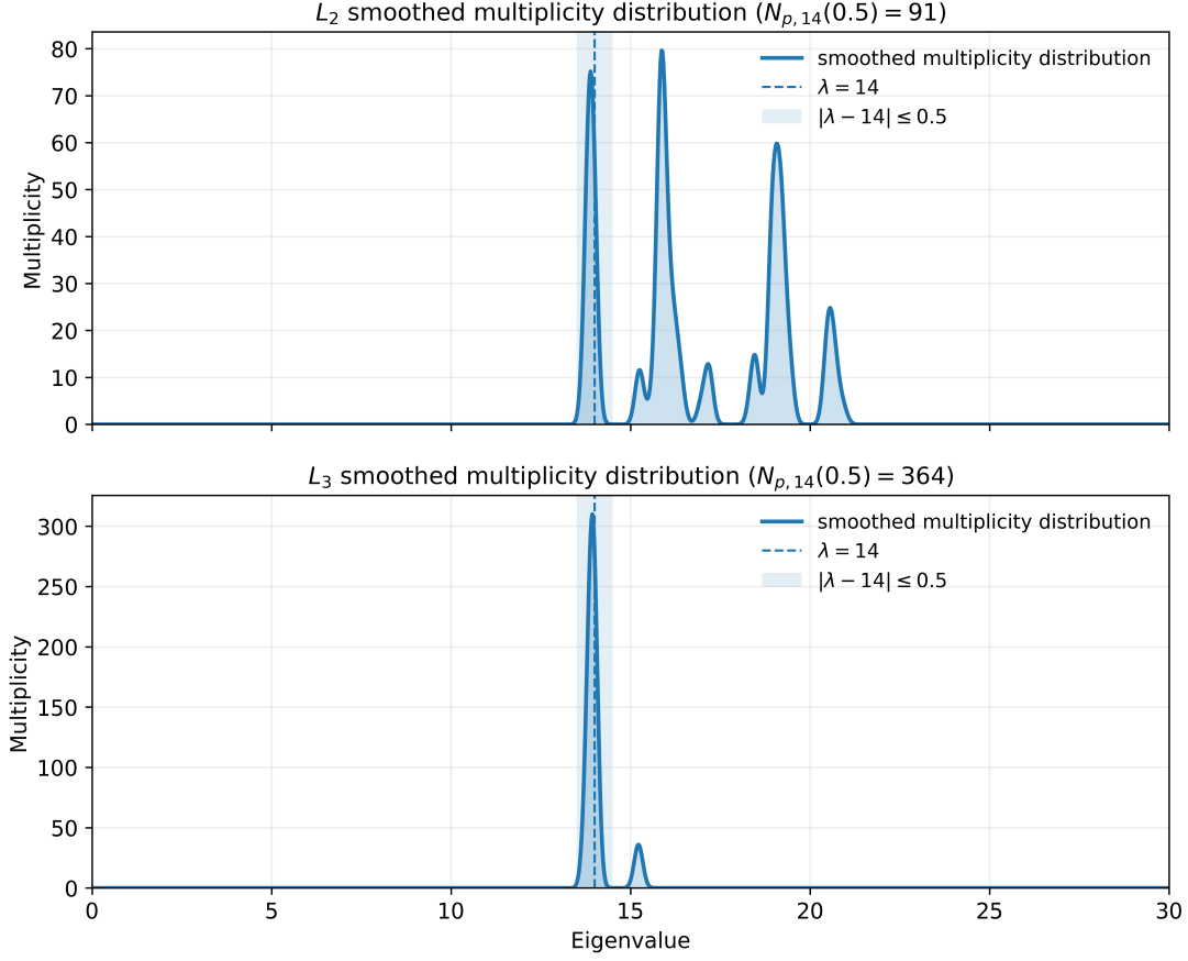
FIG. 4. Smoothed spectral multiplicity distributions of the second- and third-order Hodge Laplacians for TSOD mice at week 4. The dashed vertical line indicates the characteristic spectral scale \lambda = 14 , and the shaded region denotes the interval |\lambda - 14| \leq 0.5 used to evaluate the near-14 multiplicity. For L_2 , the interval contains N_{2,14}(0.5) = 91 eigenvalues, matching the theoretical binomial prediction M_{2,14} = \binom{14}{2} = 91 . For L_3 , the corresponding multiplicity is N_{3,14}(0.5) = 364 , matching M_{3,14} = \binom{14}{3} = 364 . Thus, both Hodge orders exhibit a spectral concentration around the same characteristic scale q = 14 with multiplicities consistent with the predicted cross-order binomial spectral fingerprint.
