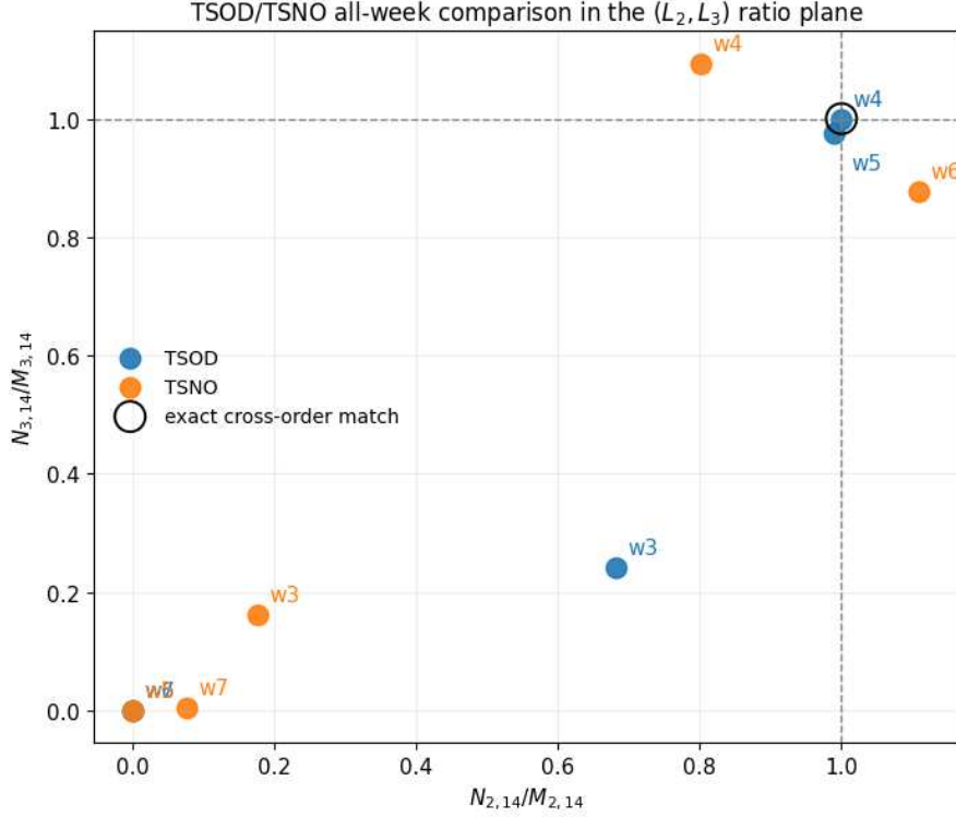
FIG. 6. Cross-order consistency of the q = 14 binomial spectral fingerprint across TSOD and TSNO mice. Each point represents one strain–week condition in the plane defined by R_2 = N_{2,14}/M_{2,14} and R_3 = N_{3,14}/M_{3,14} . The point (1, 1) represents simultaneous agreement with the theoretical multiplicities at both Hodge orders. TSOD week 4 lies exactly at (1, 1) , whereas TSOD week 5 remains close to this point. TSNO conditions deviate from the theoretical point in at least one Hodge order.
