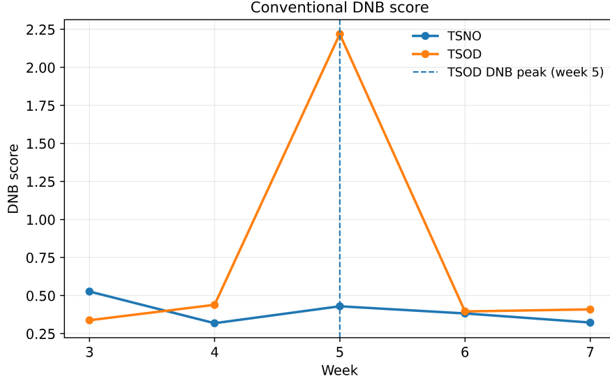
FIG. 3. Conventional DNB score from week 3 to week 7 in TSOD and TSNO mice. The DNB score was evaluated using the fixed 147-gene DNB region previously identified by Koizumi et al. [21]. A pronounced peak is observed at week 5 in the TSOD group, whereas the score remains substantially lower at week 4.
