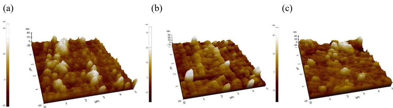
Fig. 6. AFM images of (a) membrane optode without DES, (b) blank membrane optode with DES and (c) DES membrane optode loaded with 2.5 \mu\text{g/mL} Ni(II) solution.
