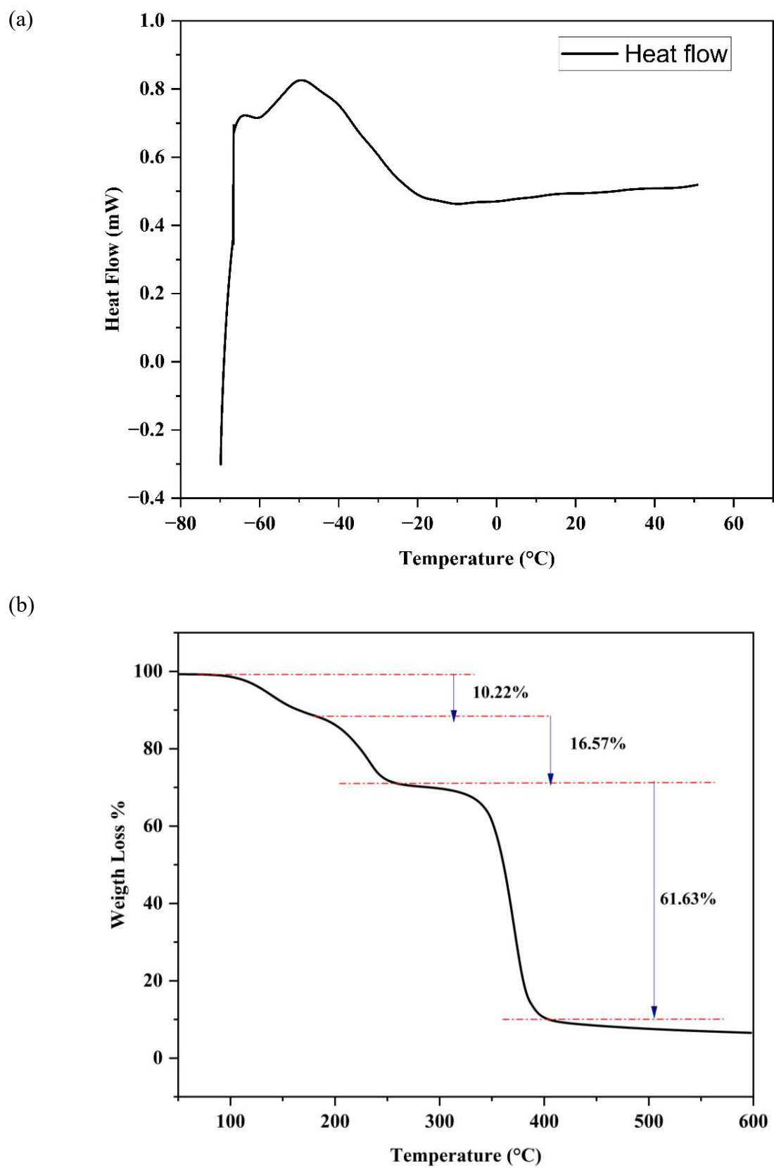
Fig. 5. (a) DSC thermogram of blank membrane optode, (b) TGA thermogram of blank membrane optode
