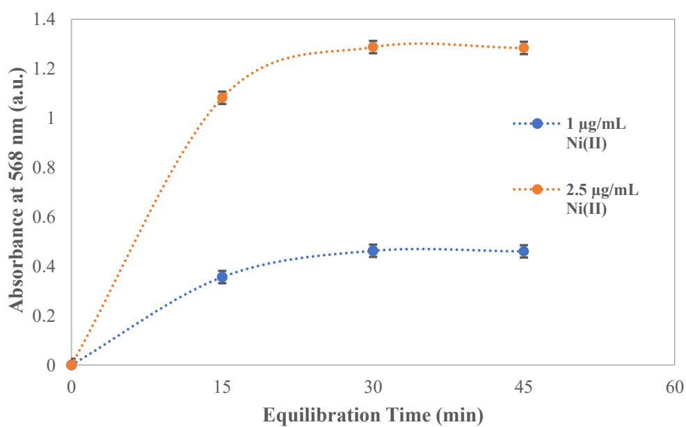
Fig. 2. (a) Effect of pH on the absorbance of the optode equilibrated with 2.5 \mu\text{g/mL} Ni(II), (b) absorbance of the membrane at 568 nm as a function of equilibration time with 1 and 2.5 \mu\text{g/mL} Ni(II) at pH 6.
