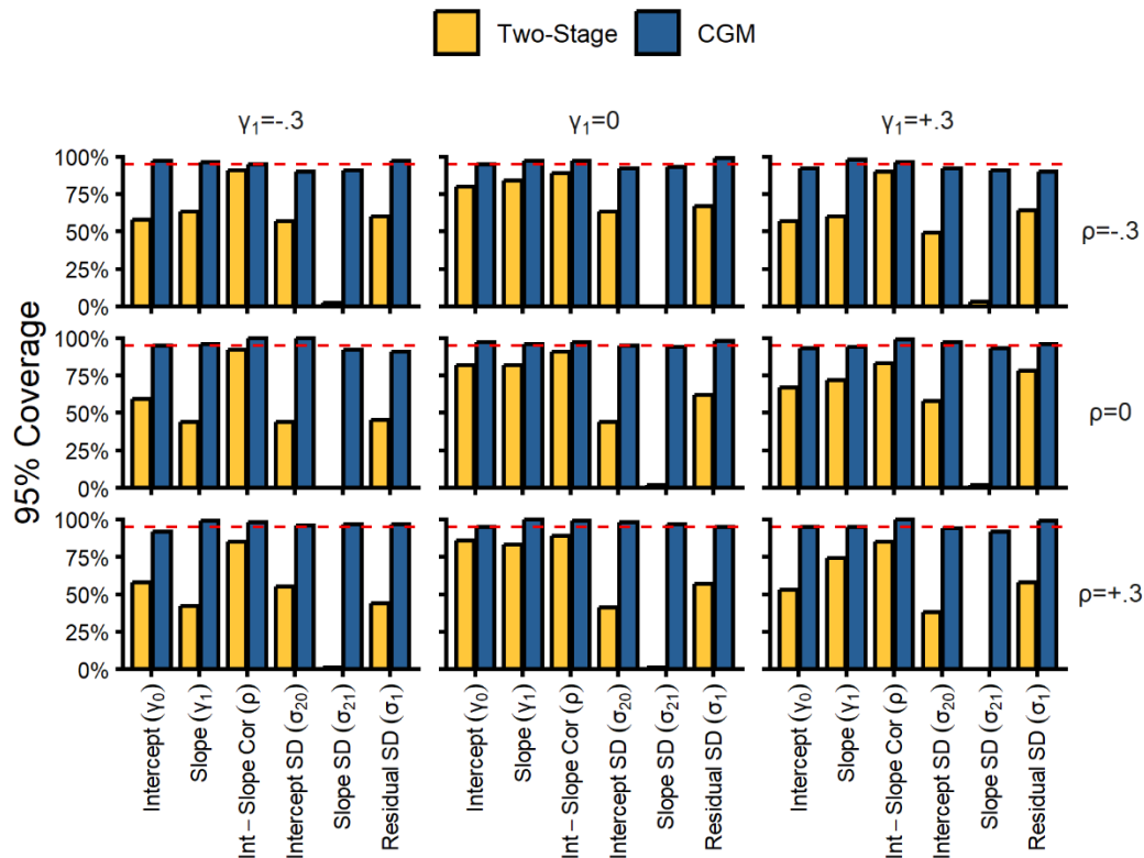
Figure 2 95% Coverage for Group-Level Growth Parameters
