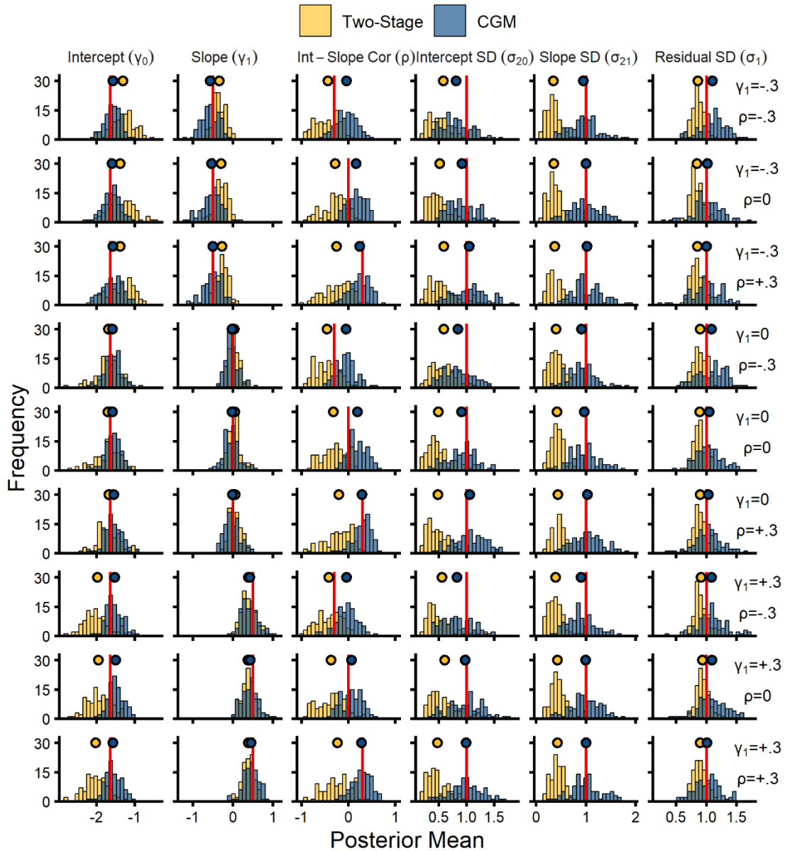
Fig. 1 Distributions of posterior means for group-level growth model parameters. Rows correspond to different simulation conditions and columns correspond to different group-level parameters. Vertical red lines indicate true values and datapoints represent the average of the posterior means across simulations.
