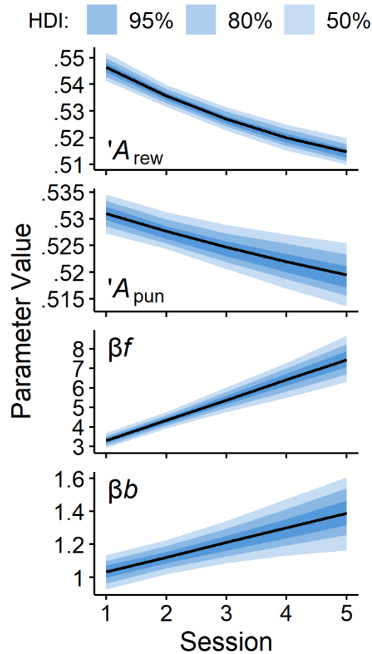
Fig. 6 Posterior predictive growth trajectories for the level 2 component of the unconditional model. Black datapaths show posterior predictive means with errorbands representing highest density intervals (HDIs). We generated these posterior predictions by simulating forward Equation 11 after fitting the unconditional model, including the level 1 error ( E_1 ) and then averaging over the simulated draws (see Online Resource for details).
