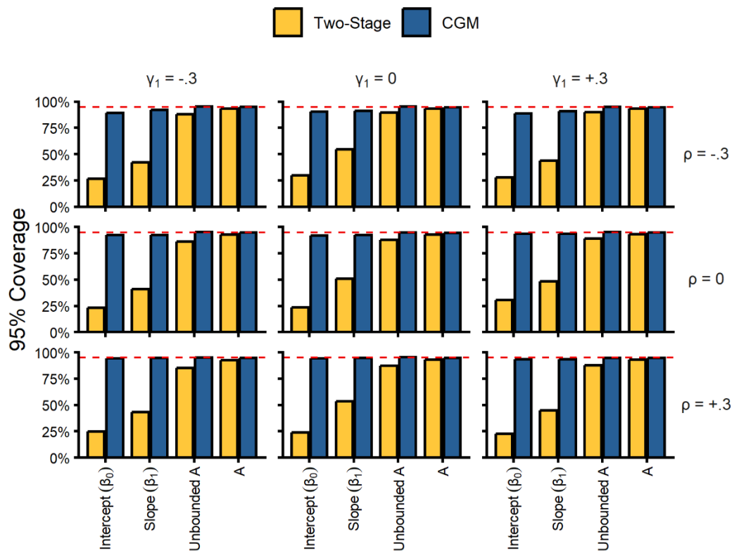
Fig. 4 95% coverage for person-level parameters from each condition across the two-stage and CGM approaches. Rows correspond to different levels of the correlation between intercepts and slopes ( \rho ). Columns correspond to different levels of the slope effect ( \gamma_1 ). The target 95% probability is indicated by the dashed red line.
