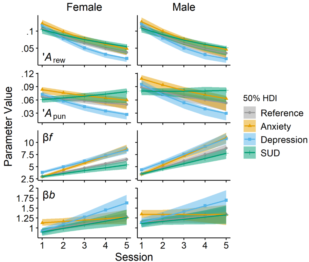
Fig. 8 Posterior predictive growth trajectories for the level 2 component of the conditional model. Reference group refers to participants without a history of anxiety, depression, or substance abuse disorder. We only show the 50% HDI for interpretability purposes, as using wider intervals makes it difficult to visualize individual trajectories and associated uncertainty. We generated these posterior predictions by simulating forward as in Figure 6.
