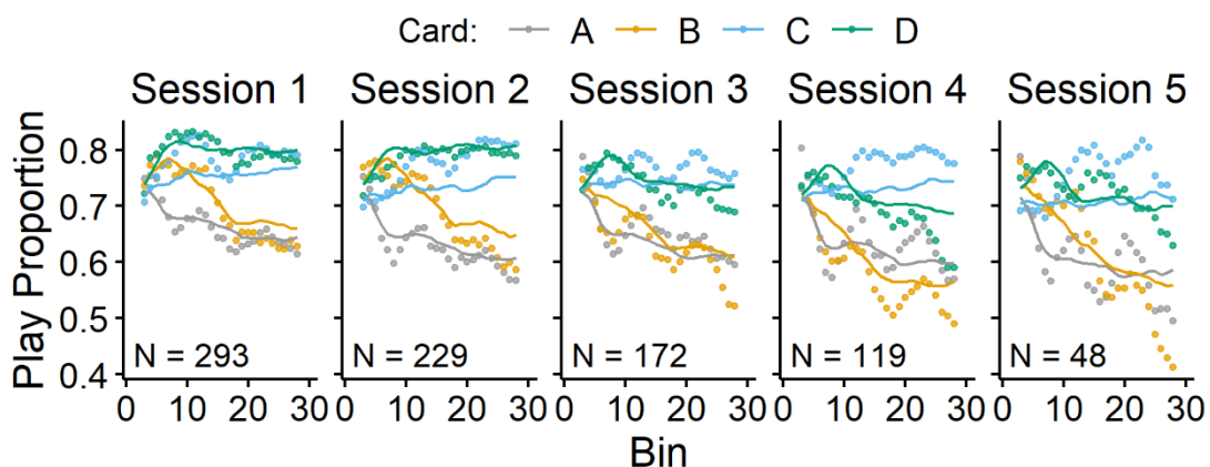
Figure 5 Observed & Model-Predicted Play Proportions
