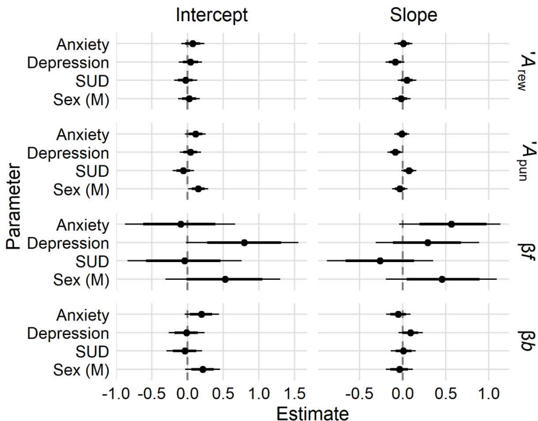
Fig. 7 Posterior distributions for the level 2 growth model terms of the conditional model (a.k.a. fixed effects). For learning rates, the parameter values are still on the untransformed scale (i.e. before the \Phi transform). Thick and thin black intervals indicate the 80% and 95% HDIs, respectively. Black datapoints indicate posterior means.
