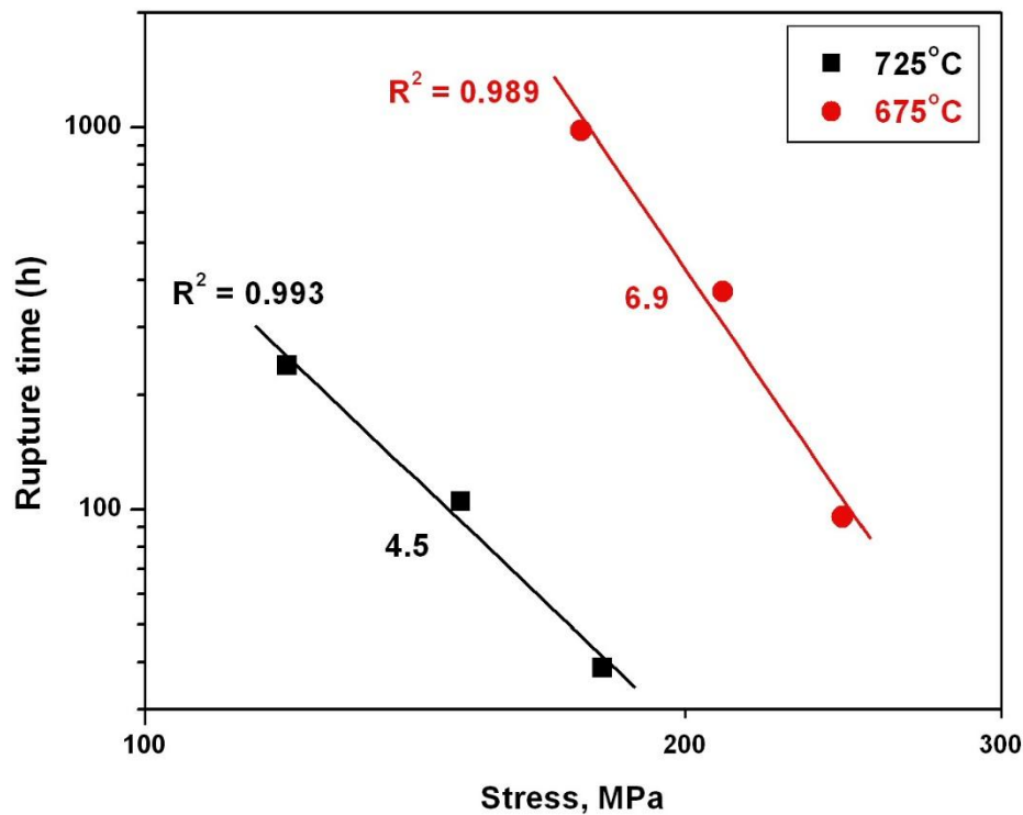
Figure 12 Stress-rupture time relationship used to determine the creep stress exponent at 675 °C and 725 °C.
