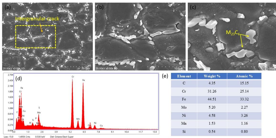
Figure 18 SEM-EDS characterization of creep ruptured sample of 316L stainless steel, tested at 725 °C/120MPa: (a) Intergranular cracking; (b) grain-boundary damage and crack propagation; (c) M_{23}C_6 precipitates; (d) EDS spectrum; and (e) elemental composition.
