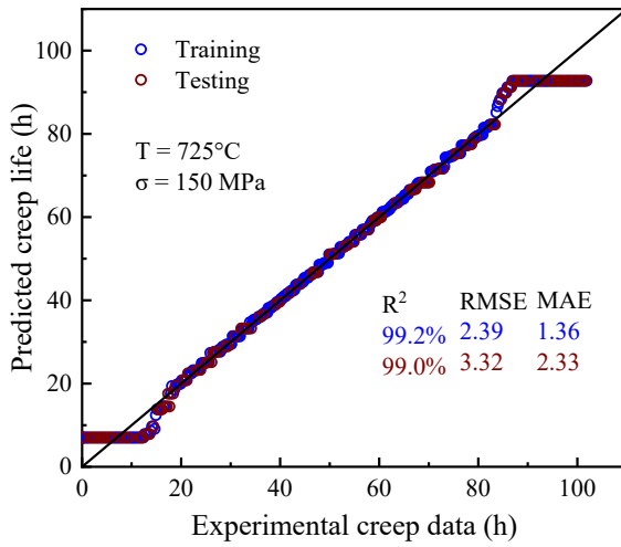
(b) XGBOOST
