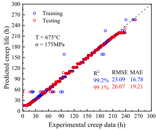
(a) LightGBM
