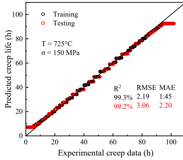
(a) LightGBM
