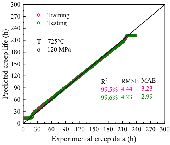
(b) XGBOOST
