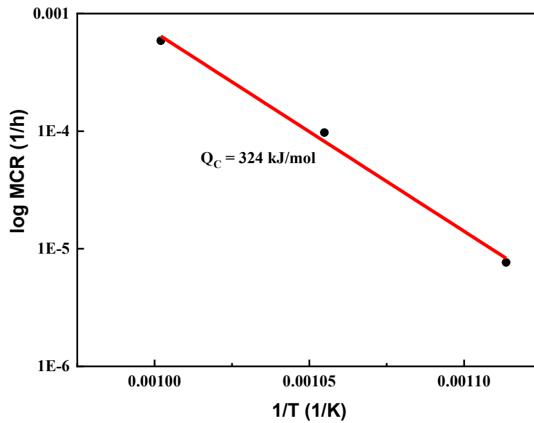
Figure 15 Arrhenius plot of minimum creep rate versus inverse of testing temperature ( 1/T ) used to determine the apparent creep activation energy of 316L ASS, using creep data obtained at 625, 675, and 725 °C.
