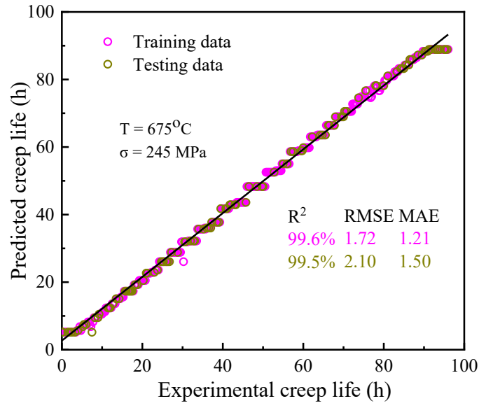
(a) LightGBM
