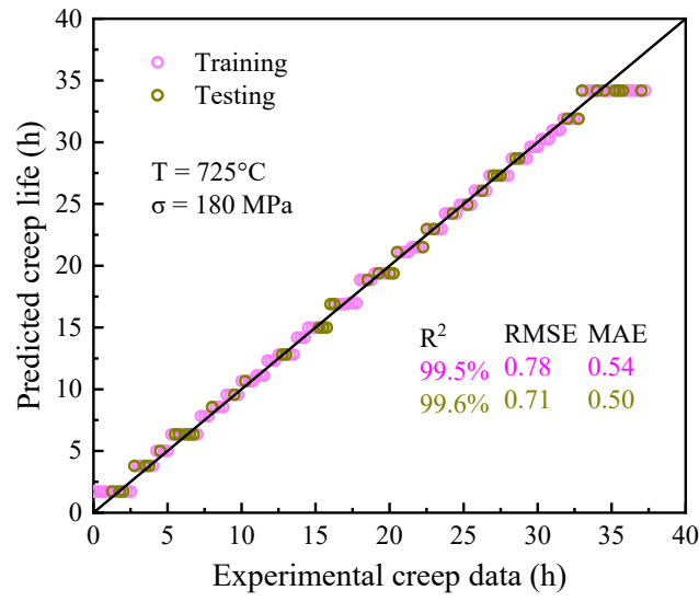
(a) LightGBM
