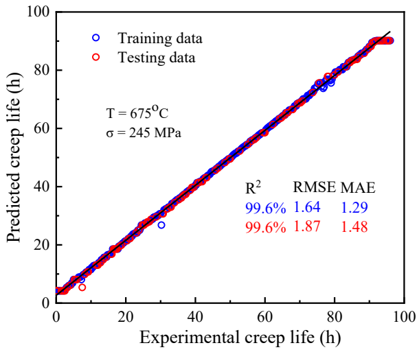
(a) XGBOOST
