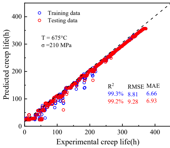
(b) XGBOOST
