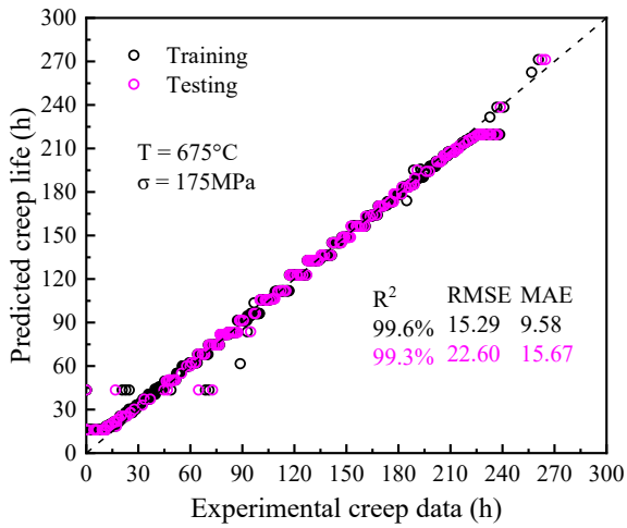
(b)XGBOOST
