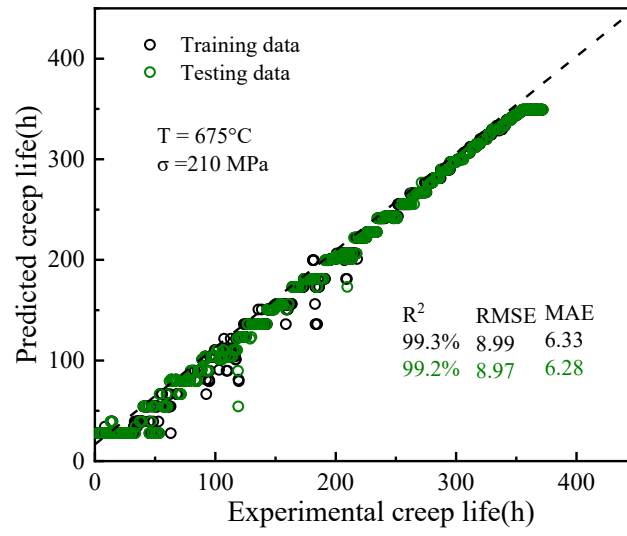
(a) LightGBM
