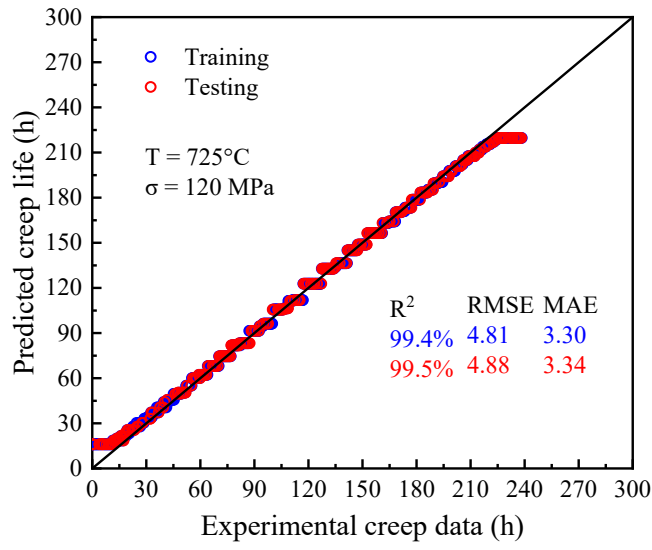
(a) LightGBM
