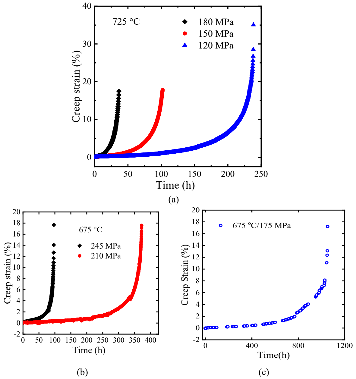
Figure 2 Experimentally measured creep strain–time curves of 316L stainless steel at (a) 725 °C under 180, 150 and 120 MPa, and (b, c) 675 °C under 245, 210 and 175 MPa.
