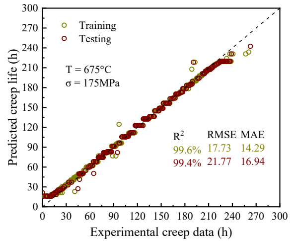
(c)Random Forest
