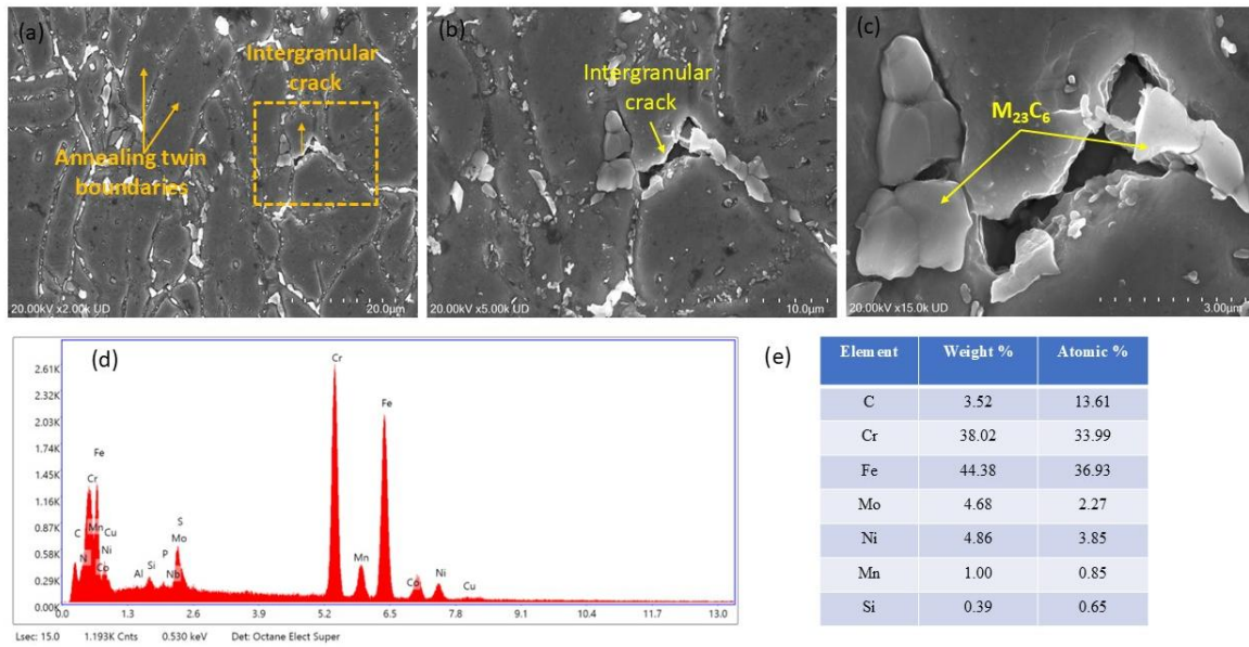
Figure 17 SEM microstructure and EDS analysis of 316L stainless steel sample tested at 675°C/175MPa until ruptured: (a) annealing twin boundaries and intergranular cracking, (b) magnified intergranular crack, (c) grain boundary Cr-rich M_{23}C_6 type carbides precipitates associate with crack propagation, (d) EDS spectrum, and (e) corresponding elemental composition.
