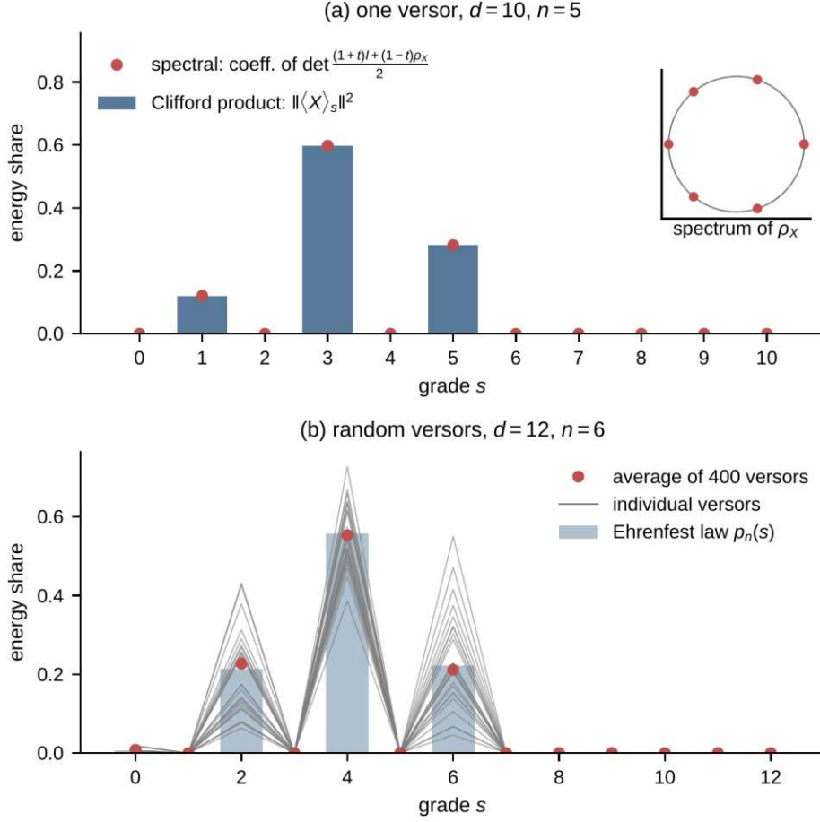
Fig. 1. (a) Grade energies of a random product of 5 unit vectors in \mathbb{R}^{10} (bars), and the coefficients of \det \left( \frac{(1+t)I + (1-t)\rho_X}{2} \right) (dots). The inset shows the spectrum of \rho_X . (b) Profiles of individual random versors ( d = 12, n = 6 ; thin lines) and their average over 400 samples (dots), compared with the Ehrenfest law of Theorem 5.1 (bars).
