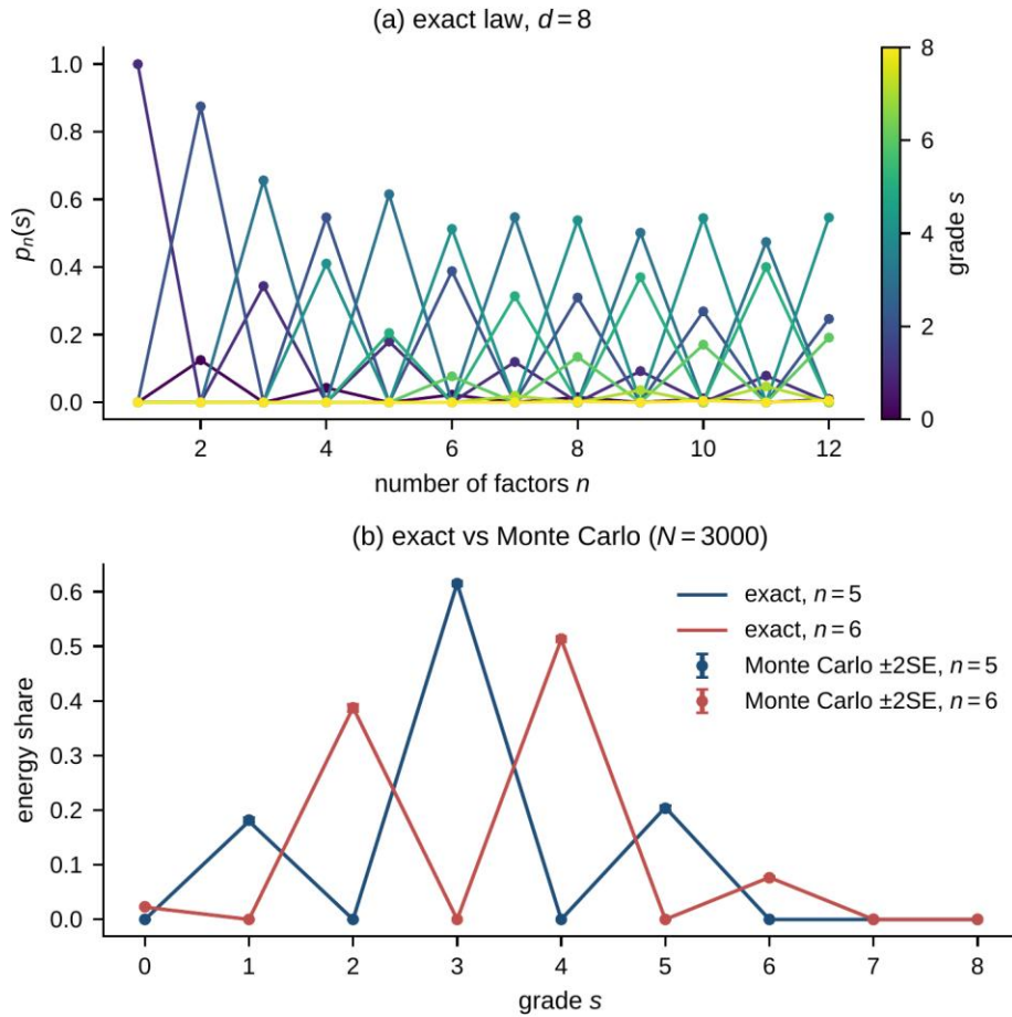
Fig. 2. (a) Exact Ehrenfest law p_n(s) for d = 8 . (b) Exact p_5 and p_6 against Monte Carlo averages over uniform unit vectors ( N = 3000 , \pm 2 standard errors).
