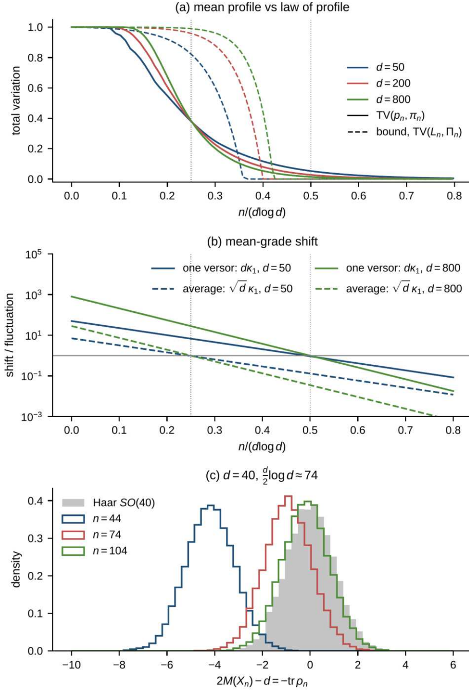
Fig. 3. The two-scale cut-off. (a) Exact TV(p_n, \pi_n) (solid) and the lower bound of Theorem 7.5(a) for TV(L_n, \Pi_n) (dashed, clipped at 0) for d = 50, 200, 800 ; as d \rightarrow \infty the cut-offs are at n/(d \log d) = \frac{1}{4} and \frac{1}{2} . (b) Shift of the mean grade from d/2 in units of its fluctuation: d\kappa_1 for an individual versor (solid) and \sqrt{d}\kappa_1 for the averaged profile (dashed). (c) Monte Carlo samples of 2M(X_n) - d = -\text{tr} \rho_n in d = 40 for n = 44, 74, 104 (12,000 samples each), against Haar measure on SO(40) .
