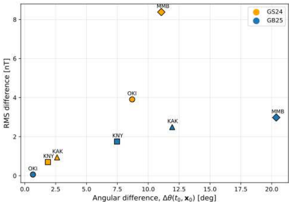
Fig. 11. Relationship between angular difference and RMS difference between CDV correction and IGRF-DI correction. Orange and blue symbols represent the GS24 and GB25 cruises, respectively.
