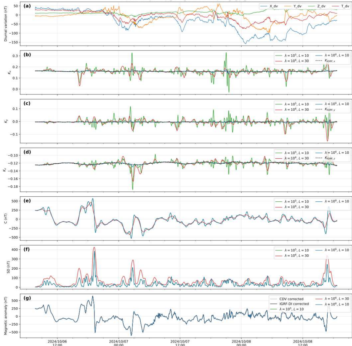
Fig. 10. Example of moving-window LS-DI correction with different regularization parameters \lambda and half-window lengths L [min]. For data sampled at 1-min intervals, a half-window length of L corresponds to a maximum window size of 2L + 1 data points. The results were obtained by applying the correction to data from the Memambetsu (MMB) observatory during the GS24 cruise. (a) Observed variations in the three magnetic-field components ( X_{dv} , Y_{dv} , Z_{dv} ) and total magnetic intensity ( T_{dv} ). (b–d) Estimated coefficients K_x , K_y , and K_z , respectively. The black dashed lines indicate the corresponding
