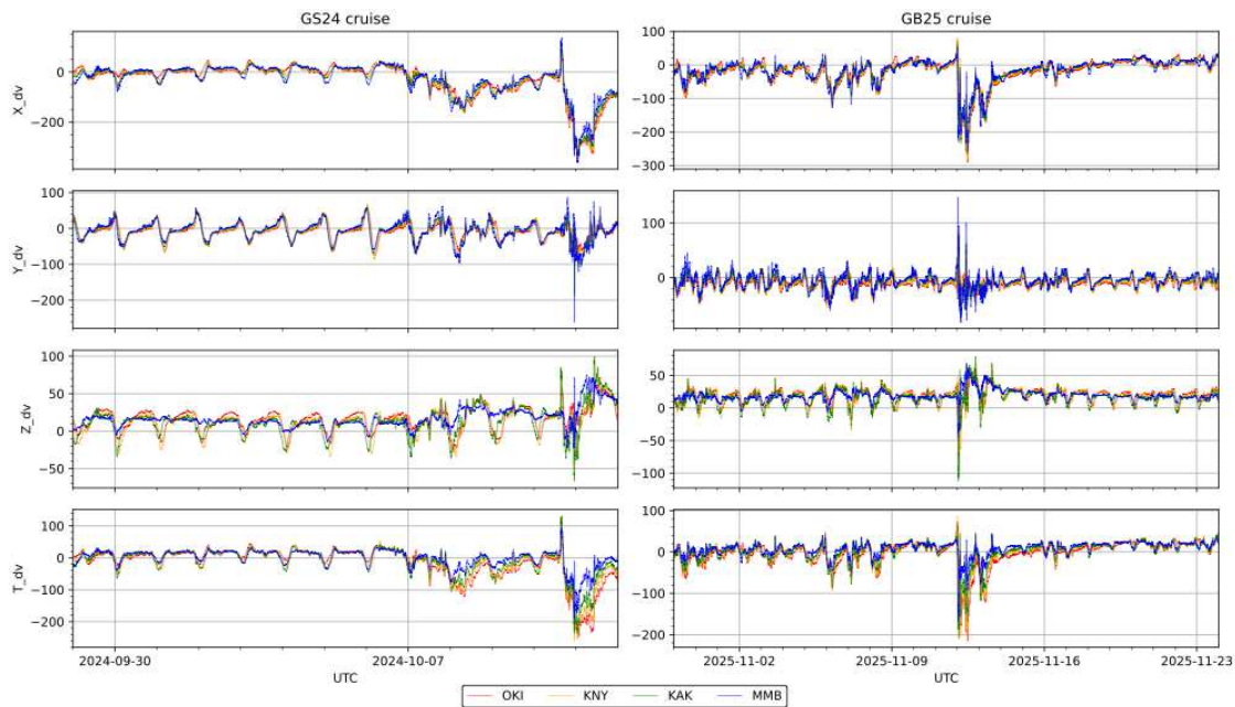
Fig. 3. Diurnal variations during the GS24 (left) and GB25 (right) cruises at Okinawa (red lines), Kanoya (orange lines), Kakioka (green lines), and Memambetsu (blue lines) observatories. From top to bottom, the panels show the diurnal variations of the X (North), Y (East), Z (Down) components and the total magnetic intensity [nT]. The constant values ( T_{base} and B_{base} ) were subtracted to derive the diurnal variations for each cruise and observatory; these values are listed in Table 1.
