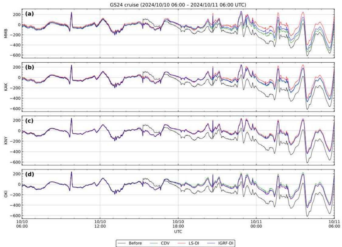
Fig. 4. Comparison of magnetic anomaly data before and after diurnal variation and DI corrections during the GS24 cruise from 06:00 UTC on 10 October to 06:00 UTC on 11 October 2024. From top to bottom, the panels show results obtained using data from the (a) Memambetsu (MMB), (b) Kakioka (KAK), (c) Kanoya (KNY), and (d) Okinawa (OKI) geomagnetic observatories, respectively. Black curves show the data before diurnal variation correction, green curves show the data after CDV-correction, red curves show the results after the LS-DI correction, and blue curves show the results after IGRF-DI correction.
