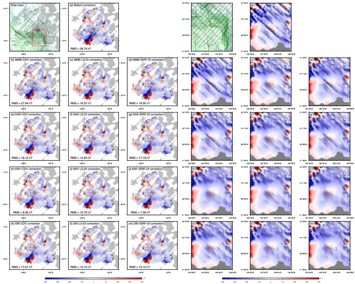
Fig. 5. Total magnetic anomaly maps and ship track lines during the GS24 cruise. Color palette for bathymetry is same to Fig.1. (a) Total magnetic anomaly before diurnal variation correction. Panels (b)–(d) show the total magnetic anomaly after (b) CDV, (c) LS-DI, and (d) IGRF-DI correction using Memambetsu (MMB) observatory data. Panels (e)–(g) show the total magnetic anomaly after (e) CDV, (f) LS-DI, and (g) IGRF-DI correction using Kakioka (KAK) observatory data. Panels (h)–(j) show the total magnetic anomaly after (h) CDV, (i) LS-DI, and (j) IGRF-DI correction using Kanoya (KNY) observatory data. Panels (k)–(m) show the total magnetic anomaly after (k) CDV, (l) LS-DI, and (m)
