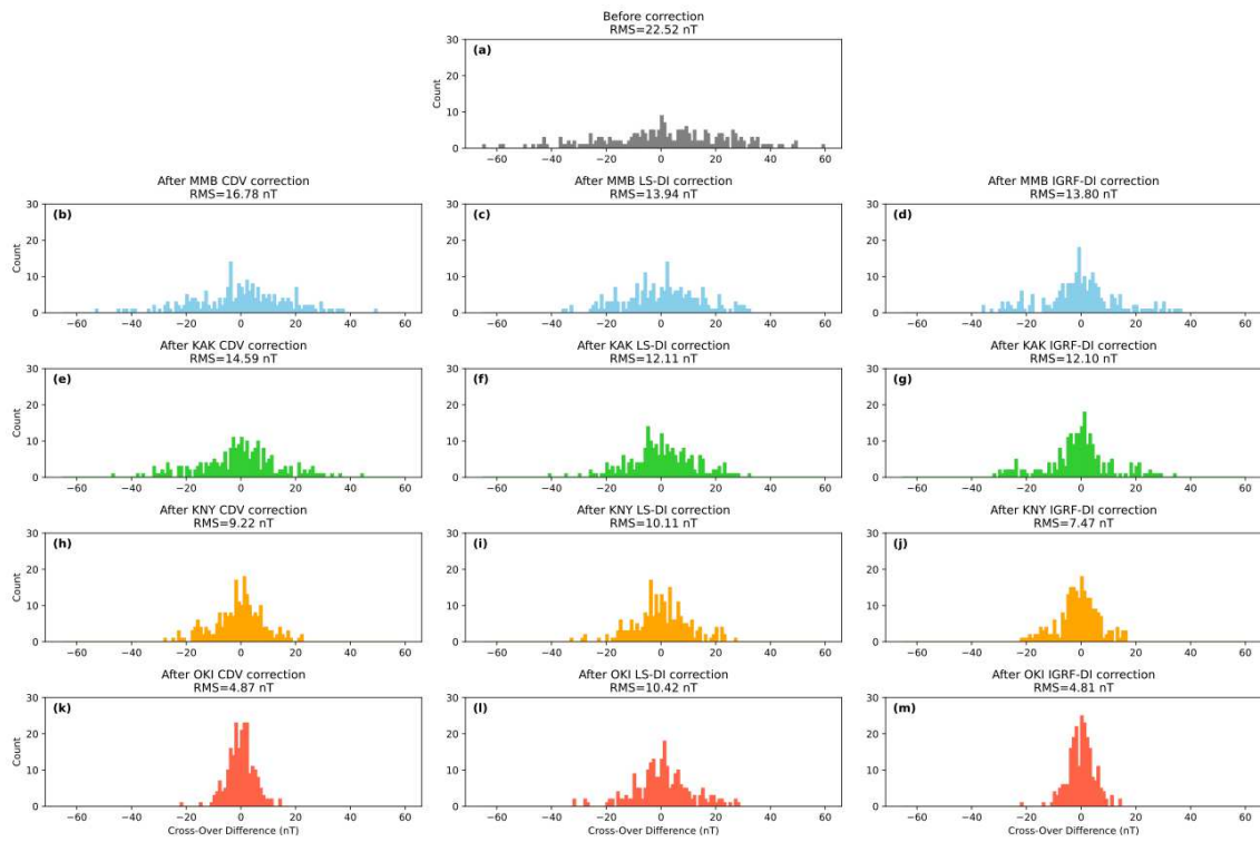
Fig. 9. Histograms of cross-over differences (CODs) during the GB25 cruise. The other details are the
