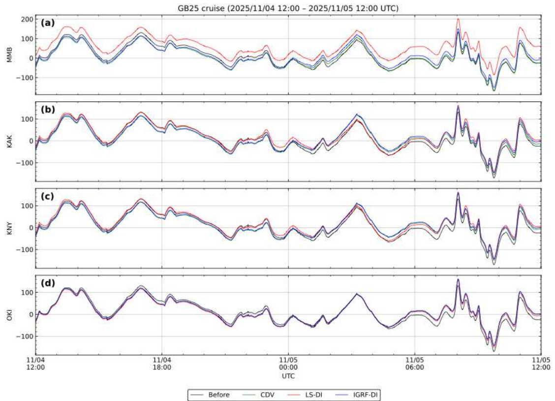
Fig. 7. Comparison of magnetic anomaly data before and after CDV, LS-DI, and IGRF-DI corrections during the GB25 cruise from 12:00 UTC on 4 November to 12:00 UTC on 5 November 2025. The other details are the same as in Fig. 4.
