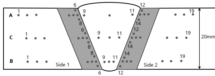
Figure 12. Locations of hardness indentations in the GTAW plate joint
