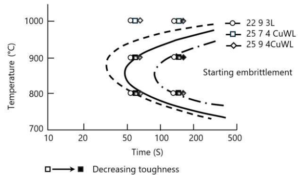
Figure 4. TTP curves of duplex and super duplex welds including one from a ZERON 100X(A) weld (typical PREN 40.5) based on loss of toughness [27]
