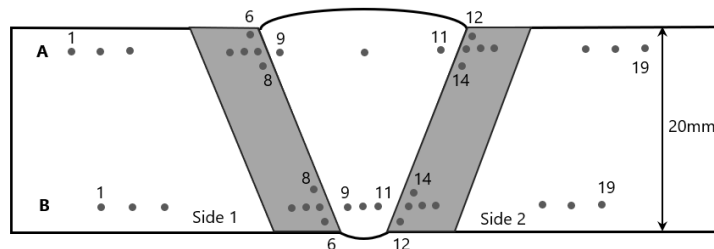
Figure 14. Locations of hardness indications in the weld joint of the synergic P-GMAW weld
