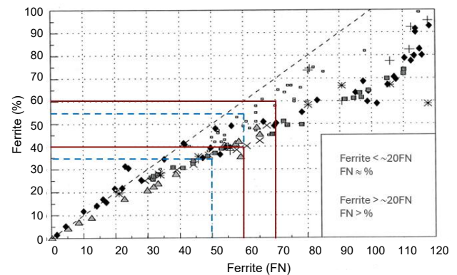
Figure 2. The expected ferrite content ranges from the ZERON 100X compositions [23]
