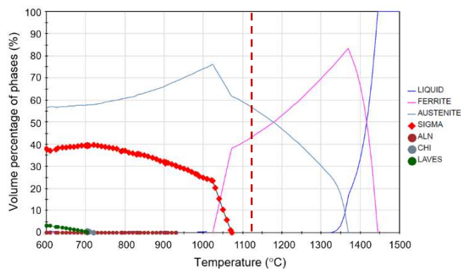
Figure 1. Predicted equilibrium phase fraction of Zeron 100X(B) composition
