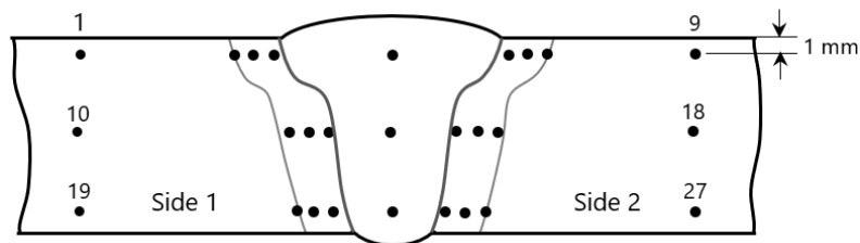
Figure 7. Illustration of hardness test indentation locations
