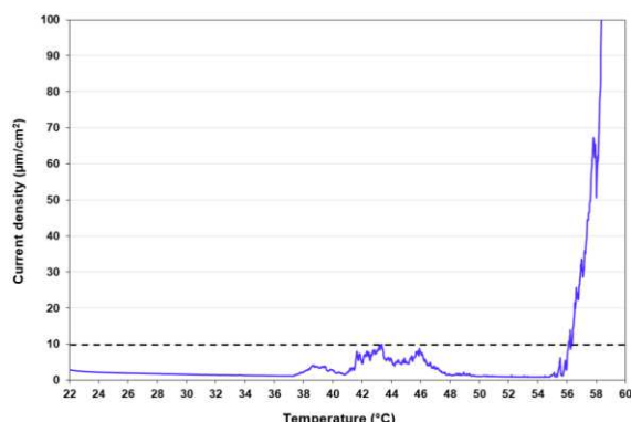
Figure 9. A typical plot of the current density changes with increasing temperature and a photograph of the root run of the weld on completion of the test showing the sites of pitting corrosion attack
