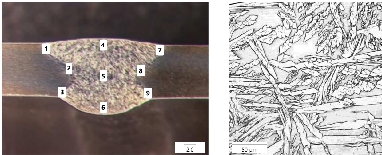
Figure 6. Microstructure of the 2" Sch. 40S, Ar+2%N 2 / Ar weld joint using ZERON 100X(B) rod
