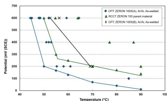
Figure 19. Effect of potential on RCCT of ZERON 100 parent material and CPT of ZERON 100 X(A) and ZERON 100X(B) GTAW Joints
