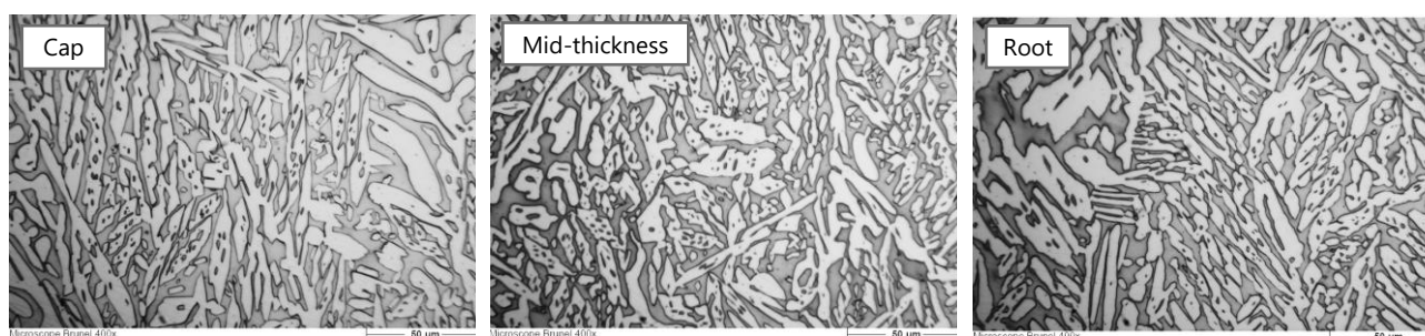
Figure 15. Microstructure of the manual synergic P-GMAW weld after post weld solution heat treatment
