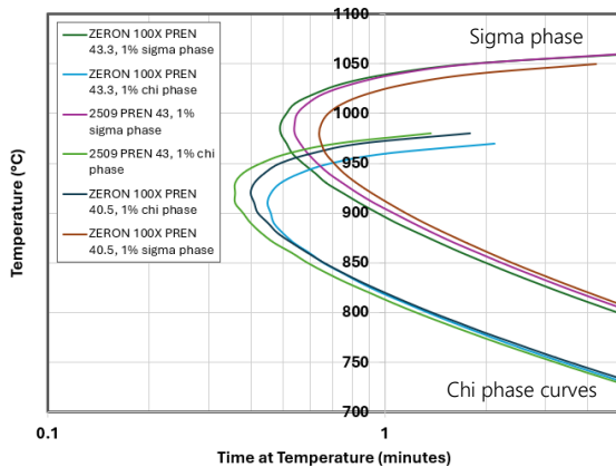
Figure 3. Predicted weld TTP curves for precipitation of 1% sigma phase and 1% chi phase in each of the alloys.
