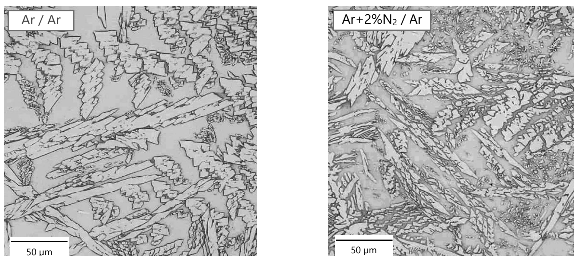
Figure 11. Microstructure of root weld of the 20 mm thick GTAW joint from ZERON 100X(B) rod
