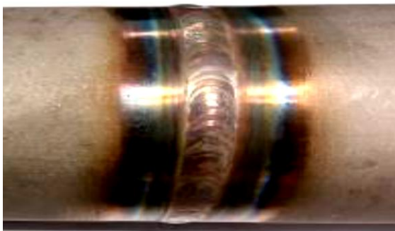
Figure 5. Surface appearances of the cap and root weld passes of the pipe joint
