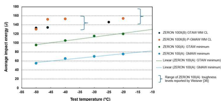
Figure 18. Charpy transition curves of ZERON 100X(B) GTAW and synergic P-GMAW weld metals
