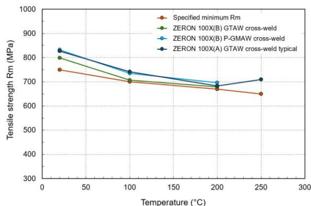
Figure 17. Cross-weld tensile strength of weld joints of ZERON 100X(A) and ZERON 100X(B) vs specified minimum requirements
