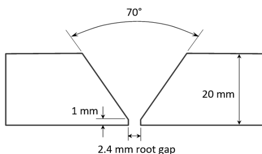
Figure 10. Illustration of joint geometry and run sequence of GTAW and P-GMAW butt welds
