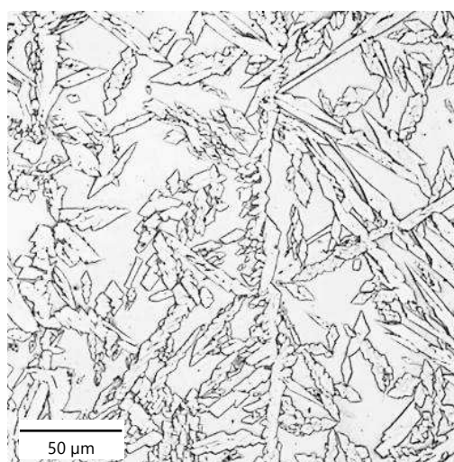
Figure 13. Microstructure of the weld root of the 20 mm thick plate weld joint produced with synergic P-GMAW using ZERON 100X(B) wire
