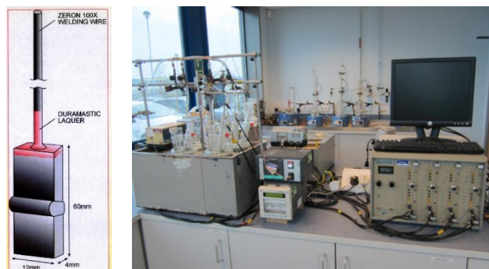
Figure 8. Schematic illustration of the corrosion test specimen and the test set unit The current density and temperature were monitored continuously throughout the test. Pitting was said to have initiated when the current density exceeded 10 \mu\text{A}/\text{cm}^2 , if the passive current density at room temperature was less than 1 \mu\text{A}/\text{cm}^2 . This follows the criteria set by Oldfield and Sutton [32]. After testing, the samples were washed, dried and examined under a microscope for indications of
