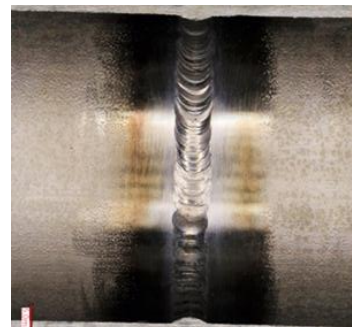
Figure 5. Surface appearances of the cap and root weld passes of the pipe joint
