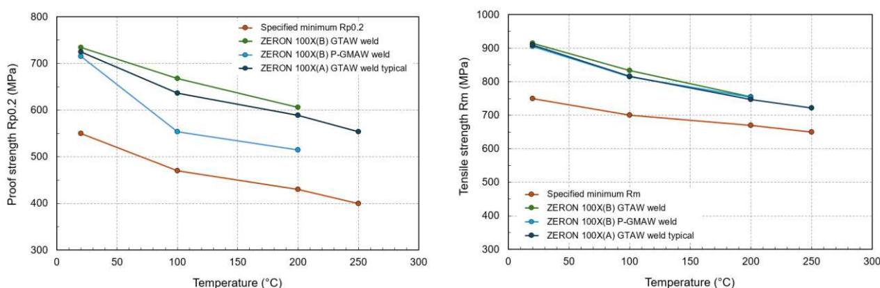
Figure 16. Weld R_{p0.2} and R_m strength vs specified minimum
