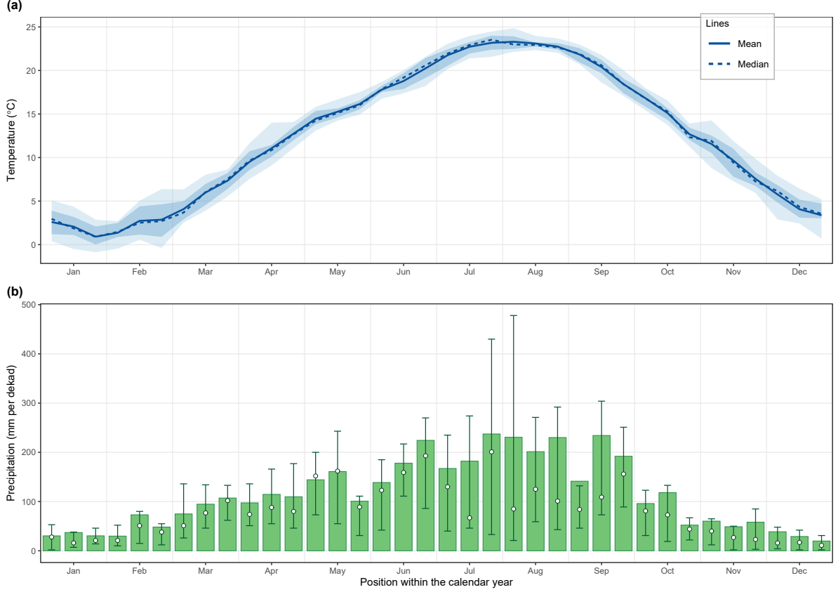
Fig. 2 Dekadal climatology of the Yanase environment during 1981–2005, the 25 complete years shared by the two datasets. (a) ERA5-Land 2-m air temperature averaged over the 3 \times 3 grid-cell domain. Solid and dashed lines show the arithmetic mean and median, respectively; dark and light shading denote the interquartile and 10th–90th percentile ranges. (b) JMA Yanase precipitation. Bars show mean precipitation per dekad, open points show medians, and vertical intervals show the interquartile range. Temperature is drawn from ERA5-Land because Yanase has no temperature record. Fixed predictor windows and the complete monthly and dekadal response surfaces are reported in Fig. 4 and Supplementary Figs. S4–S7
