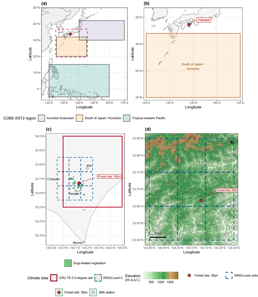
Fig. 1 Spatial setting of the Yanase study and climate-data domains. (a) Ocean–atmosphere context over Northeast Asia and the western North Pacific, showing the three fixed COBE-SST2 regional means; the dashed rectangle marks panel (b). (b) Western Japan and adjacent waters, showing forest site 39yn, the South-of-Japan/Kuroshio region, and the extent enlarged in panel (c). (c) Sugi-related vegetation, the JMA stations at Yanase, Kito, Odochi, and Murotomisaki, the CRU TS 0.5-degree cell containing the site (the four-point interpolation support is specified in the Supplementary Material), the individual ERA5-Land 0.1-degree cells in the 3 \times 3 averaging domain, and forest site 39yn. (d) Elevation and contours across the complete ERA5-Land domain, with forest site 39yn, the individual grid cells, a 5-km scale bar, and north orientation. Map lines delineate study areas and do not necessarily depict accepted national boundaries
