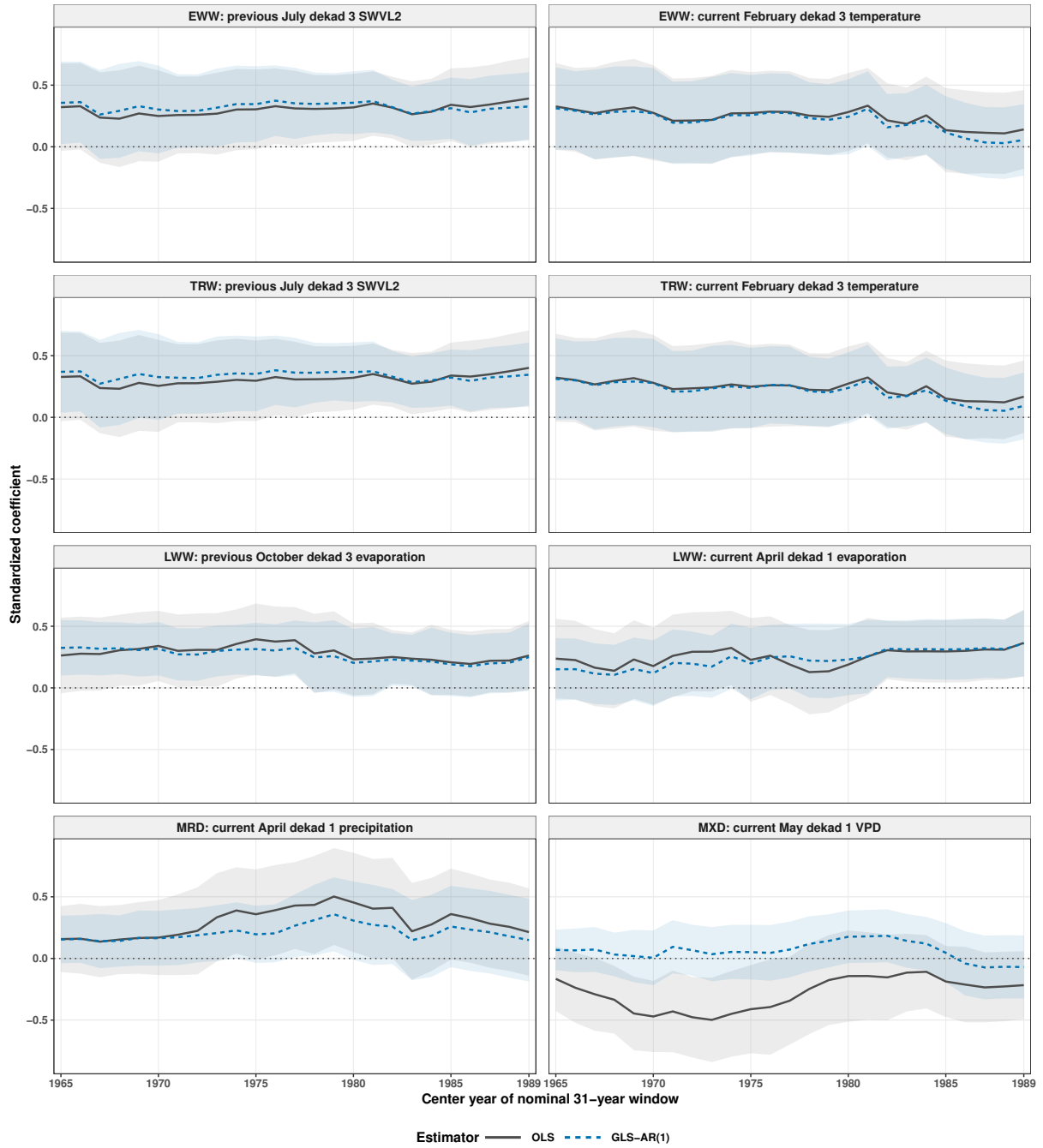
Fig. 5 Temporal stability of the selected climate-growth coefficients in 31-year moving windows. Predictors and responses were standardized with the full-period 1950–2004 scaling before each window was fitted. Previous-July soil water for EWW and TRW, previous-October and current-April evaporation for LWW, and current-April precipitation for MRD retained their expected signs in the required fraction of windows. The May VPD coefficient for MXD repeatedly changed sign, supporting its classification as temporally unstable
