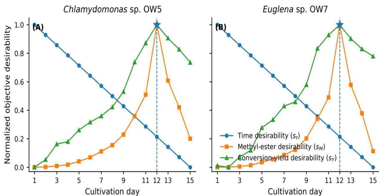
Figure 3: Normalized objective trajectories reveal the temporal trade-off between cultivation time, methyl-ester output and conversion yield
