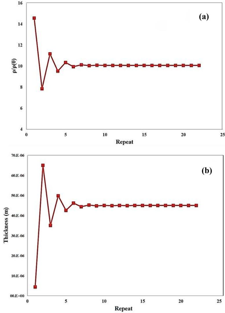
Fig 7. Calculation of unknown thickness with measured surface resistance R_s = 0.002358 (a) Iteration \rho/\rho_0 , (b) Iteration of thickness.
