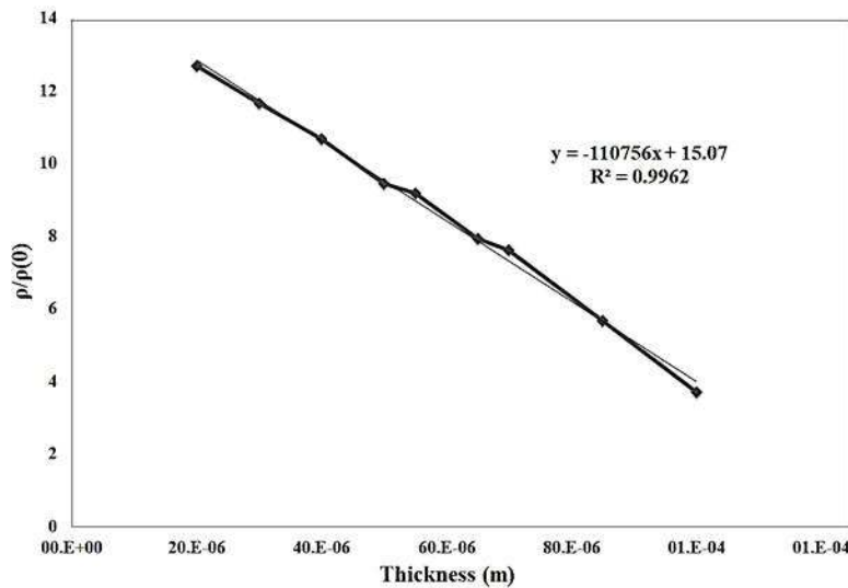
Fig 6. Variation of \rho/\rho_0 as a function of thickness.
