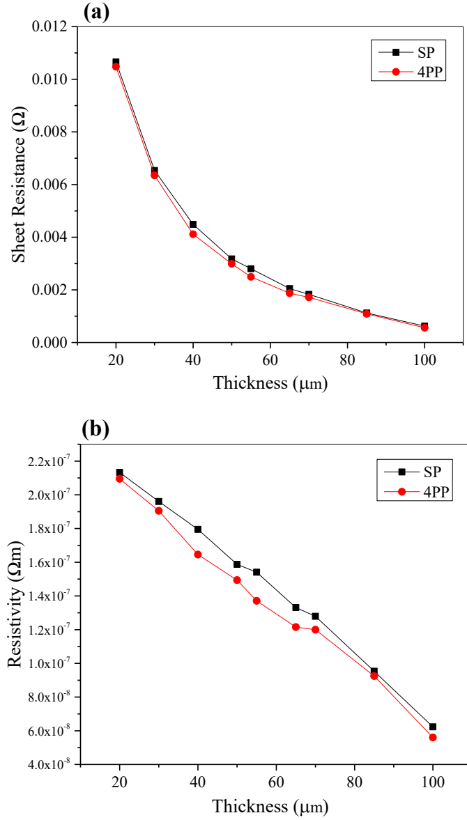
Fig. 5. (a) Sheet resistance and (b) electrical resistivity as a function of thickness measured by single-probe and four-point probe methods.
