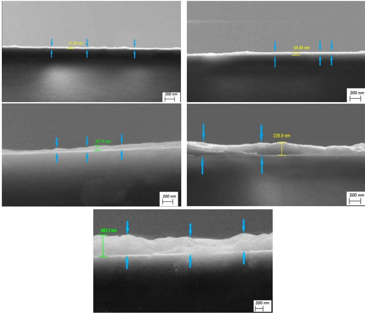
Fig 9. Cross-sectional FESEM image of the cross-sectional surface of pure copper coating with the thickness of about (a) 34 nm, (b) 53 nm, (c) 90 nm, (d) 213 nm, and (e) 529 nm.
