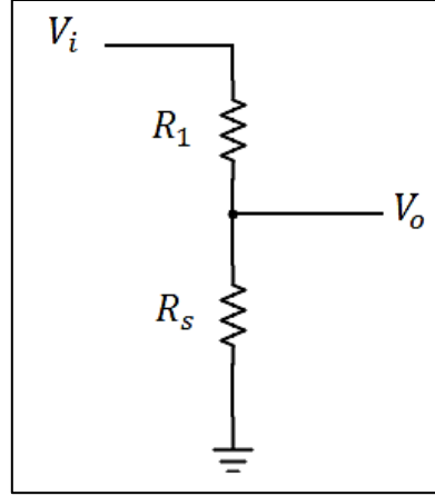
Fig. 2. Voltage divider circuit for sheet resistance measurement.
