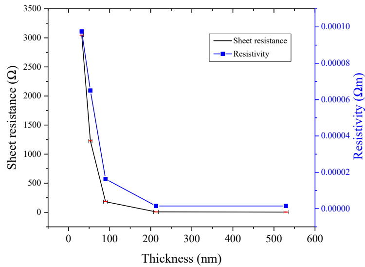
Fig. 10. Sheet resistance and electrical resistivity as a function of thickness measured by single-point probe method in nanometer thicknesses.
