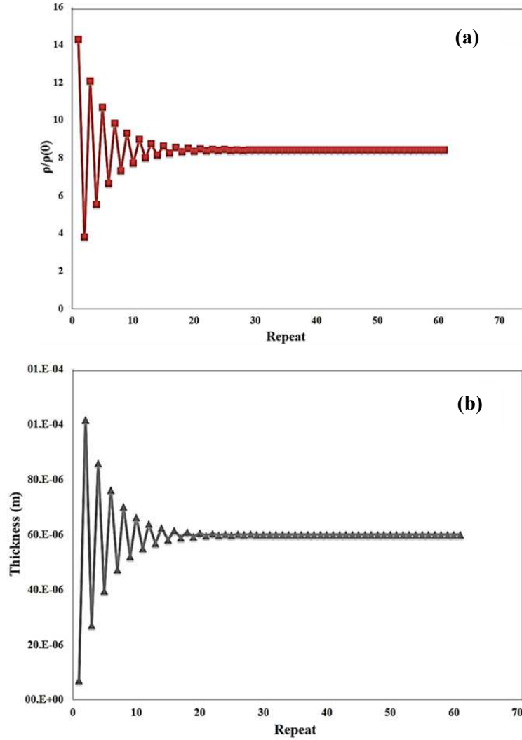
Fig 8. Calculation of unknown thickness with measured surface resistance R_s = 0.003765 . (a) Iteration \rho/\rho_0 , (b) Iteration of thickness.
