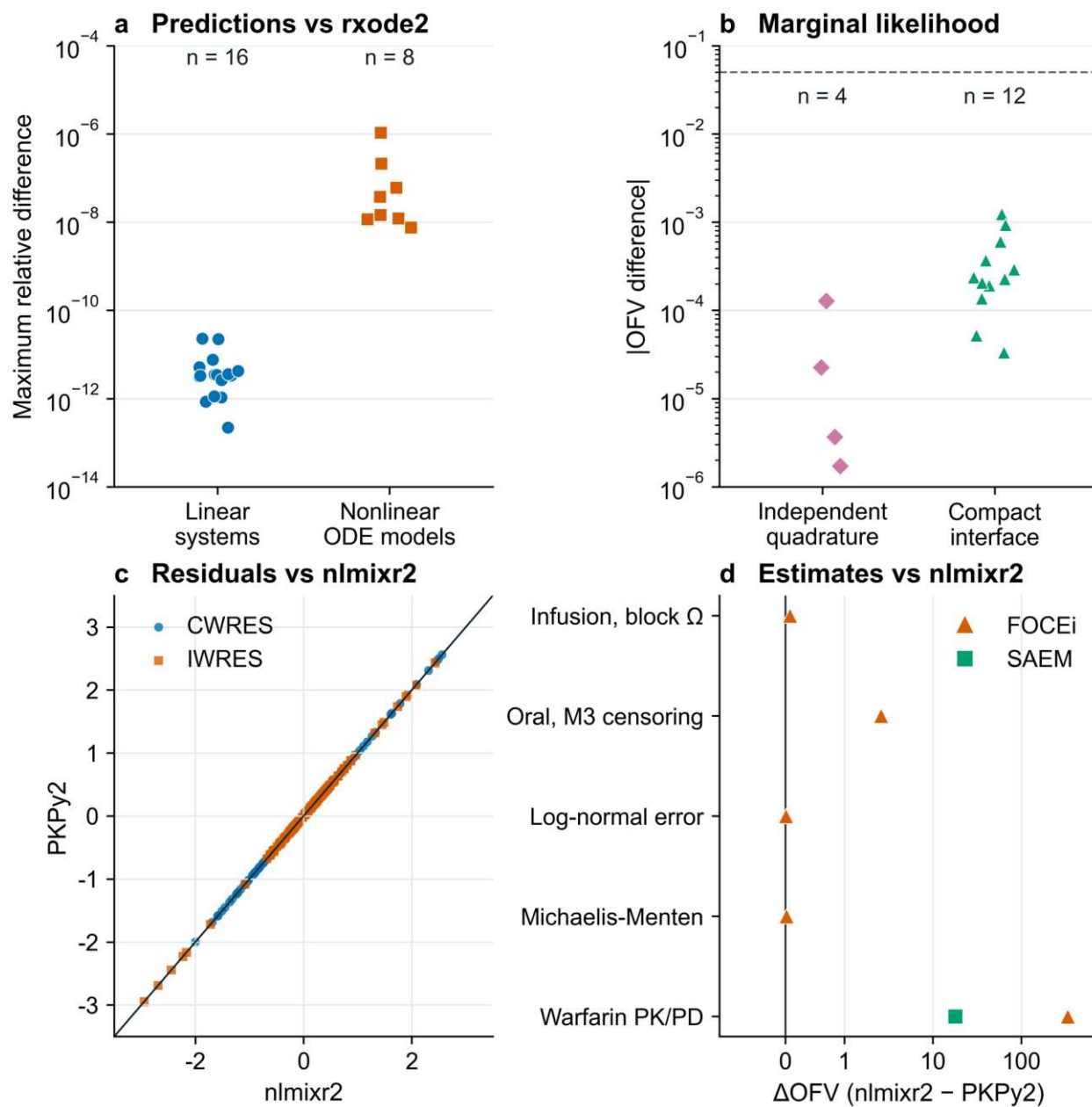
Fig. 6 Verification of the event-record interface. (a) Maximum relative differences of PKPy2 predictions from rxode2 in linear and nonlinear (ODE) scenarios. (b) Absolute OFV differences from an independent quadrature implementation and from the compact interface; the dashed line marks the convergence tolerance of 0.05. (c) CWRES and IWRES of the theophylline model from PKPy2 and nlmixr2 at identical parameters. (d) Exact OFV at the nlmixr2 FOCEi and SAEM estimates minus that at the PKPy2 estimates
