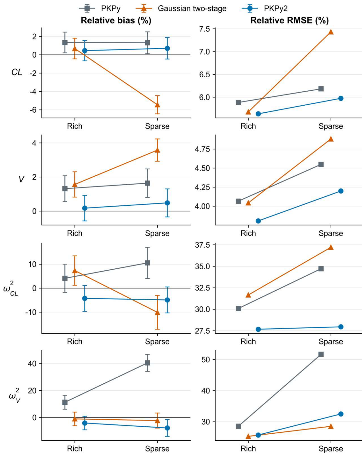
Fig. 2 Parameter recovery in the primary simulation by PKPy, the Gaussian two-stage control, and PKPy2. Left, relative bias with \pm 1.96 Monte Carlo standard errors; right, relative root mean squared error (RMSE). Each point summarizes 100 datasets (98 for the rich-sampling Gaussian control)
