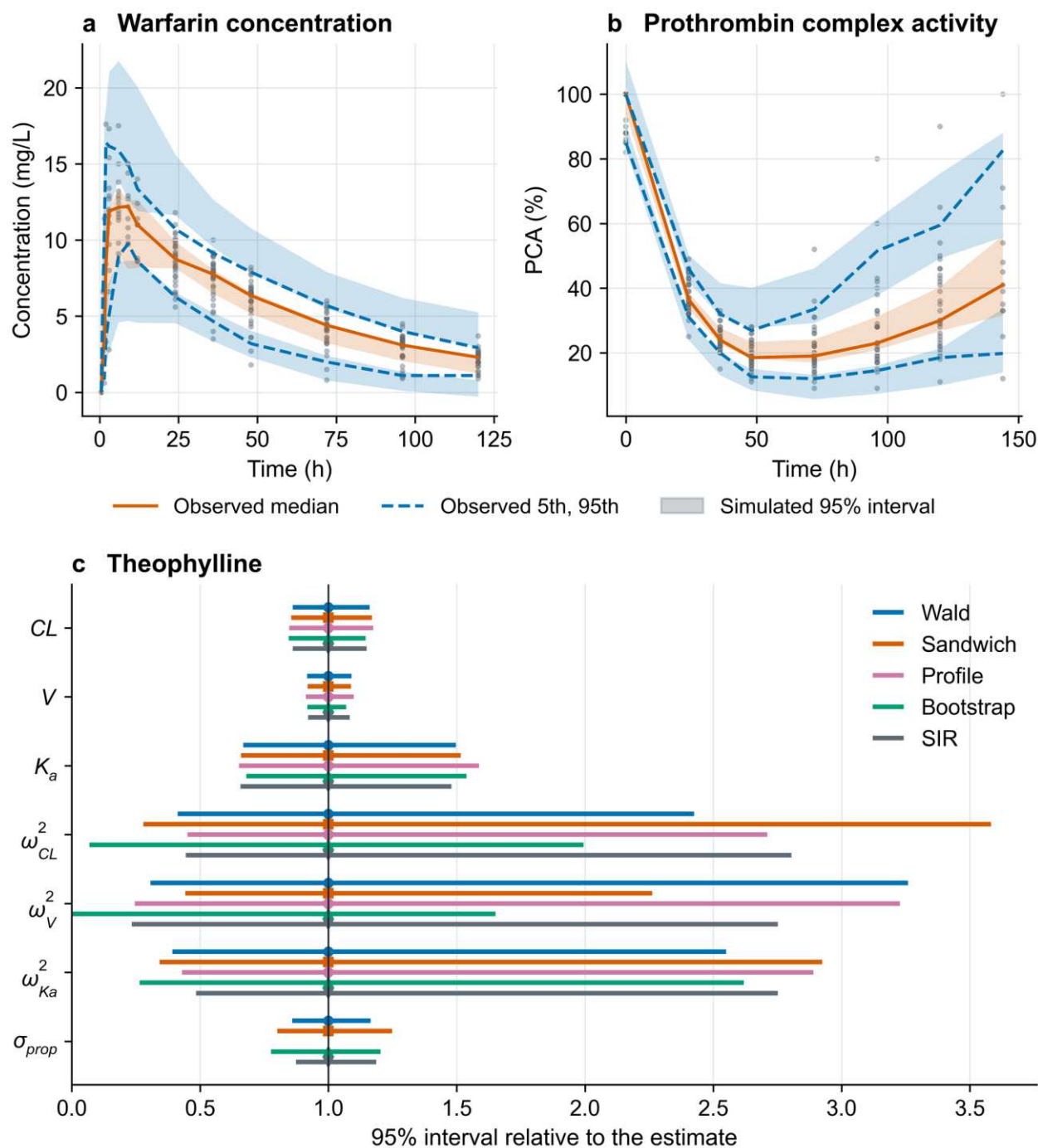
Fig. 7 Warfarin PK/PD application and interval methods. (a, b) Visual predictive checks of plasma concentration and prothrombin complex activity (PCA): observed 5th, 50th, and 95th percentiles (lines), 95% intervals of the simulated percentiles (bands), and observations (points). (c) 95% intervals for the theophylline model from the Wald, sandwich, profile-likelihood, bootstrap, and SIR methods, relative to the estimate
