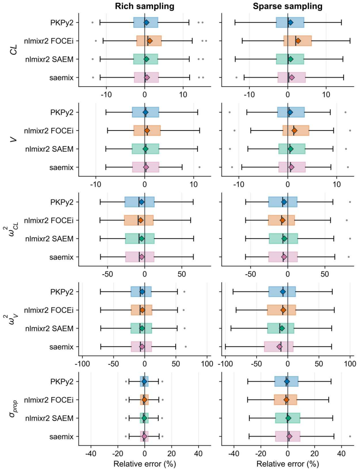
Fig. 5 Relative errors of PKPy2, nlmixr2 FOCEi, nlmixr2 SAEM, and saemix estimates in the 200 primary simulation datasets. Boxes show medians and interquartile ranges, whiskers extend to 1.5 times the interquartile range, and diamonds mark means
