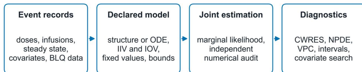
Fig. 1 Population inference in PKPy and PKPy2. (a) PKPy fits each subject separately and summarizes the individual log parameters. (b) PKPy2 reads event records, fits the declared population model jointly by marginal likelihood with an independent numerical audit, and provides diagnostics and interval estimates
