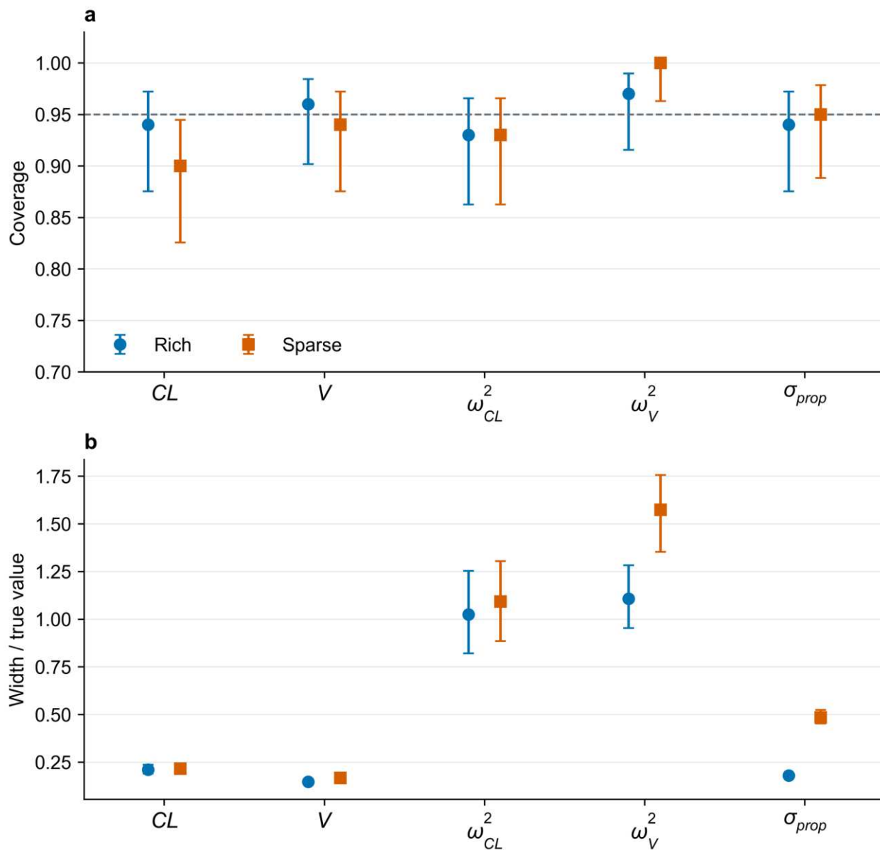
Fig. 3 Coverage (a) and width (b) of PKPy2 95% confidence intervals in the primary simulation. Error bars in (a) are Wilson 95% intervals, and the dashed line marks 95%. Widths are medians relative to the true value, with interquartile ranges
