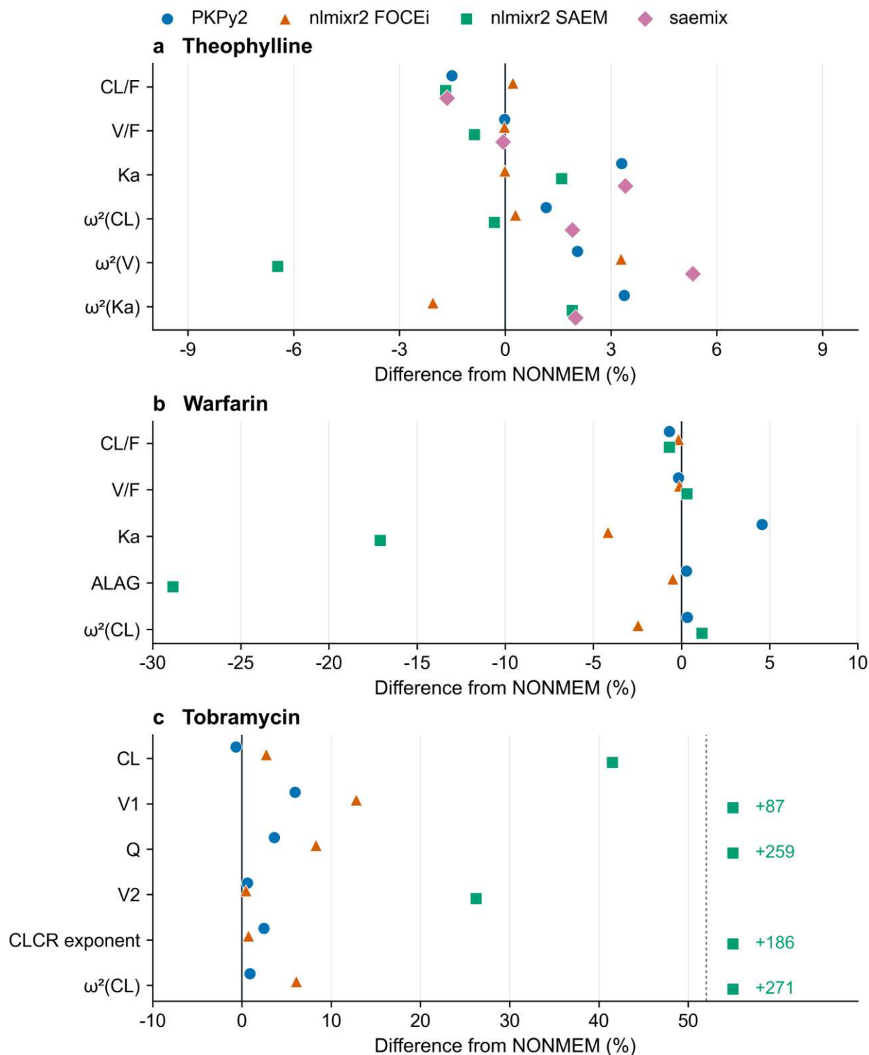
Fig. 4 Differences of the theophylline (a), warfarin (b), and tobramycin (c) estimates from the published expert NONMEM estimates. Tobramycin estimates were obtained with the expert-judgment constraints. Differences larger than 50% are plotted to the right of the dotted line and labeled with their values
