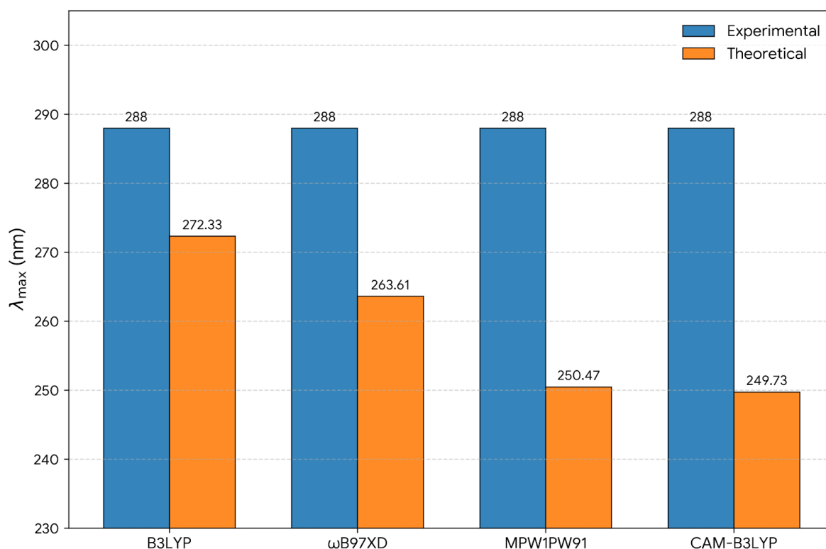
Fig 2 Benchmark of DFT functionals against experimental UV-Vis absorption maximum ( \lambda_{\max} ).
