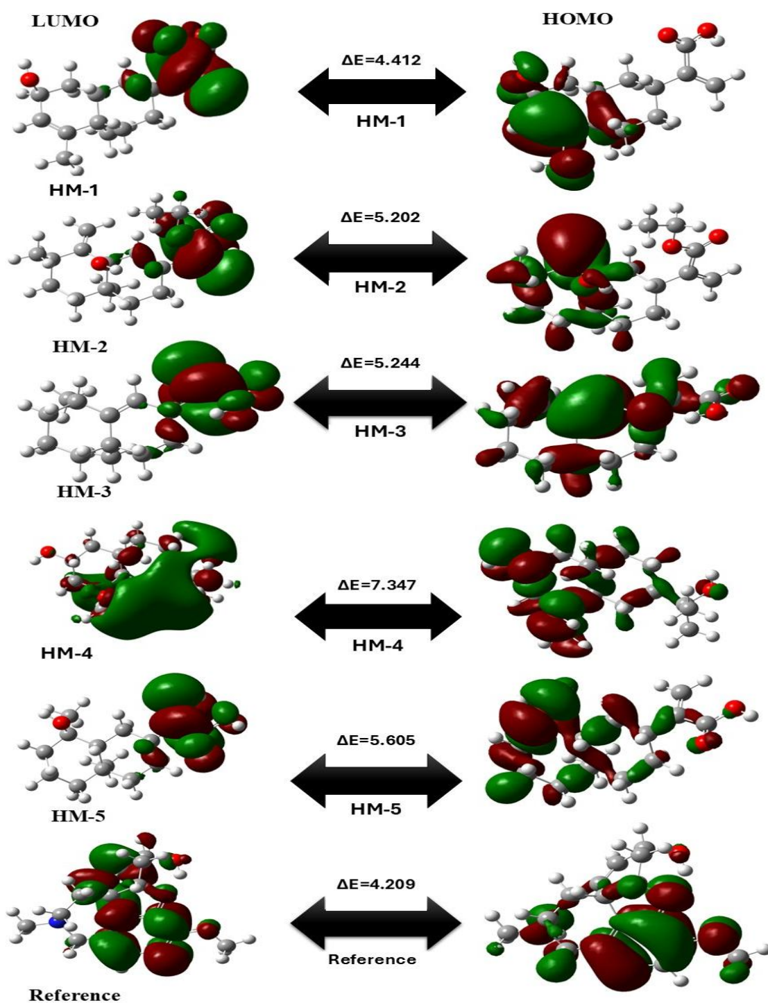
Fig 4 Frontier molecular orbital (HOMO and LUMO) electron density distribution patterns for the reference compound (R) and natural compounds HM-1 to HM-5.
