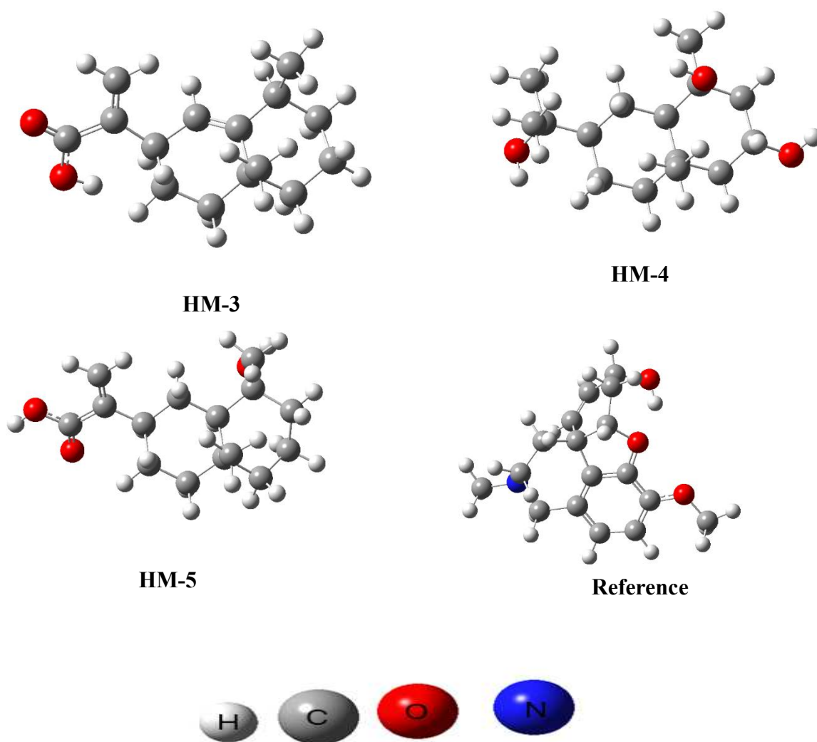
Fig 3 Representation of optimized 3D structure of the reference (R) and natural compounds HM-1 – HM-5.
