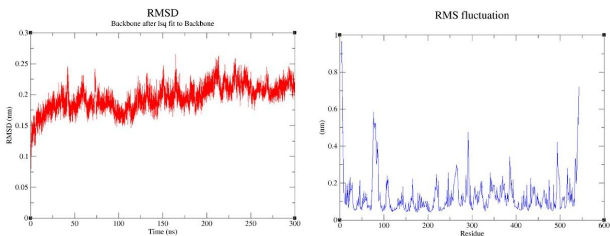
Fig 10: RMSD and RMS plot
