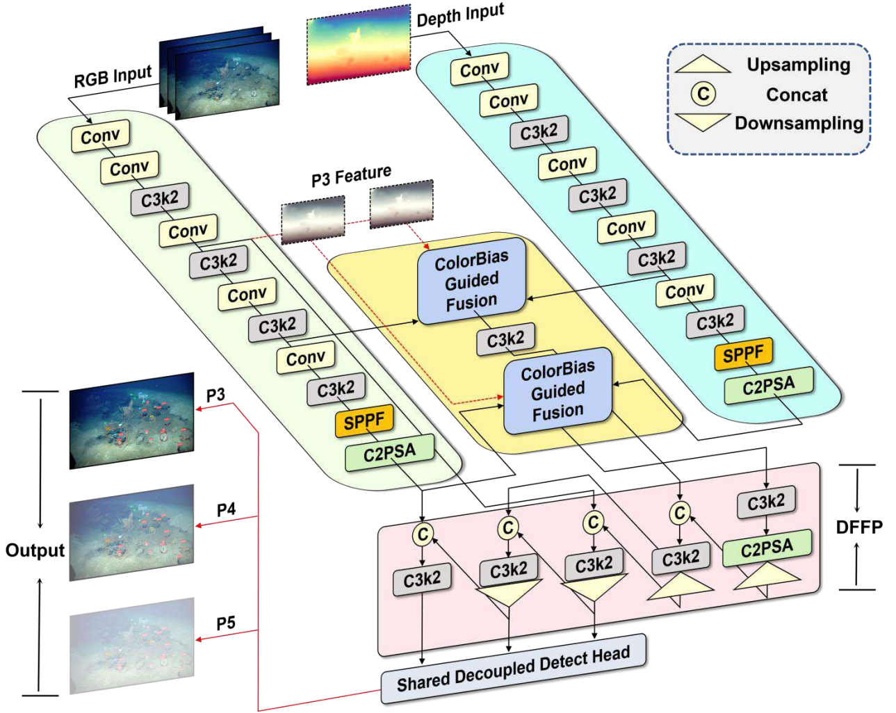
Fig.2. Architecture of the UCH-Net for underwater cultural heritage detection. The framework integrates dual-stream RGB and depth feature extraction, Color-Bias-Guided Fusion for physical-prior-guided multimodal feature integration, and a Shared Decoupled Detect Head for multiscale object prediction.
