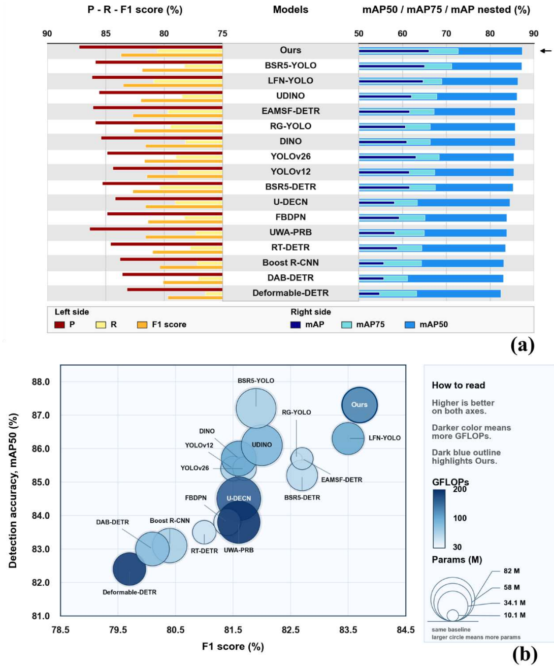
Fig.4. Comparative detection performance and accuracy–efficiency trade-offs of UCH-Net and competing methods on the RUOD dataset. The upper panel (a) compares Precision, Recall, F1-score, mAP50, mAP75 and mAP across the evaluated detectors. The lower panel (b) illustrates the relationship between detection accuracy and model complexity, with bubble size representing the number of parameters and color intensity indicating computational cost in GFLOPs.
