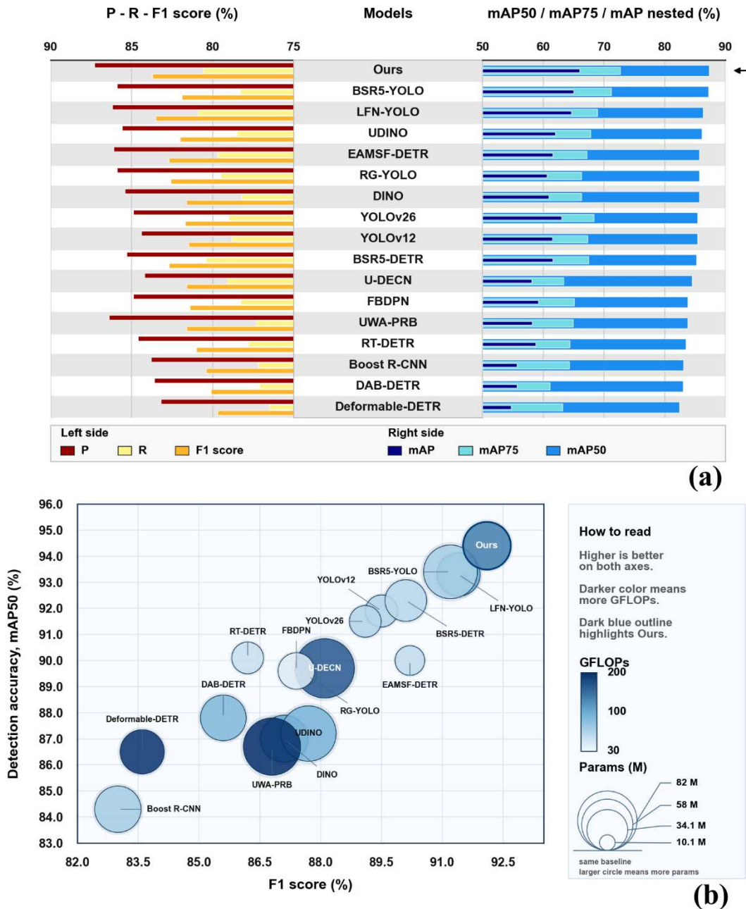
Fig.3. Comparative detection performance and accuracy-efficiency trade-offs of UCH-Net and competing methods on the WRF dataset. The upper panel (a) compares Precision, Recall, F1-score, mAP50, mAP75 and mAP across the evaluated detectors. The lower panel (b) illustrates the relationship between F1-score and detection accuracy, with bubble size representing the number of model parameters and color intensity indicating computational complexity in GFLOPs. The figure provides a comparative overview of detection accuracy and model efficiency across different architectures.
