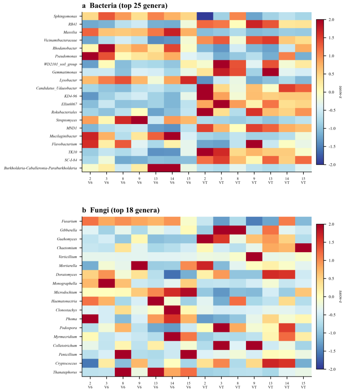
Fig. S3. Genus-level community composition. Heatmap of row z-scored relative abundances for the top 25 bacterial and top 18 fungal genera across cultivar × stage groups (genus names in italics; unclassified taxa labeled at the lowest resolved rank).
