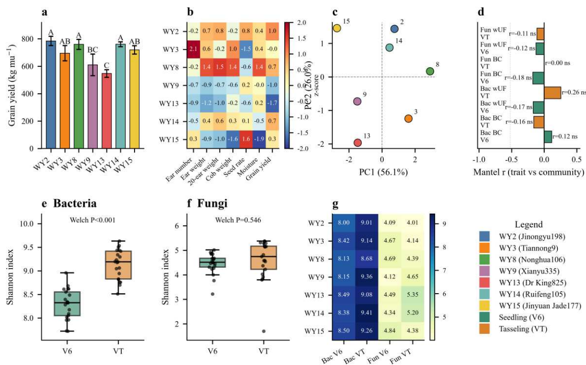
Fig. 2. Phenotypic variation, phenotype–microbiome decoupling, and alpha-diversity. (a) Grain yield of the seven cultivars (mean \pm SE, n = 3 ; uppercase letters denote Tukey HSD groups, P < 0.05 ). (b) Heatmap of z-scored agronomic traits. (c) Principal component analysis of agronomic traits (PC1 = 56.1 %, PC2 = 26.0 %). (d) Genotype-level Mantel tests between agronomic-trait and community distance matrices ( 7 \times 7 mean matrices; 9,999 permutations); no test remained significant after Benjamini–Hochberg correction (dashed line: r = 0 ). (e, f) Bacterial and fungal Shannon diversity by developmental stage (Welch's t-test; NS, not significant). (g) Shannon diversity across cultivar \times stage combinations (mean \pm SEM). V6, seedling stage; VT, tasseling stage.
