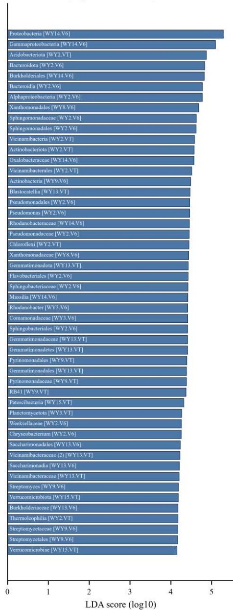
Fig. S4. LEfSe differentially abundant features (LDA > 3.0), top 50 per kingdom. (a) Bacteria (top 50 of 341 significant features). (b) Fungi (top 50 of 172). Bars show LDA scores; group membership is given in brackets (e.g., [WY14;V6]). Numerical suffixes, e.g., "Fungi (3)", distinguish biomarkers reported at multiple taxonomic ranks that resolve to the same display name.
