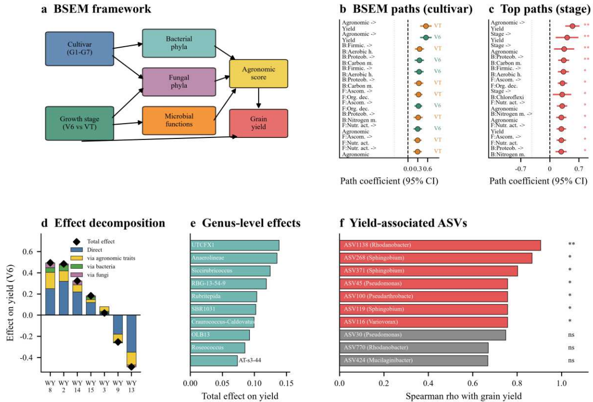
Fig. 6. A Bayesian structural equation framework links microbiome features to measured grain yield. (a) A priori BSEM structure: source variables (cultivar, growth stage) → dominant phyla → predicted functional guilds → agronomic-trait composite → measured yield. (b) Top significant paths of the genotype models (V6 and VT; standardized coefficients with 95 % credible intervals). (c) Top significant paths of the pooled stage model. (d) Cultivar-level decomposition of total microbial effects on yield into direct and indirect components at V6 and VT. (e) Genus-level total-effect decomposition (top 10 genera). (f) Yield-associated ASVs identified by machine-learning signature analysis (Spearman \rho with measured yield; significance stars as in Table S8). Model fit indices and the fraction of yield variance reproduced by each model are reported in Table 4. Grain yield was measured in the field; no forecasting was performed. Significance: * P < 0.05 , ** P < 0.01 , *** P < 0.001 .
