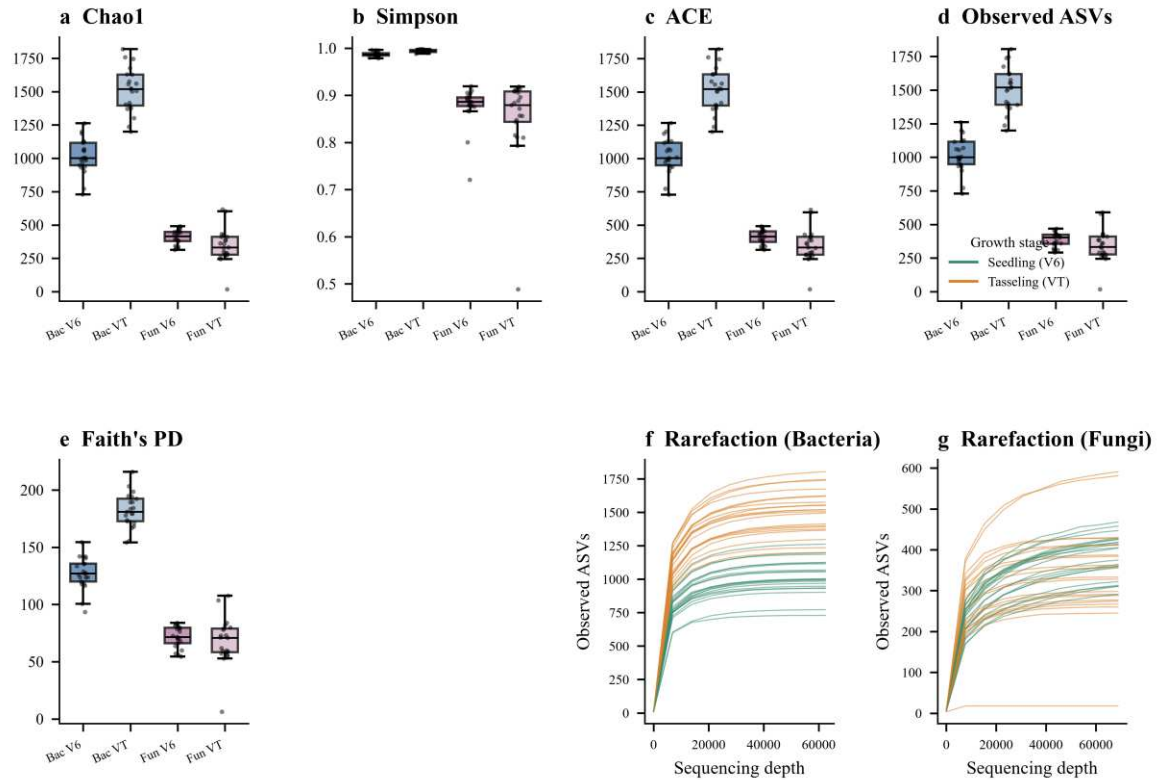
Fig. S2. Alpha-diversity indices and rarefaction. (a–e) Chao1, Simpson, ACE, observed features, and Faith's phylogenetic diversity for bacteria and fungi at V6 and VT (boxplots with per-sample points; Welch's t-test between stages). (f, g) Rarefaction curves of observed features for bacteria and fungi (mean per cultivar \times stage group; legend in panel d). Bacterial indices increased strongly at VT; fungal indices showed no significant stage difference.
