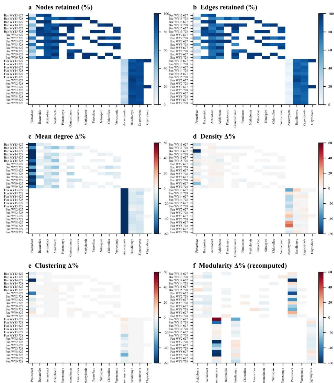
Fig. S7. Network robustness across six metrics after phylum-level removal. (a–e) Percentage of nodes retained, edges retained, and percentage changes in average degree, density, and clustering coefficient across all 28 networks. (f) Percentage change in modularity recomputed de novo from edge tables (only removals of phyla with \geq 3 nodes shown).
