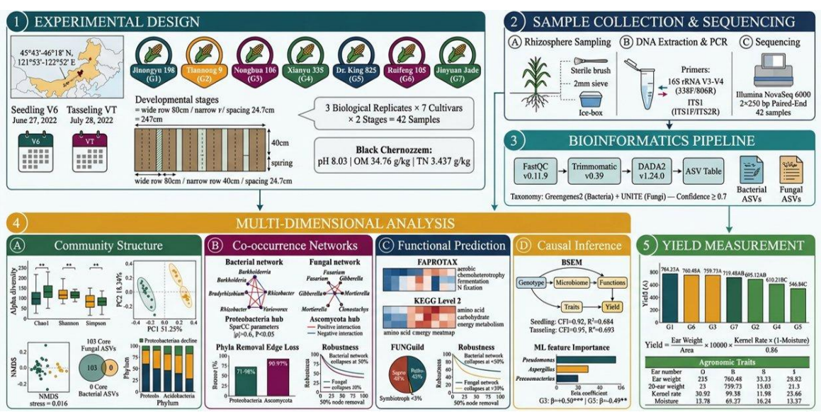
Fig. 1. Experimental design and integrative analytical framework. Seven maize cultivars were grown in a replicated field trial and rhizosphere-sampled at the seedling (V6) and tasseling (VT) stages (42 samples); bacterial (16S rRNA) and fungal (ITS) communities were profiled in parallel and integrated through diversity analyses, co-occurrence networks with robustness validation, functional annotation, Bayesian structural equation modeling (BSEM), and machine-learning-based signature identification. G1–G7 denote BSEM cultivar codes.
