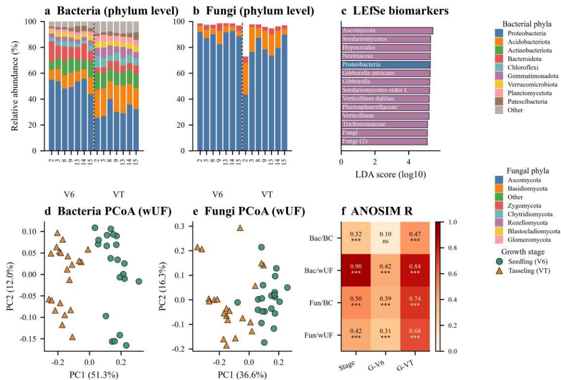
Fig. 3. Community composition and beta-diversity. (a, b) Phylum-level relative abundance of bacterial and fungal communities across cultivars and stages (top 10 phyla plus remainder). (c) LefSe biomarkers (top 14 by LDA score; group membership in brackets). (d, e) Principal coordinate analysis on weighted UniFrac distances for bacteria (PC1 = 51.25 %, PC2 = 11.98 %) and fungi (PC1 = 36.64 %, PC2 = 16.33 %). (f) ANOSIM R values for the factors stage (all samples) and genotype (within each
