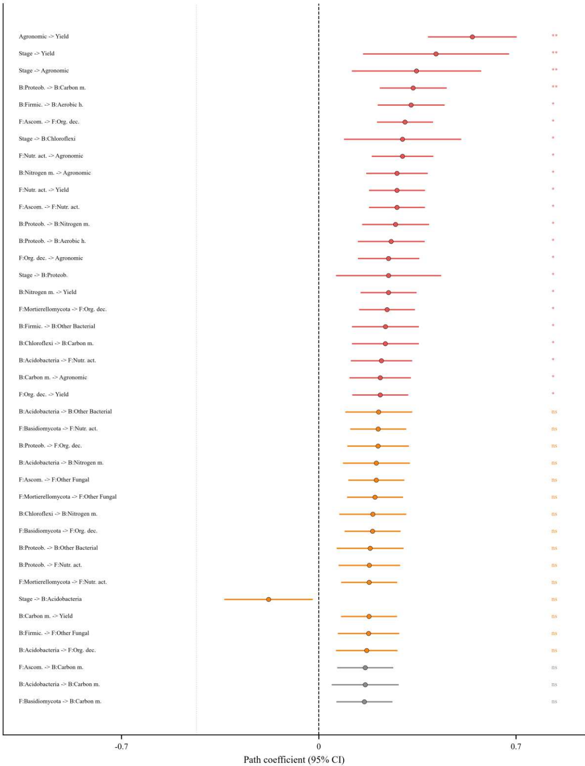
Standardized paths of the growth-stage BSEM (top 40 by |\beta| ; red P < 0.05 , orange P < 0.1 )
