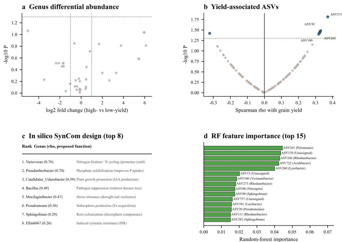
Fig. S10. Machine-learning signature identification (no forecasting performed). (a) Volcano plot of genus-level differential abundance between high- and low-yield cultivar groups; no genus passed the significance thresholds (dashed lines: P = 0.05 , |\log_2 \text{fold change}| = 1 ), a genuine null result. (b) Yield-associated ASVs (Spearman \rho with measured yield versus -\log_{10} P ); the four strongest correlates are labeled. (c) In silico SynCom candidate design (top eight genera by positive yield association, with proposed functions; hypothesis-generating only). (d) Random-forest feature importance (top 15 ASVs; in-sample ranking).
