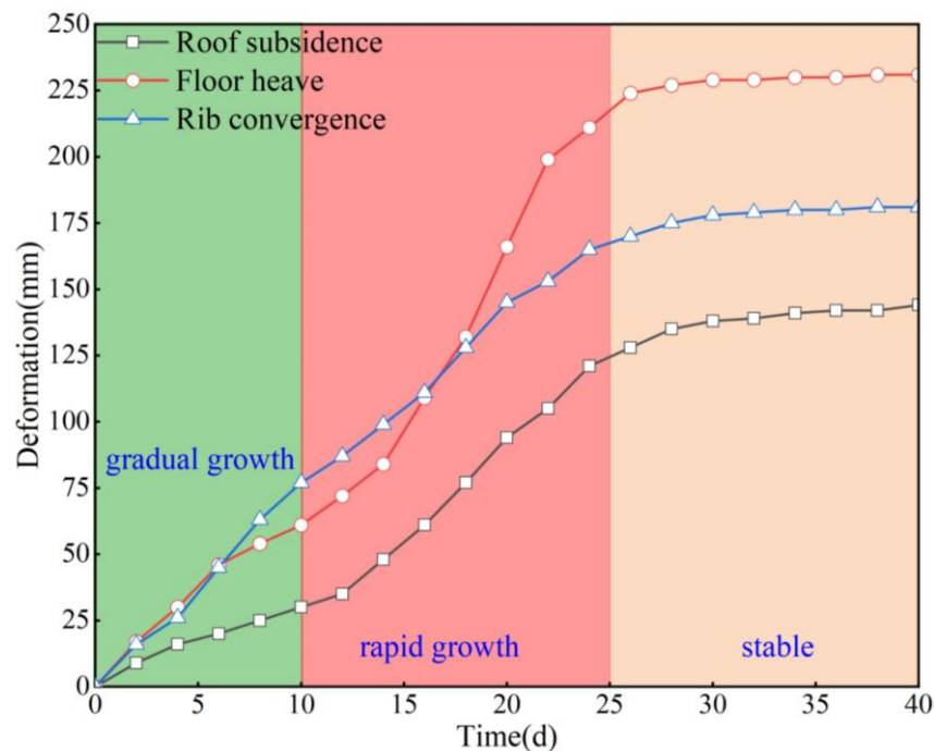
Fig. 21. Deformation of the roadway surrounding rock after pressure relief.
