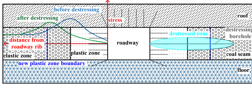
Fig. 6. Principle of borehole pressure relief.
