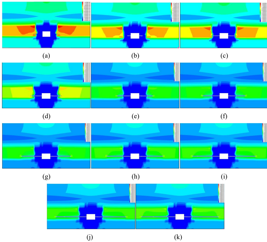
Fig. 18. Elastic strain energy density contours in the roadway ribs for different borehole depths: (a) no borehole; (b) 2 m; (c) 4 m; (d) 6 m; (e) 8 m; (f) 10 m; (g) 12 m; (h) 14 m; (i) 16 m; (j) 18 m; (k) 20 m.
