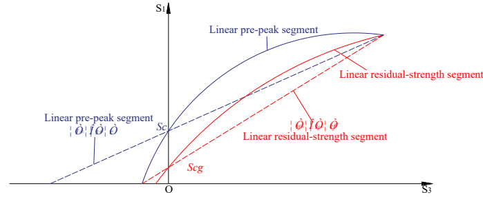
Fig. 7. Peak and residual strength curves of coal.
