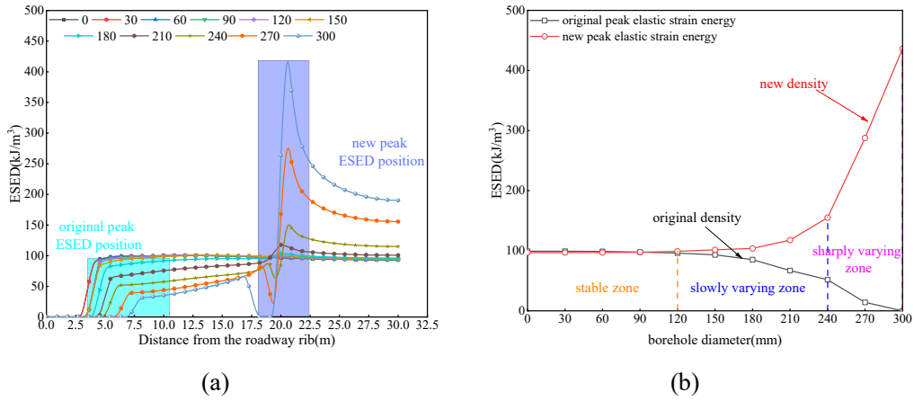
Fig. 17. Relationship between borehole diameter and elastic strain energy density: (a) energy density profiles in the roadway rib; (b) peak energy density values.
