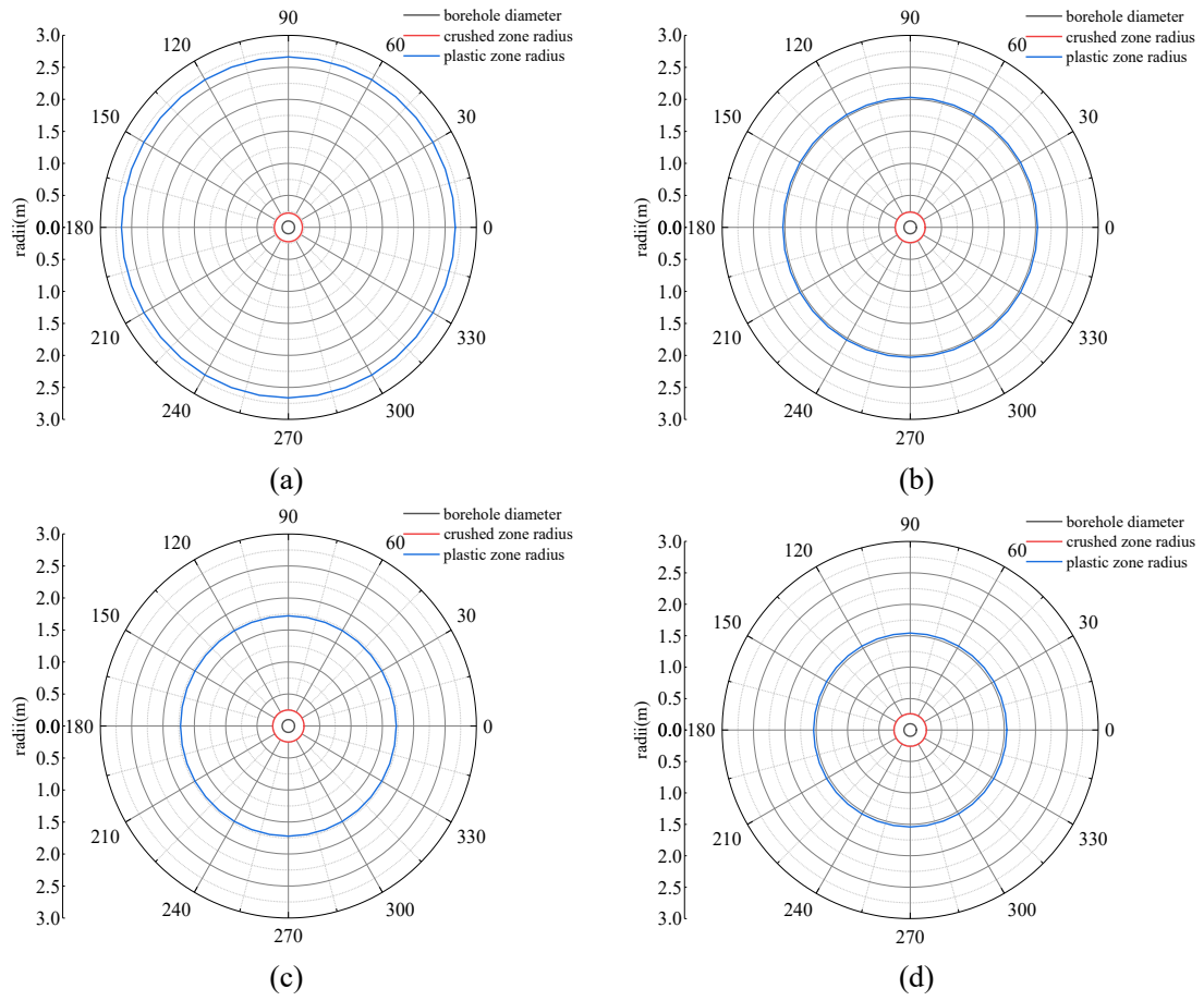
Fig. 11. Pressure relief zones for different cohesion values: (a) c = 2.0 MPa; (b) c = 2.5 MPa; (c) c = 3.0 MPa; (d) c = 3.5 MPa.
