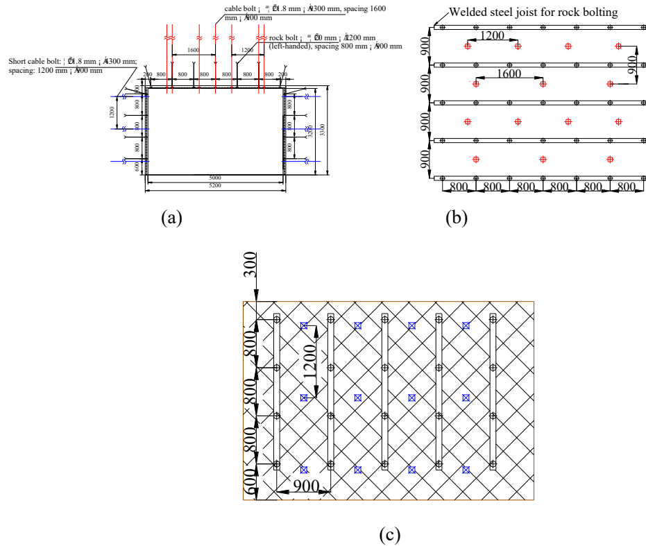
Fig. 3. Original support layout for the 50502 haulage roadway: (a) cross section; (b) roof layout; (c) rib layout.
