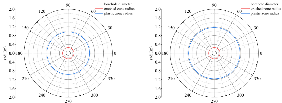
Fig. 9. Pressure relief zones for different borehole diameters: (a) 100 mm; (b) 200 mm; (c) 300 mm; (d) 400 mm.
