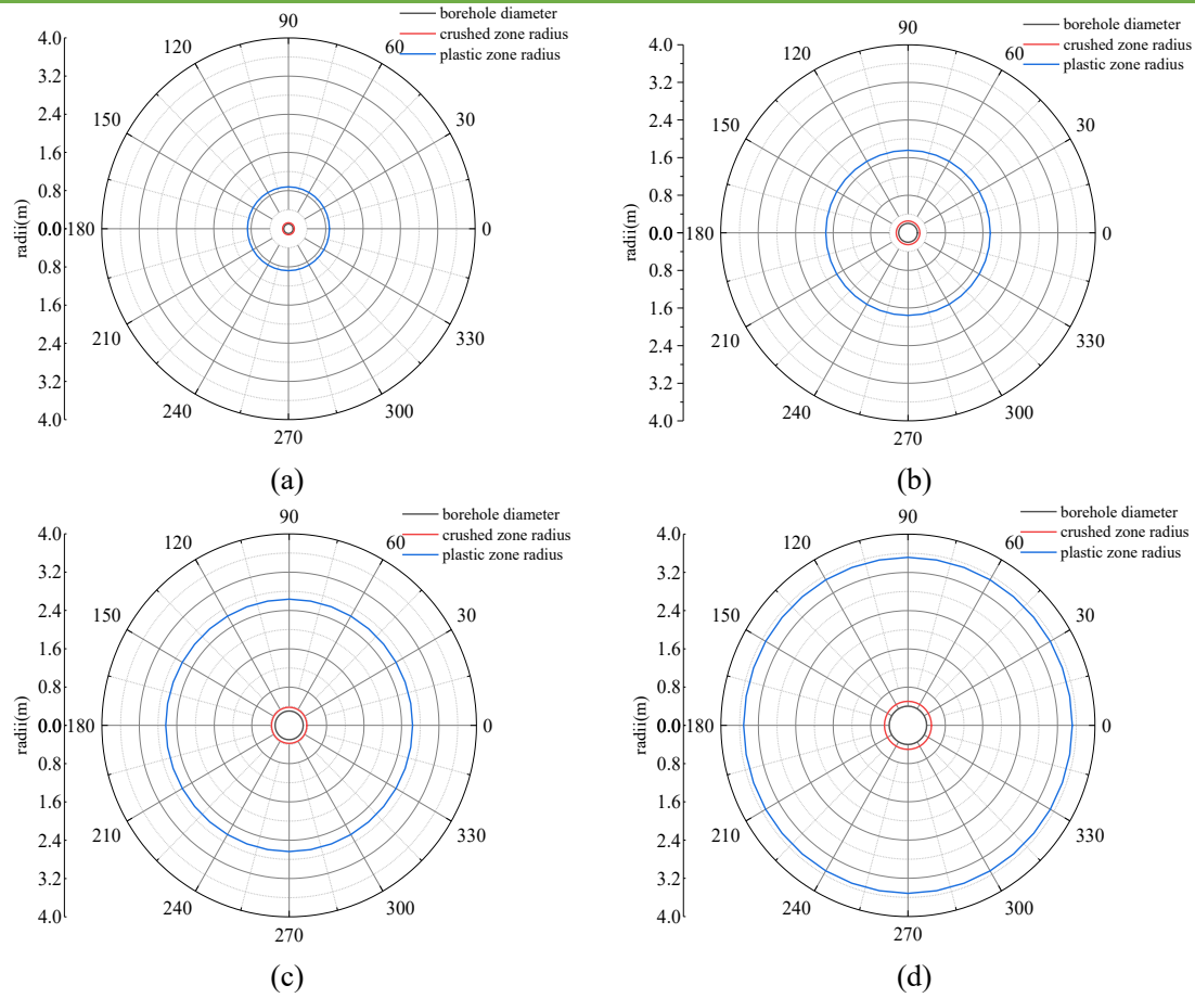
Fig. 9. Pressure relief zones for different borehole diameters: (a) 100 mm; (b) 200 mm; (c) 300 mm; (d) 400 mm.
