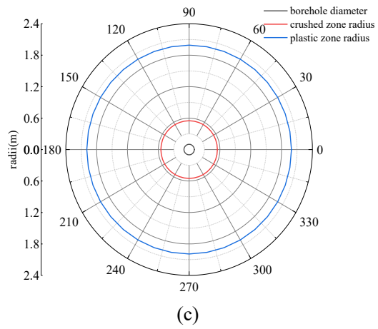
Fig. 13. Pressure relief zones for different lateral stress coefficients: (a) \lambda = 0.6 ; (b) \lambda = 1.0 ; (c) \lambda = 1.4 ; (d) \lambda = 1.8 .
