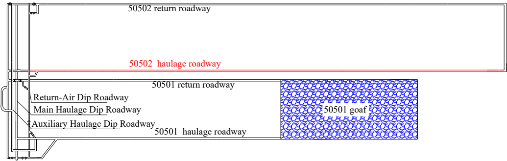
Fig. 1. Plan view of the 50502 working face.
