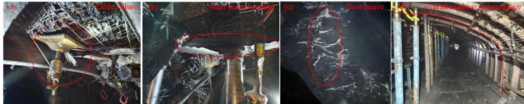
Fig. 5. Roadway failure characteristics.
