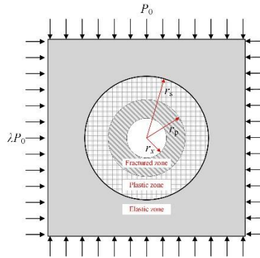
Fig. 8. Zonation of the surrounding rock around a pressure relief borehole.
