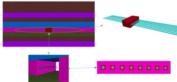
Fig. 15. Numerical model of borehole pressure relief.
