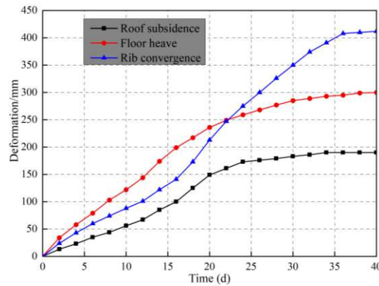
Fig. 4. Deformation curves of the roadway surrounding rock.
