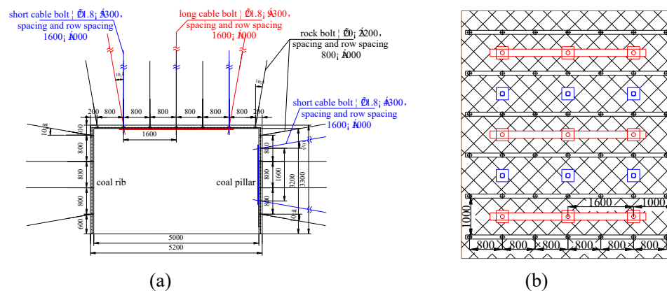
Fig. 20. Support layout for the 50502 haulage roadway: (a) cross section; (b) roof support layout.
