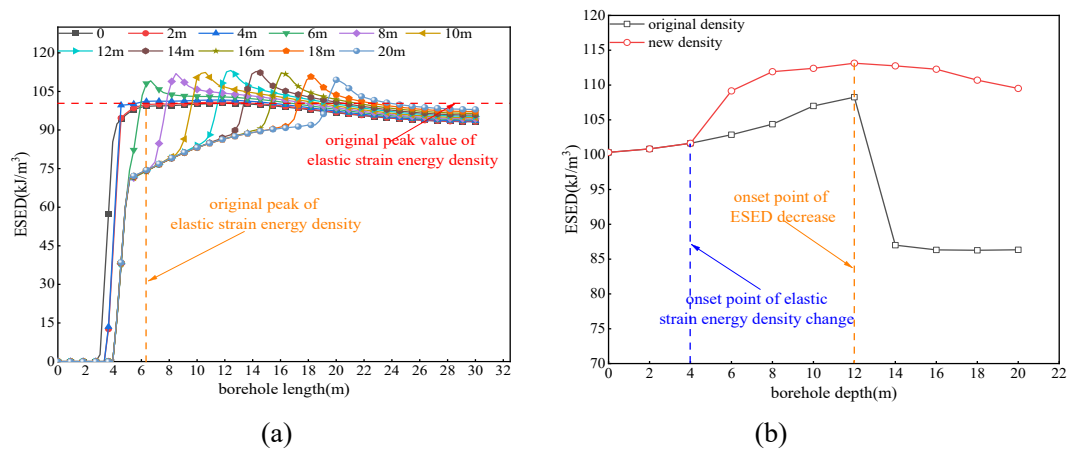
Fig. 19. Elastic strain energy density in the roadway ribs for different borehole depths: (a) energy density profiles; (b) peak values.
