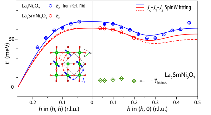
FIG. 3. Dispersion and intrinsic damping of spin excitations in \text{La}_2\text{SmNi}_2\text{O}_7 . Red open circles show the undamped mode energies E_{0,q} of \text{La}_2\text{SmNi}_2\text{O}_7 extracted from resolution-convolved DHO fits to the RIXS spectra, with a representative fit shown in Fig. 2(c). Green open diamonds show the intrinsic damping parameters \gamma_q obtained from the same convolved fits. For each \text{La}_2\text{SmNi}_2\text{O}_7 spectrum, the resolution function was determined from a Pearson-VII fit to the elastic line. For comparison, blue open circles show the corresponding E_{0,q} values of \text{La}_3\text{Ni}_2\text{O}_7 , obtained by reanalyzing the source spectra of Ref. [16] with a 36.5-meV-FWHM Gaussian resolution function. The blue solid curve is a bilayer J_c - J_1 - J_2 SpinW fit to the \text{La}_3\text{Ni}_2\text{O}_7 dispersion. The red solid and dashed curves show, respectively, the common-scale fit with s = 0.90 and the free-parameter fit to the five \text{La}_2\text{SmNi}_2\text{O}_7 data points. The inset illustrates the assumed single-stripe spin configuration and defines the exchange-parameter convention. The vertical gray line marks the \Gamma point. Error bars denote formal standard errors from the spectral fits.
