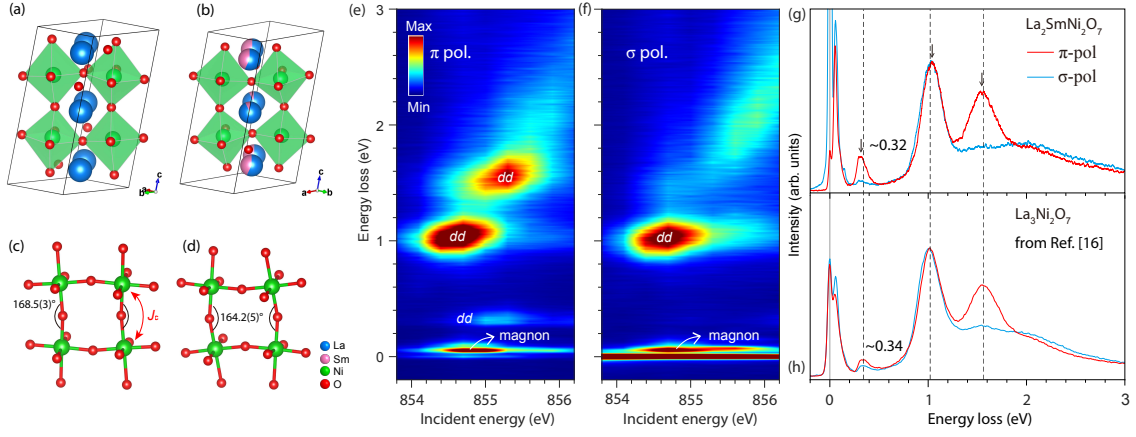
FIG. 1. Local structure and Ni- L_3 RIXS spectra of \text{La}_2\text{SmNi}_2\text{O}_7 . (a),(b) Crystal structures of monoclinic \text{La}_3\text{Ni}_2\text{O}_7 and \text{La}_2\text{SmNi}_2\text{O}_7 ( P2_1/m ), respectively. (c),(d) Ball-and-stick representations of the corner-shared \text{NiO}_6 bilayers, with the interlayer Ni-O AP -Ni bond angles reported in Ref. [7] indicated. (e),(f) Incident-energy-dependent Ni- L_3 -edge RIXS intensity maps of \text{La}_2\text{SmNi}_2\text{O}_7 measured with \pi - and \sigma -polarized incident light, respectively. The measurements were performed at T = 20 K with a scattering angle 2\theta = 90^\circ and an incident angle \theta = 20^\circ . (g) Corresponding incident-energy-integrated spectra of \text{La}_2\text{SmNi}_2\text{O}_7 obtained from (e),(f) over the incident-energy range 853.8–856.2 eV. (h) Incident-energy-integrated Ni- L_3 RIXS spectra of \text{La}_3\text{Ni}_2\text{O}_7 , reproduced from Ref. [16]. Black dashed lines mark the peak energies of the electronic excitations in \text{La}_3\text{Ni}_2\text{O}_7 , while black arrows indicate the corresponding peak positions in \text{La}_2\text{SmNi}_2\text{O}_7 . The spectra show closely comparable local electronic excitations in the two compounds, with the lowest-energy feature shifting only modestly from \sim 0.34 eV in \text{La}_3\text{Ni}_2\text{O}_7 to \sim 0.32 eV in \text{La}_2\text{SmNi}_2\text{O}_7 .
