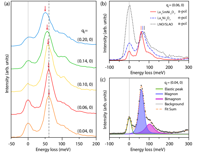
FIG. 2. Well-defined dispersive spin excitations in \text{La}_2\text{SmNi}_2\text{O}_7 . (a) Waterfall plot of Ni- L_3 -edge RIXS spectra measured along the [H, 0] direction using \pi -polarized incident photons with E_i = 854.65 eV at T = 20 K. Well-defined dispersive magnetic excitations are observed. Red arrows mark the peak positions of the spin excitations. (b) Comparison of spin-excitation spectra at q_{||} = (0.06, 0) , close to the band top near the zone center, for \text{La}_2\text{SmNi}_2\text{O}_7 , bulk \text{La}_3\text{Ni}_2\text{O}_7 , and \text{La}_3\text{Ni}_2\text{O}_7/\text{SrLaAlO}_4 . Short vertical ticks indicate the fitted magnon peak positions. The data for \text{La}_3\text{Ni}_2\text{O}_7 and \text{La}_3\text{Ni}_2\text{O}_7/\text{SrLaAlO}_4 are reproduced from Refs. [16, 40]. (c) Representative resolution-convolved DHO fit to the RIXS spectrum of \text{La}_2\text{SmNi}_2\text{O}_7 at q_{||} = (0.04, 0) . For this spectrum, the experimental resolution function was determined from the fitted elastic line, giving an energy-resolution FWHM of \Delta E \approx 20 meV. The shaded components denote elastic scattering, one-magnon and bimagnon excitations, together with an empirical high-energy background. The dashed curve represents the total fit.
