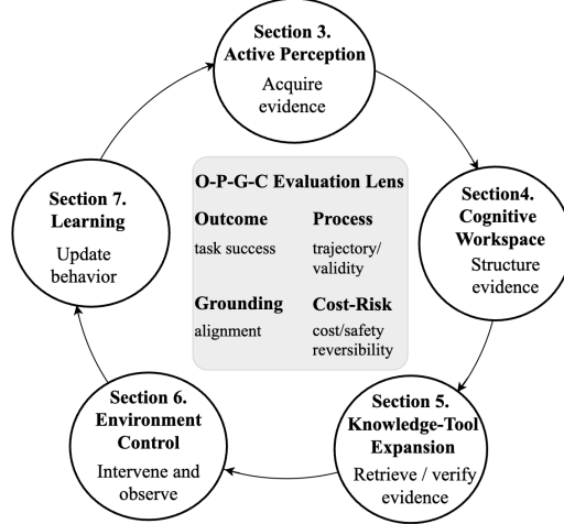
Fig. 1 Closed-loop evidence framework for multimodal agency. The five evidence loops organize Sections 3–7, while the O-P-G-C lens summarizes the evaluation dimensions discussed in Section 8
