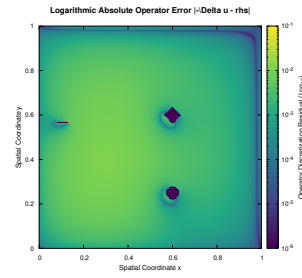
(b) Absolute discretization error |\Delta u - \text{rhs}| .
