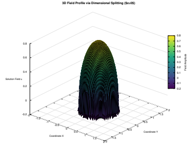
(a) 3D Obstacle Problem a snapshot splitting method
