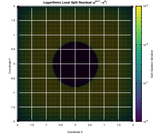
(b) 3D Obstacle Problem error a snapshot splitting method
