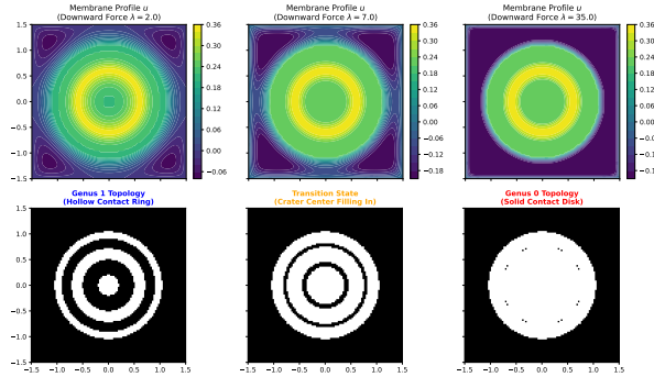
Figure 3: Numerical test of the topological change under increasing downward force \lambda . Top row of plots : continuous solution of membrane displacement profiles u . Bottom row of plots : characteristic function of the active contact zone \Omega_\Lambda = \{x \in \Omega : |u(x) - \psi(x)| < 5 \times 10^{-3}\} where variation \lambda = 2.0, 7.0, 35.0 , the topology smoothly changes from a doubly connected ring (genus 1) to a simply connected solid disk (genus 0).
