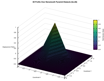
(c) 3D Obstacle Problem a snapshot splitting method nonsmooth case
