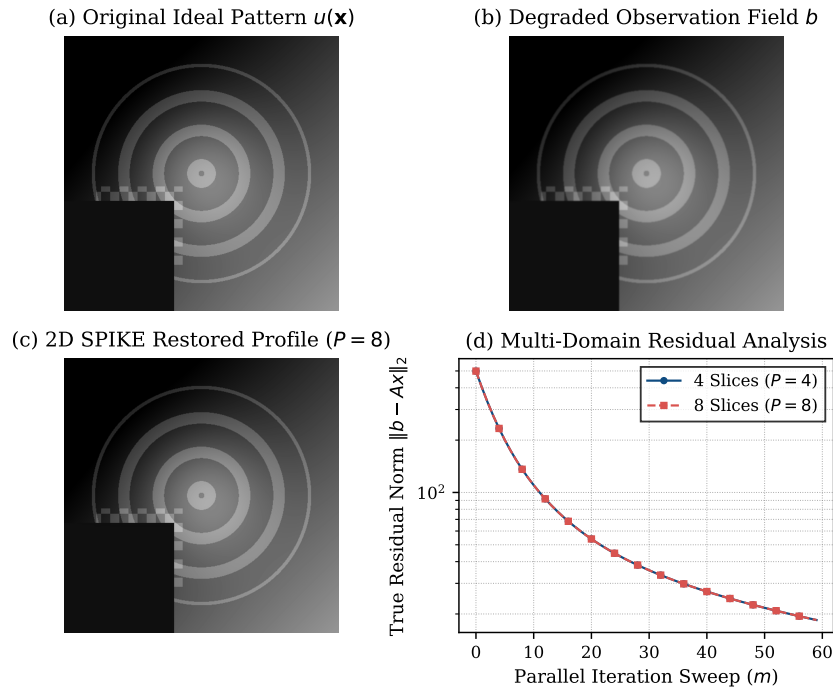
Figure 8: Image deblurring problem
