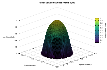
(a) Numerical solution surface u(x, y) .
