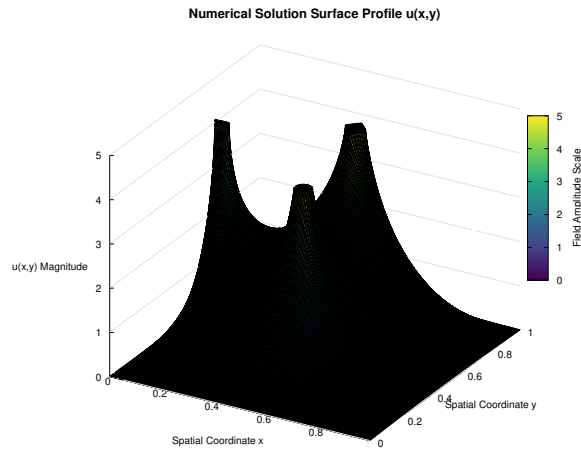
(a) Numerical solution surface u(x, y) .
