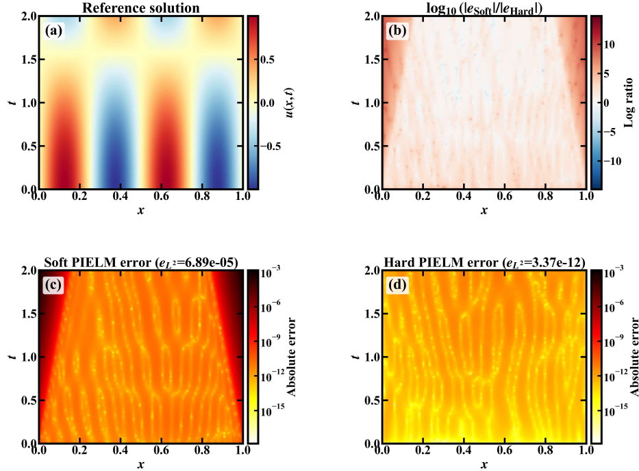
Figure 9: Wave 1D benchmark ( N = 3000 , N_{\text{int}} = 10,000 ). (a) Reference solution on [0, 1] \times [0, 2] . (b) Log-ratio map. (c,d) Pointwise absolute errors on a common logarithmic color scale.
