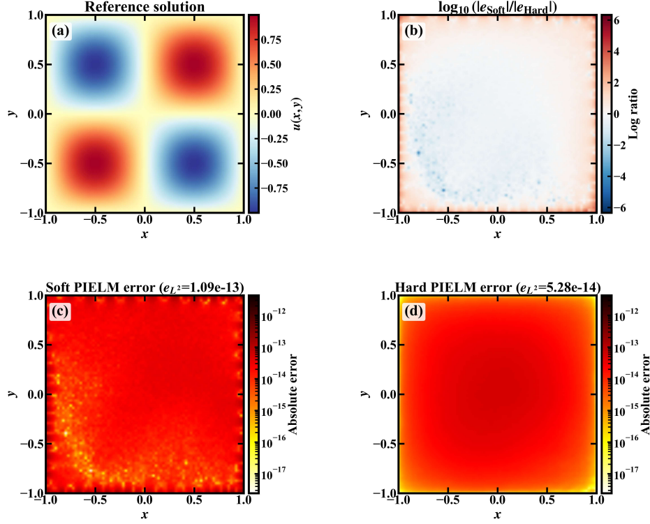
Figure 3: Poisson 2D benchmark ( N = 2000 , N_{\text{int}} = 10,000 ). (a) Reference solution. (b) Log-ratio map \log_{10}(|e_{\text{Soft}}|/|e_{\text{Hard}}|) . (c,d) Pointwise absolute errors on a common logarithmic color scale.
