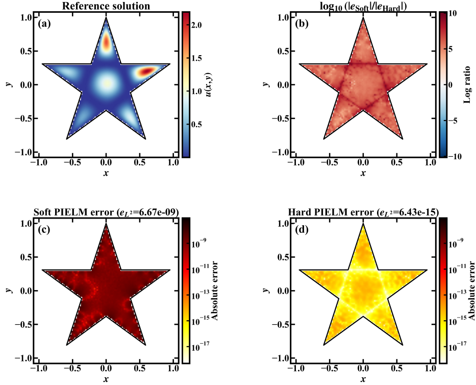
Figure 11: Pentagram nonlinear reaction benchmark ( N = 3000 , N_{\text{int}} = 10,000 , 30 Picard iterations). (a) Reference solution on the pentagram domain. (b) Log-ratio map. (c,d) Pointwise absolute errors on a common logarithmic color scale.
