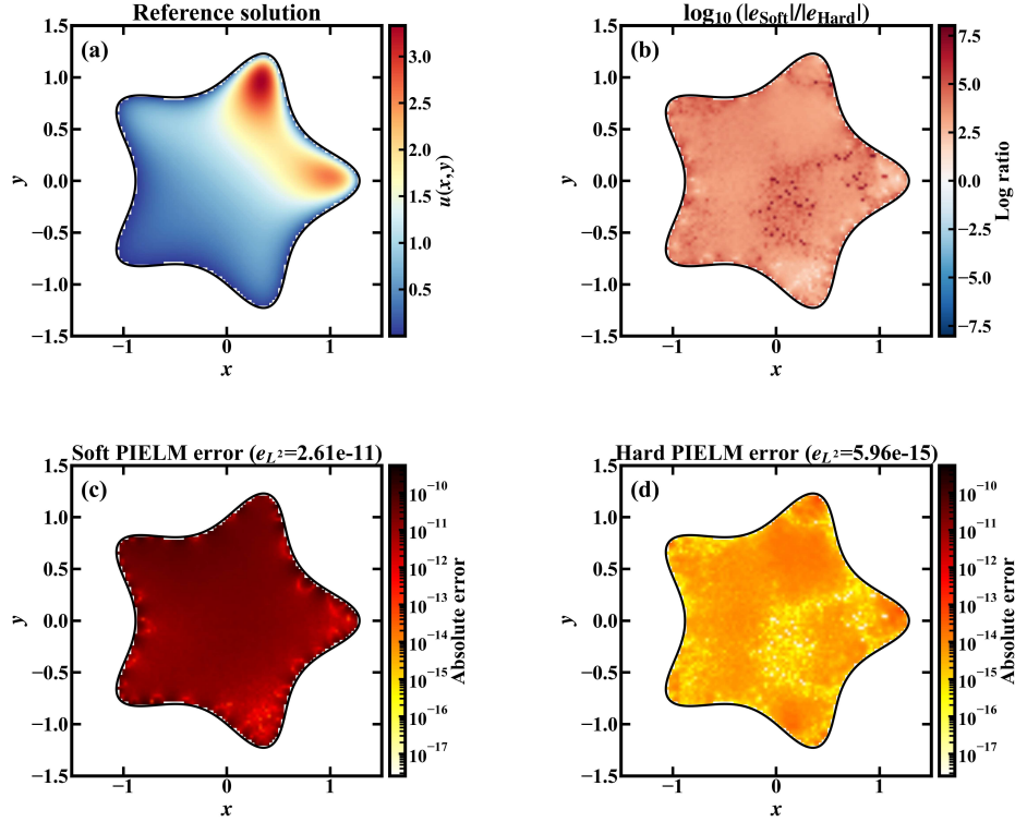
Figure 13: Flower domain nonlinear reaction benchmark ( N = 2000 , N_{\text{int}} = 10,000 , 30 Picard iterations). (a) Reference solution on the five-petal flower domain. (b) Log-ratio map. (c,d) Pointwise absolute errors on a common logarithmic color scale.
