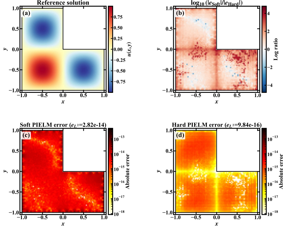
Figure 5: L-shape Poisson benchmark ( N = 3000 , N_{\text{int}} = 10,000 ). (a) Reference solution on [-1, 1]^2 \setminus [0, 1]^2 . (b) Log-ratio map. (c,d) Pointwise absolute errors on a common logarithmic color scale.
