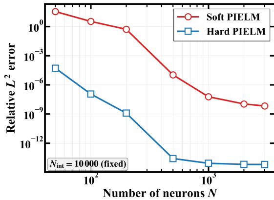
(a) Neuron sweep: relative L^2 error vs. N at fixed N_{\text{int}} = 10,000 .
