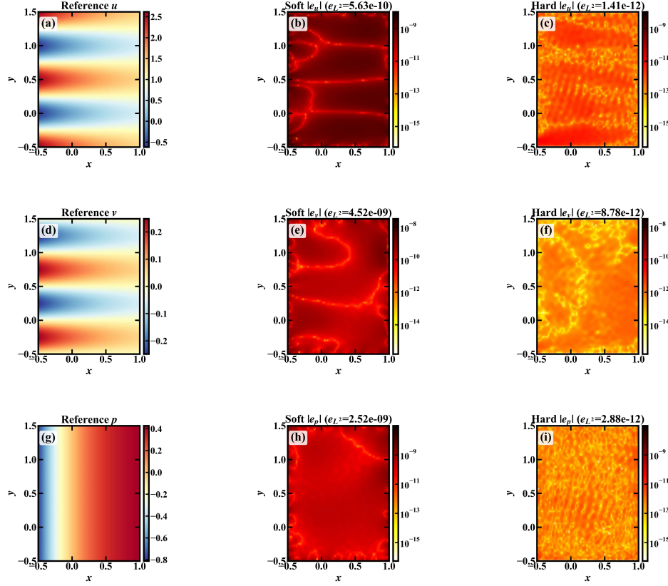
Figure 7: Navier–Stokes Kovaszny flow ( N = 1500 , N_{\text{int}} = 8192 , 40 Picard iterations). Rows show u , v , and p ; columns show the reference solution, Soft error, and Hard error. Error maps use a common logarithmic scale within each row.
