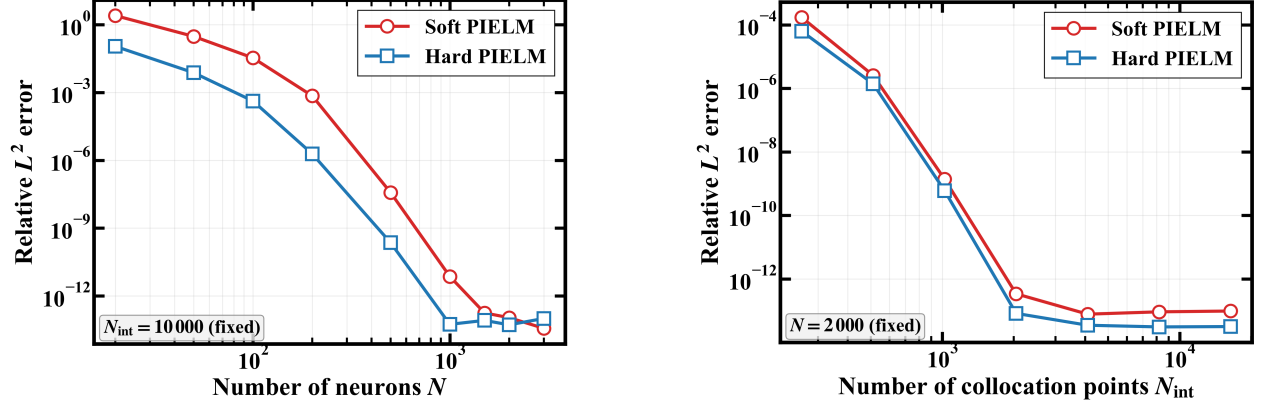
(a) Neuron sweep: relative L^2 error vs. N at fixed N_{\text{int}} = 10,000 .
