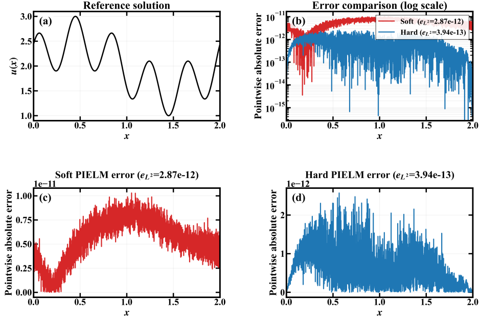
Figure 1: Helmholtz 1D benchmark ( N = 1000 , N_{\text{int}} = 10,000 ). (a) Reference solution. (b) Log-scale pointwise error comparison. (c,d) Soft and Hard pointwise errors on a linear scale.
