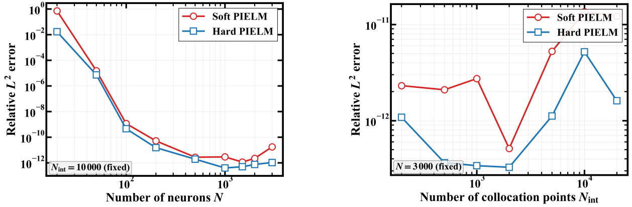
(a) Neuron sweep: relative L^2 error vs. number of neurons N at fixed N_{\text{int}} = 10,000 .
