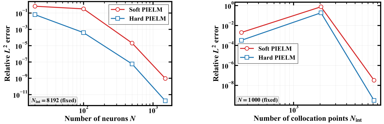
(a) Neuron sweep: combined relative L^2 error vs. N at fixed N_{\text{int}} = 8192 .
