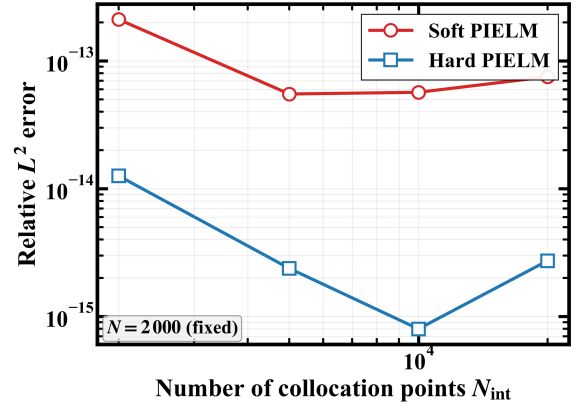
(b) Collocation sweep: relative L^2 error vs. N_{\text{int}} at fixed N = 2000 .
