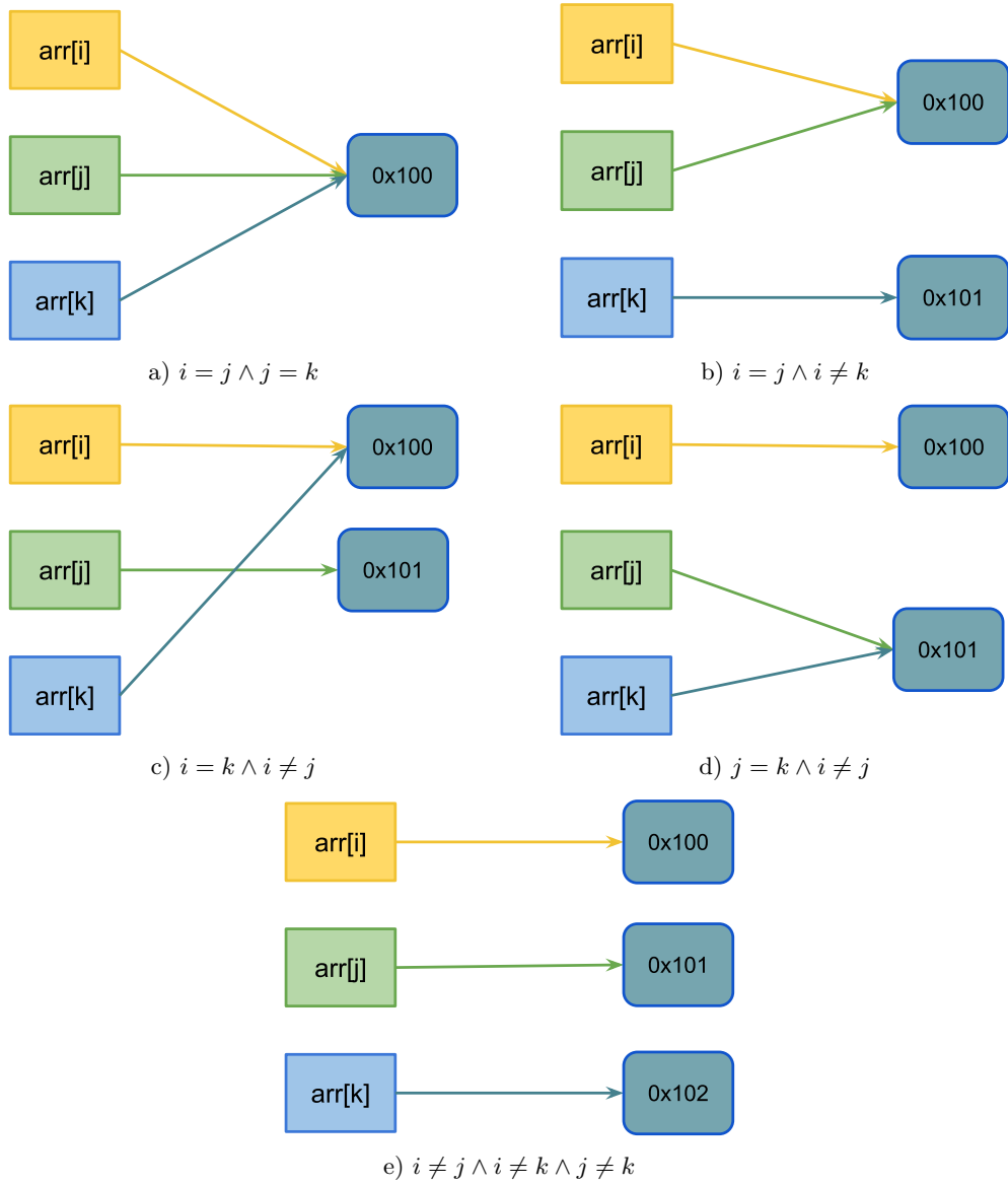
Fig. 7 Possible aliasing configurations for the three symbolic array accesses in Figure 6
