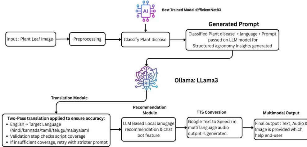
Fig. 4: Image-agentic inference workflow integrating visual classification, interpretability, and multilingual recommendation generation.
