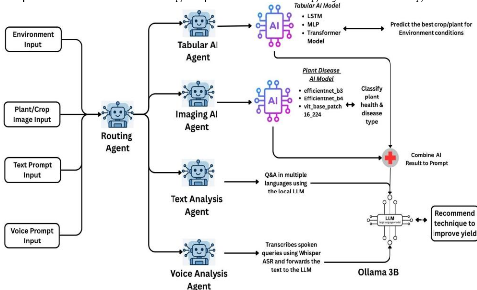
Fig. 2: Overall multi-agent training and orchestration framework. Multimodal inputs are processed through specialized agents for tabular modeling, visual disease classification, interpretability, and LLM-based reasoning
