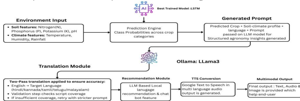
Fig. 3: Tabular and text-agentic inference workflow integrating crop prediction, multilingual reasoning, and speech synthesis.
