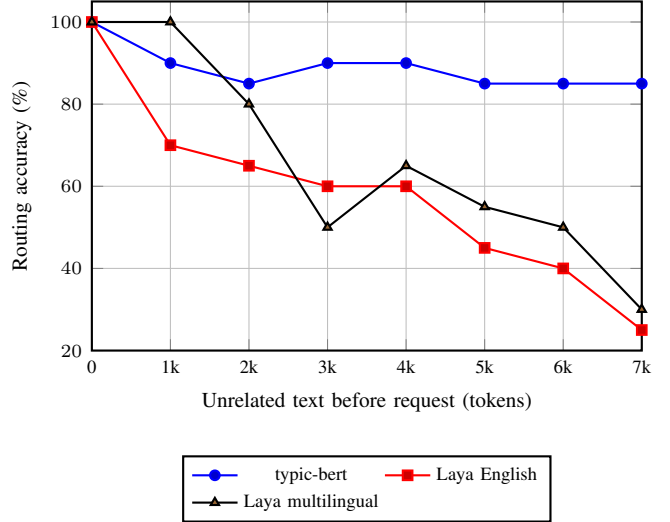
Fig. 1. Routing accuracy as unrelated text is added before the request. Each point contains 20 English requests; all models use a maximum length of 8,192 tokens.
