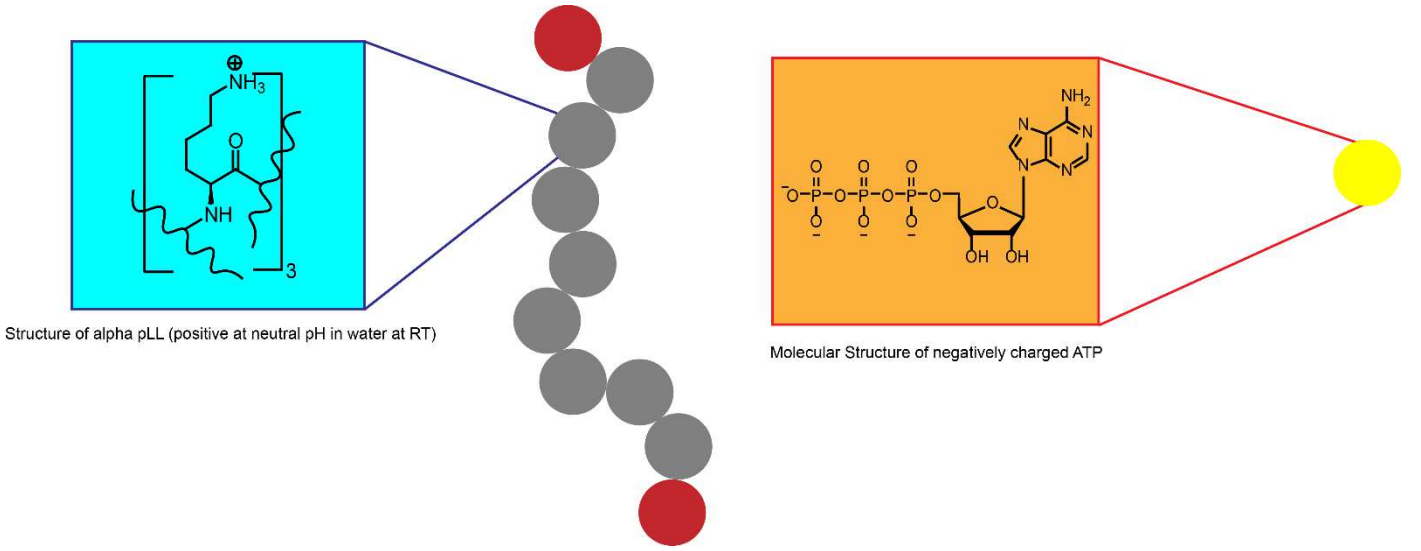
Figure 1. Schematic Representation of the (left) coarse-grained 10 beads alpha poly-L-Lysine (pLL) model and (right) single bead Adenosine Triphosphate (ATP) chosen for the MC simulation. Each bead corresponds to three monomers of L-Lysine having three positive charges at neutral pH and room temperature. The terminal beads are coloured differently for visual clarity. The ATP bead contains the relevant number of negative charges.
