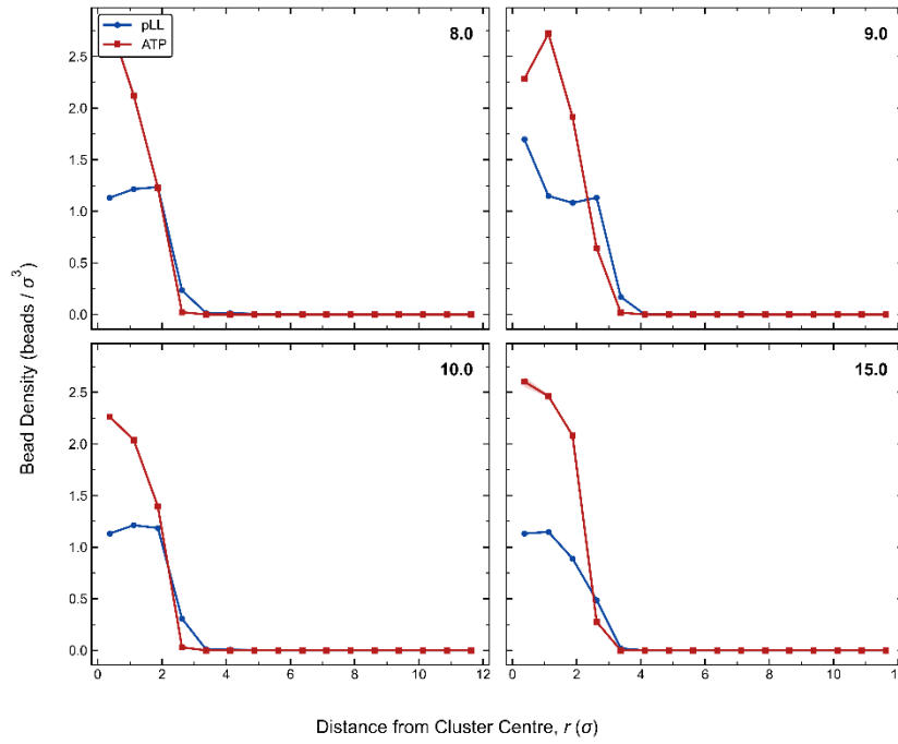
Figure 7. Radial distributions of the key parameters dictating the coacervate structure. (a) Variation of net charge as a function of the radial distance (starting from the cluster centre). (b) Distribution of bead densities of pLL and ATP as a function of radial distances.
