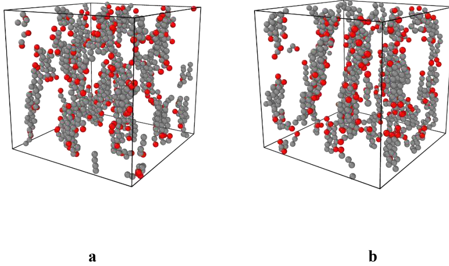
Figure 4. Simulation results of the 100-molecule model pLL system with and without hydrophobic attraction ( \epsilon_{\text{att}} ) at fixed T^* = 0.5 and \text{frac} = 0.08 . a) \epsilon_{\text{att}} = 0.15 , b) \epsilon_{\text{att}} = 0.0 .
