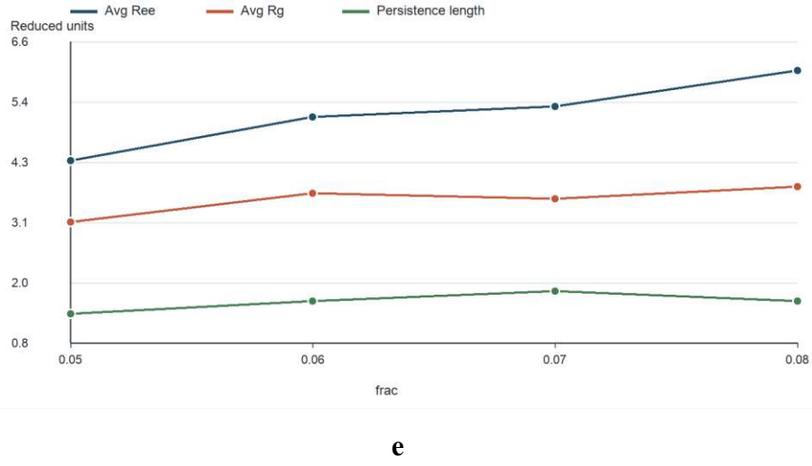
Figure 3. Simulation results of the 100-molecule model pLL system corresponding to different monomer charges ( frac ) at fixed T^* = 0.5 and hydrophobically induced attraction ( \epsilon_{att} = 0.15 ). a) frac = 0.05 , b) frac = 0.06 , c) frac = 0.07 , d) frac = 0.08 . e) Variation of average end to end length ( \langle R_{ee} \rangle ), average radius of gyration ( \langle R_g \rangle ) and persistence length ( L_p ), all in reduced units, with frac .
