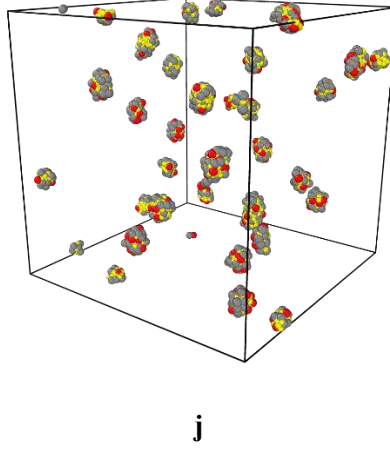
Figure 5. Simulation results from 2 million runs of the 100-molecule model pLL system corresponding to different numbers of ATP molecules/pLL molecule (ATP/pLL number ratios) at fixed T^* = 0.5 and effective charge frac = 1.0 , a) 2, b) 3, c) 4, d) 5, e) 6, f) 7, g) 8, h) 9, i) 10, and j) 15. The ATP molecules are represented by single yellow beads while the pLL molecules are represented by grey beads with red beads at the termini (Figure 1).
