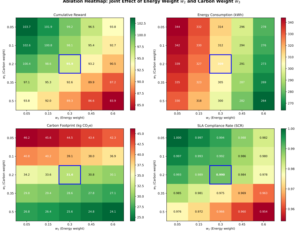
Fig. 6 Reward-Weight Sensitivity Heatmap: w_2 vs w_3 (at Episode 100).
