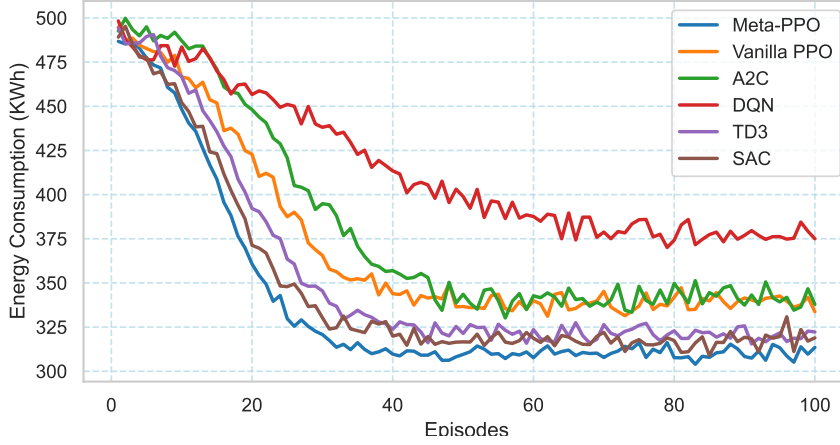
Fig. 3 Energy consumption comparison of different DRL-based methods ( Meta-PPO, Vanilla PPO, A2C, DQN, TD3 and SAC).
