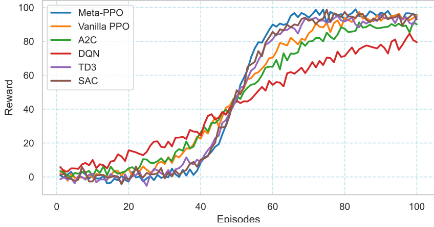
Fig. 2 Reward convergence of different DRL-based methods ( Meta-PPO, Vanilla PPO, A2C, DQN, TD3 and SAC) over training iterations.
