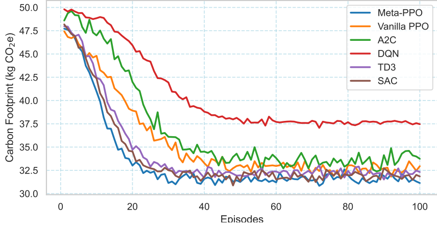
Fig. 4 Carbon Footprint comparison of Meta-PPO, Vanilla PPO, A2C,DQN,TD3 and SAC cumulated in a monthly time-frame.
