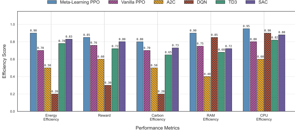
Fig. 8 Comparison of different DRL algorithms based on Energy Efficiency, CPU Efficiency, RAM Efficiency, Reward, and Carbon Efficiency.
