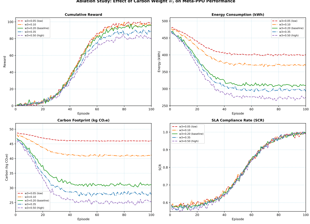
Fig. 7 Ablation and Reward-Sensitivity Analysis: Effect of Carbon Footprint Weight w_3 .
