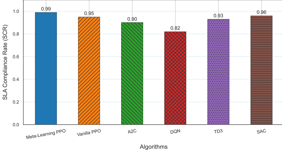
Fig. 5 Comparison of SLA Compliance Rates Across DRL Algorithms.
