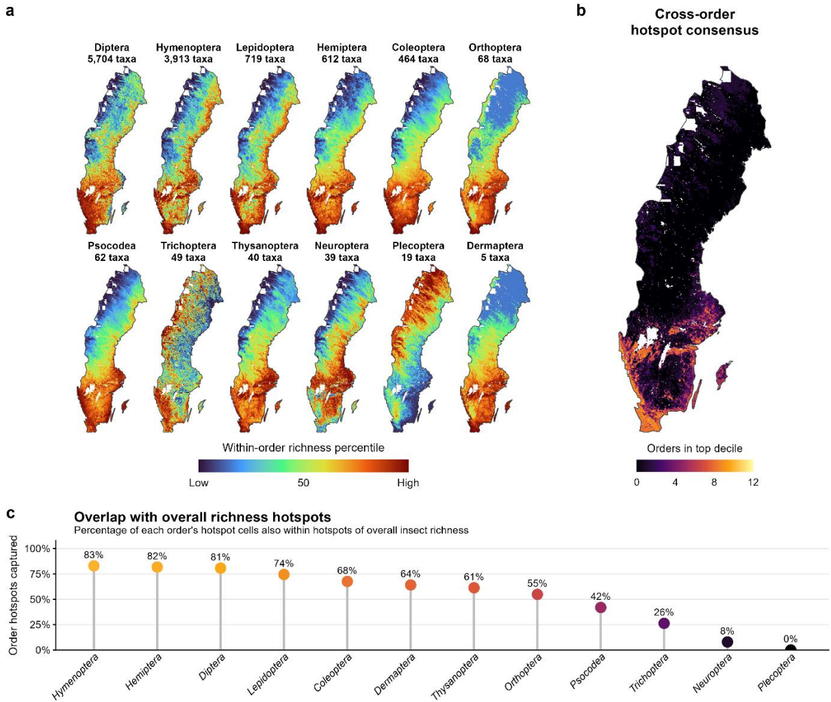
Figure 3: Order-specific richness patterns and hotspot overlap across Sweden. a) Predicted richness patterns for 12 insect orders, expressed as within-order richness percentiles to allow comparison among orders differing strongly in the number of modelled taxa. The number of modelled taxa is shown for each order. b) Cross-order hotspot consensus, showing the number of orders for which each approximately 2-km grid cell fell within the upper 10% of predicted richness values for that order. c) Overlap between order-specific richness hotspots and hotspots based on overall insect richness. Values show the percentage of hotspot cells for each order that were also classified as richness hotspots for all insect taxa combined. Hotspots were defined separately for each order, and for all insects, as cells at or above the corresponding 90th percentile.
