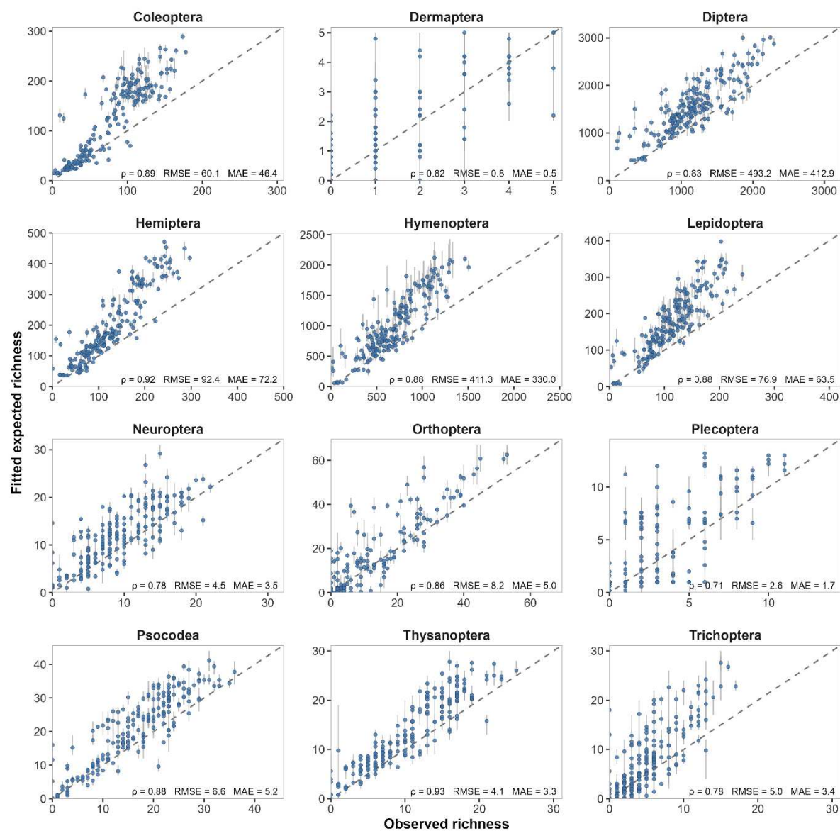
1137 Extended Data Figure 1: Correspondence between observed and predicted insect richness across sampling sites. Observed 1138 richness at Malaise traps is shown against predicted richness for each of 12 insect orders. Predicted richness was obtained by 1139 converting taxon-level occurrence probabilities to presence-absence predictions using taxon-specific F1 thresholds and summing 1140 these predictions within each order. Points show the mean predicted richness across the five selected joint species distribution 1141 models, and vertical lines show the minimum-to-maximum range across these models. Dashed lines indicate the 1:1 1142 relationship. Spearman's rank correlation coefficient ( \rho ), root mean squared error (RMSE) and mean absolute error (MAE) were 1143 calculated from the mean prediction across the five models. Because models were fitted using the full dataset, these 1144 comparisons describe correspondence at sampled sites rather than independent predictive performance.
