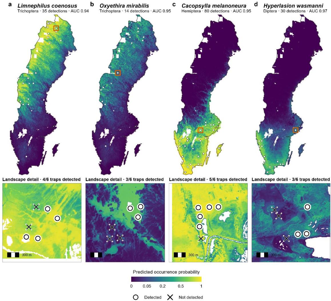
Figure 4: Contrasting taxon-level distributions connect national and landscape-scale patterns of insect diversity. a-d) Predicted occurrence probability at the national scale (upper row) and within selected multi-trap landscapes at 10-m resolution (lower row) for Limnephilus coenosus (a), Oxyethira mirabilis (b), Cacopsylla melanoneura (c) and Hyperlasion wasmanni (d). Predictions show the mean occurrence probability across the five selected joint species distribution models for each order. Taxa were selected to represent contrasting northern, southern, broad and spatially restricted distribution patterns while retaining informative local variation. White circles on the national maps indicate sampling locations at which the taxon was detected, and orange squares locate the corresponding landscape panels. In the local panels, circles indicate detections and crosses indicate non-detections at Malaise traps. AUC values are mean site-grouped cross-validated AUC values across the five selected models. All panels use a common probability scale; the color scale is square-root transformed for visualization, while legend labels report untransformed occurrence probabilities.
