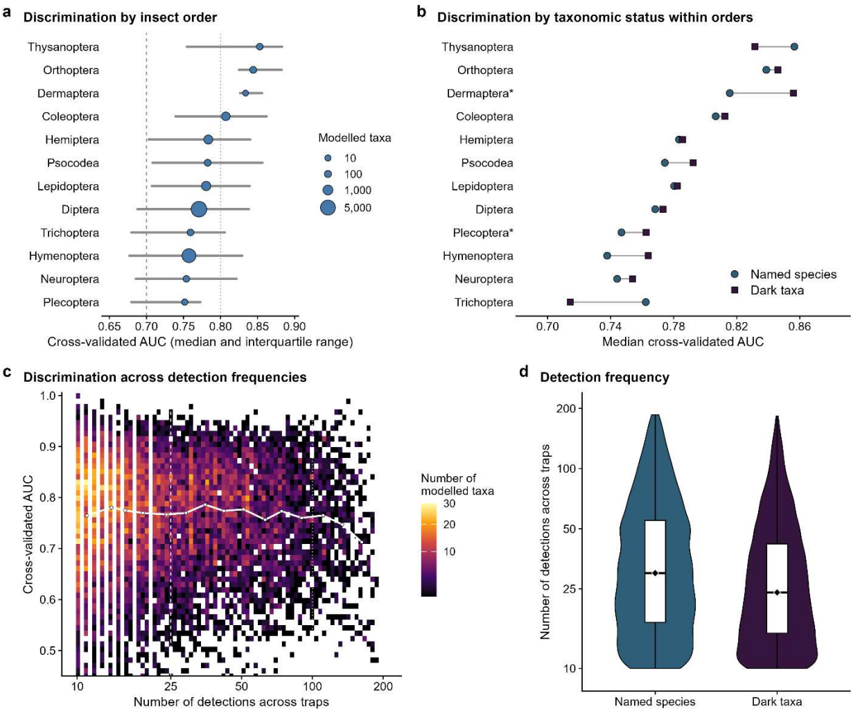
Extended Data Figure 2: Cross-validated model discrimination across insect orders, detection frequencies and taxonomic status. a) Median site-grouped cross-validated area under the receiver operating characteristic curve (AUC; points) and interquartile range (horizontal lines) for taxa in each of 12 insect orders. Point size indicates the number of modelled taxa; vertical reference lines mark AUC values of 0.7 and 0.8. b) Median cross-validated AUC for named species and dark taxa within each insect order. Dark taxa are defined here as molecular clusters lacking species-level taxonomic assignments. Lines connect the two taxonomic groups within orders. Asterisks indicate orders for which either the named-species or dark-taxon group contained fewer than ten taxa. c) Relationship between the number of trap detections and cross-validated AUC across all 11,694 modelled taxa. Color indicates the number of taxa in each two-dimensional bin, and the white line connects median AUC values for logarithmically spaced detection-frequency bins containing at least 50 taxa. Vertical reference lines mark 25 and 100 detections. d) Distribution of detection frequencies for 5,160 named species and 6,534 dark taxa. Violins show the distributions, white boxes show the interquartile ranges and diamonds indicate the medians; detection frequency is shown on a logarithmic scale.
