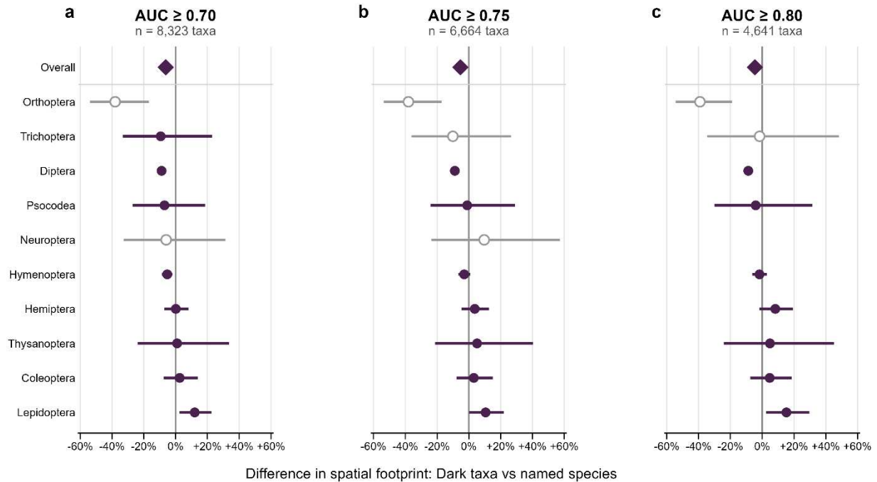
Extended Data Figure 4: Robustness of dark-taxon spatial-footprint differences to model-performance filtering. a-c) Differences in predicted spatial footprint between dark taxa and named species after progressively restricting analyses to taxa with cross-validated AUC \geq 0.70 (a), \geq 0.75 (b) and \geq 0.80 (c). Spatial footprint was quantified as the area required to contain 90% of a taxon's predicted probability mass. Diamonds show the overall dark-taxon vs. named-species difference estimated across insect orders, and circles show order-specific differences; horizontal lines indicate 95% confidence intervals. Negative values indicate smaller spatial footprints for dark taxa than for named species. Filled circles denote comparisons represented by at least ten named species and ten dark taxa, whereas open circles denote comparisons with 5–9 taxa in at least one group; order-level comparisons with fewer than five taxa in either group are not shown. The numbers above each panel give the total number of taxa retained at the corresponding AUC threshold.
