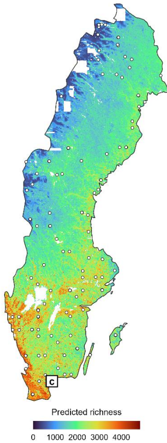
Figure 1: A national map of insect diversity across Sweden. a) Predicted total insect richness across Sweden based on joint species distribution models fitted separately for 12 insect orders. National predictions were generated for 2 million randomly sampled 10-m cells and averaged within approximately 2-km grid cells for visualization at the national scale. Open circles show sampling sites, and the box marks the landscape shown in c. b) Taxonomic scope of the mapped insect diversity across orders, showing the number of mapped insect taxa and the contributions of named species versus unnamed DNA sequence clusters, i.e., dark taxa. c) Predicted insect richness within an example landscape at the original 10-m prediction grain. Circle size and fill show observed richness at Malaise traps.
