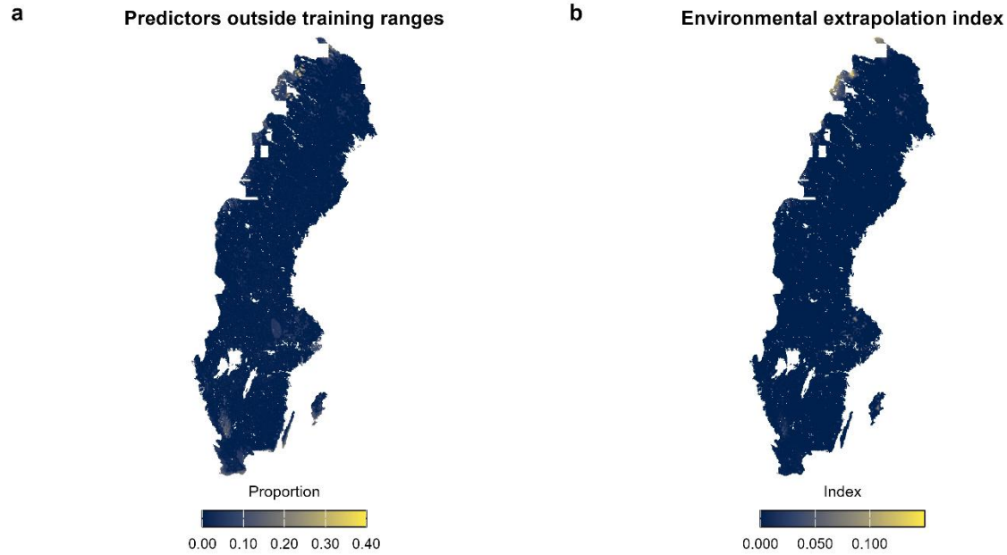
Extended Data Figure 5: Environmental extrapolation in national insect predictions. a) Proportion of the 20 environmental predictors for which conditions in each mapped cell fell outside the range represented by the sampling network. b) Environmental extrapolation index, calculated as the mean normalized distance beyond the corresponding training range across the environmental predictors. Higher values indicate cells in which predictions rely more strongly on environmental extrapolation. At least one predictor fell outside its training range across 43.5% of mapped land, but only 1.5% of the area had at least 3 predictors outside their training ranges and 0.6% exceeded an extrapolation index of 0.05. Stronger extrapolation was concentrated locally, particularly in northern and northwestern Sweden.
