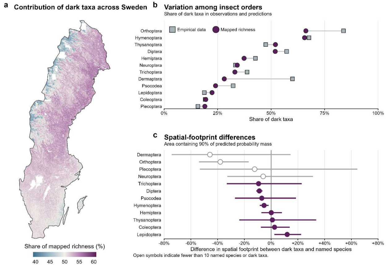
Figure 2: Dark taxa make a substantial contribution to mapped insect diversity. a) Spatial variation in the contribution of dark taxa to mapped insect richness across Sweden, expressed as the percentage of mapped richness represented by dark taxa. b) Variation among insect orders in the share of modelled taxa represented by dark taxa and their contribution to mapped richness. Squares show the proportion of modelled taxa that were dark taxa and circles show the proportion of mapped richness contributed by dark taxa; lines connect the two estimates within each order. c) Order-specific differences in spatial footprint between dark taxa and named species, quantified as the area required to contain 90% of predicted probability mass. Points show estimated percentage differences between dark taxa and named species and horizontal lines show 95% confidence intervals; negative values indicate smaller spatial footprints for dark taxa. Open symbols indicate orders represented by fewer than ten named species or dark taxa. Across all 12 orders, 11,694 taxa were mapped, comprising 5,160 named species and 6,534 dark taxa.
