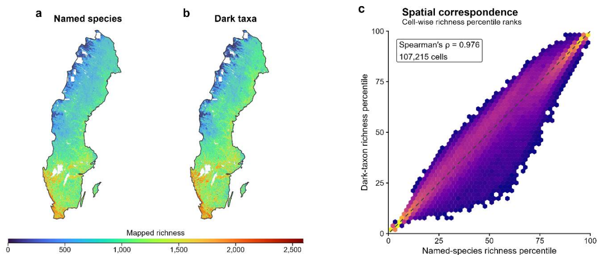
1161 Extended Data Figure 3: Spatial correspondence between mapped richness of named species and dark taxa. a,b) Mapped 1162 richness of named species (a) and dark taxa (b), defined here as molecular clusters lacking species-level taxonomic assignments, 1163 across Sweden. Both maps are shown on the same color scale. National predictions were generated for 2 million randomly 1164 sampled 10-m cells distributed across Sweden and averaged within approximately 2-km grid cells for national-scale visualization. 1165 c) Cell-wise correspondence between named-species and dark-taxon richness, expressed as percentile ranks across mapping 1166 cells. Hexagon color indicates the number of mapping cells, and the dashed line shows the 1:1 relationship.
