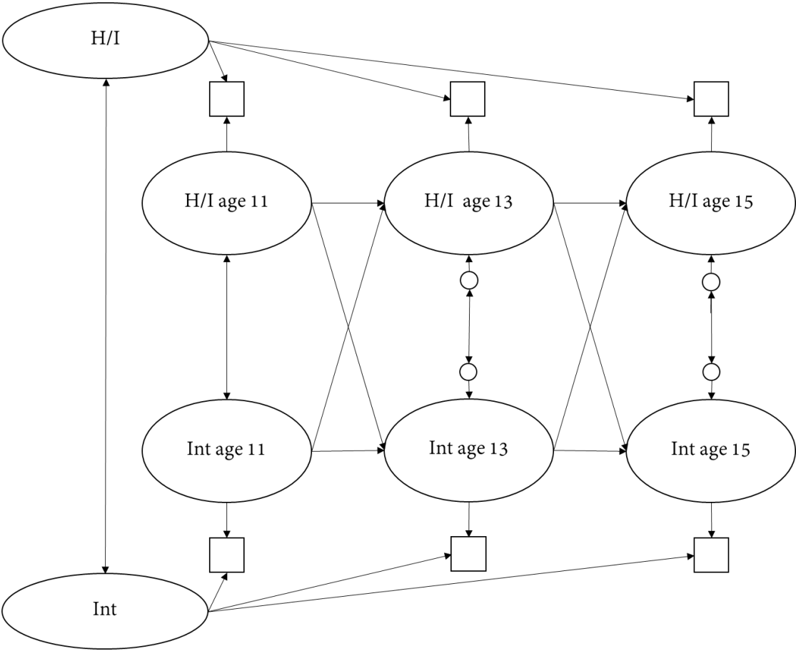
Figure 1: Example RI-CLPM
