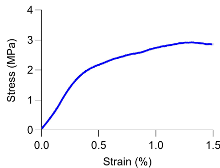
Figure 4. Structural and mechanical characterization of the spatially matched iliac bone biopsy. (a) MicroCT reconstruction of the biopsy showing internal microarchitecture and segmentation of cortical and trabecular compartments. (b) Unconfined compression testing of the same biopsy following microCT imaging. (c) Representative stress–strain response obtained during compression testing.
