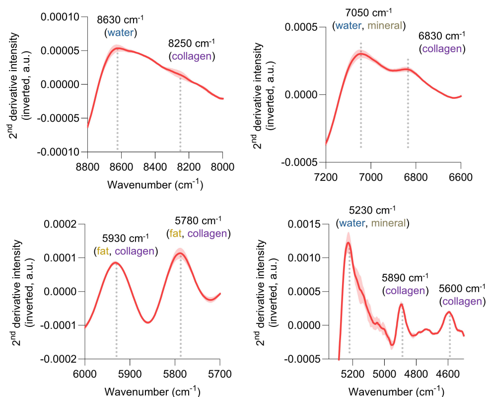
Figure 3. NIR spectra acquired directly from the intact iliac bone biopsy site. (a) Intact-surface NIR spectrum showing characteristic absorption features associated with major bone constituents. (b) Second-derivative spectra highlighting selected spectral peaks associated with water, mineral, collagen, and fat. Shaded regions represent the standard deviation across replicate spectra.
