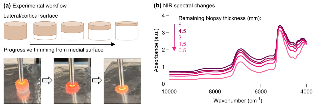
Figure 5. Influence of underlying tissue on intact-surface NIR spectra. (a) Serial trimming workflow in which tissue was progressively removed from the medial surface while NIR spectra were repeatedly acquired from the unchanged lateral cortical surface. (b) Intact-surface NIR spectra at decreasing remaining biopsy thicknesses, showing systematic spectral changes as underlying tissue was removed.
