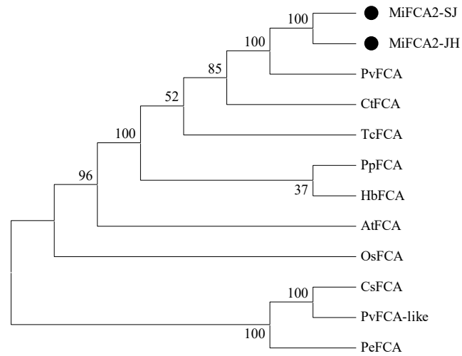
Supplemental Fig. 1 A phylogenetic tree of FCA proteins. the FCA proteins information (species and gene names) were as follows: MiFCA2-SJ ( Mangifera indica ), MiFCA2-JH ( Mangifera indica ), PvFCA ( Pistacia vera ), CtFCA ( Citrus trifoliata ), TcFCA ( Theobroma cacao ), PpFCA ( Prunus persica ), HbFCA ( Hevea brasiliensis ), AtFCA ( Arabidopsis thaliana ), OsFCA ( Oryza sativa ), CsFCA ( Citrus sinensis ), PvFCA-like ( Pistacia vera ), PeFCA ( Populus euphratica )
