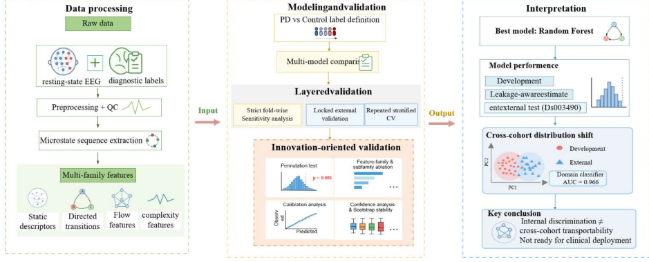
Fig. 1 Analytical framework for multi-family EEG microstate marker evaluation. The study separates exploratory within-cohort discrimination, leakage-aware internal validation, and locked external testing, followed by cross-cohort distribution-shift analysis.
