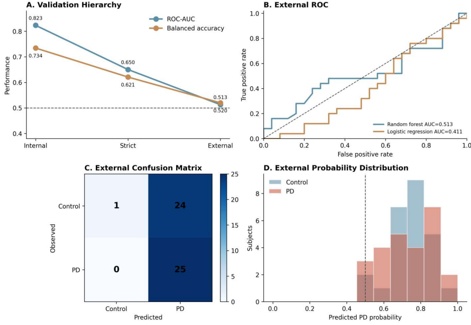
Fig. 9 Locked external validation on OpenNeuro ds003490. A, validation hierarchy from exploratory repeated CV to leakage-aware fold-wise evaluation and independent testing. B–D, external ROC curves, random-forest confusion matrix, and predicted-probability distributions. The near-chance external performance provides the principal evidence that the development signal was not robustly transportable.
