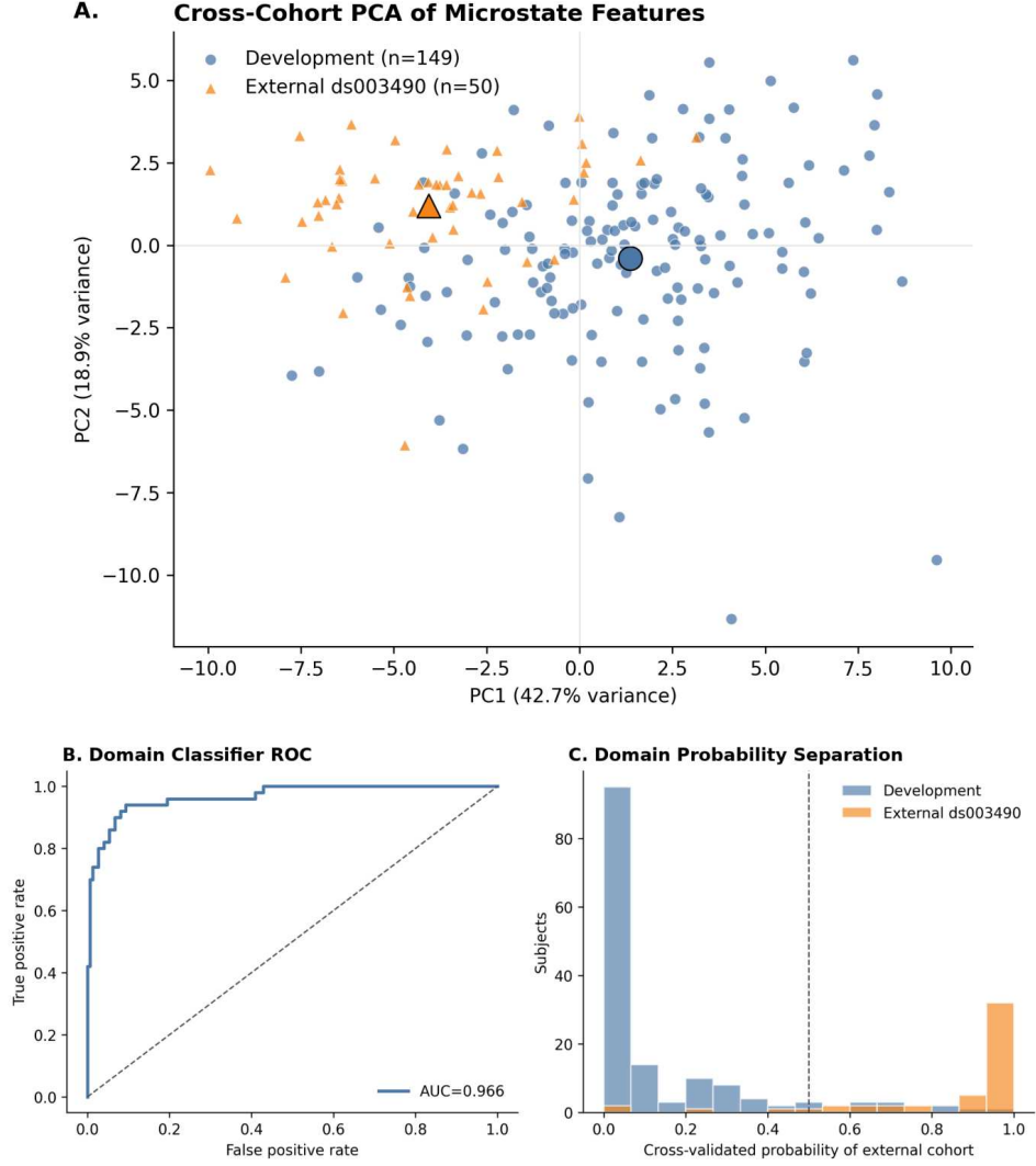
Fig. 10 Cross-cohort distribution shift in the multi-family microstate feature space. A, principal component analysis of development and external participants. B, cross-validated dataset-origin ROC curve. C, dataset-origin probability distributions. The dataset-origin ROC-AUC of 0.966 indicates strong cohort separability and provides a feature-space explanation for limited external transportability.
