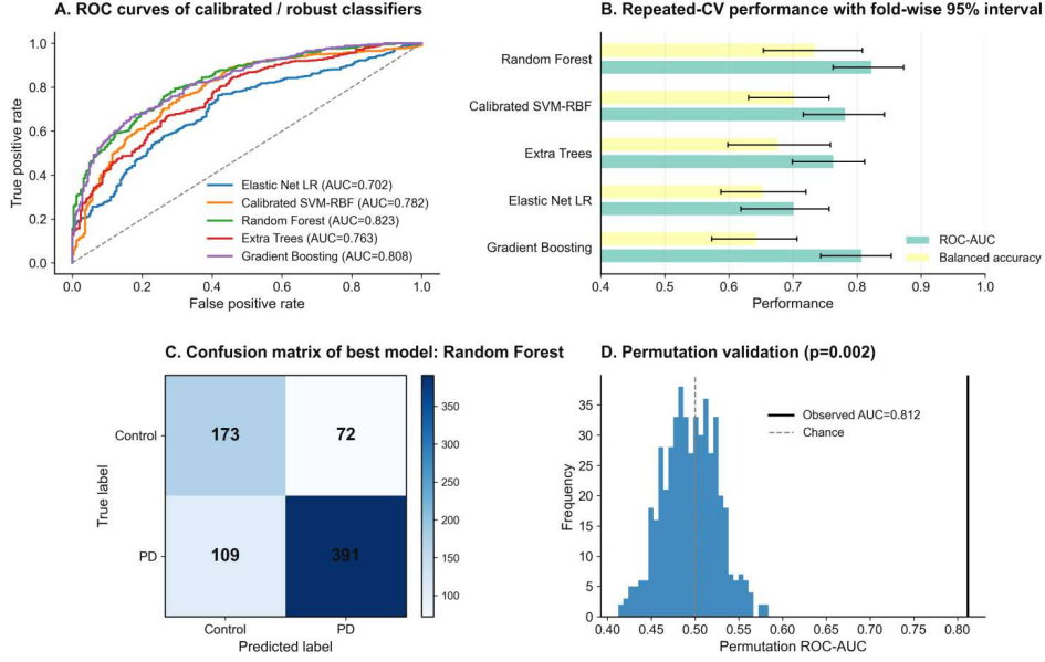
Fig. 5 Exploratory within-cohort discrimination using the multi-family microstate feature set. A, ROC curves across evaluated classifiers. B, repeated-CV ROC-AUC and balanced accuracy. C, repeated-CV confusion summary for the random forest model; counts represent accumulated out-of-fold predictions across the five repeated cross-validation runs rather than unique participants. D, permutation-based comparison with shuffled-label performance. These panels characterize development-cohort signal and are not evidence of external diagnostic validity.
