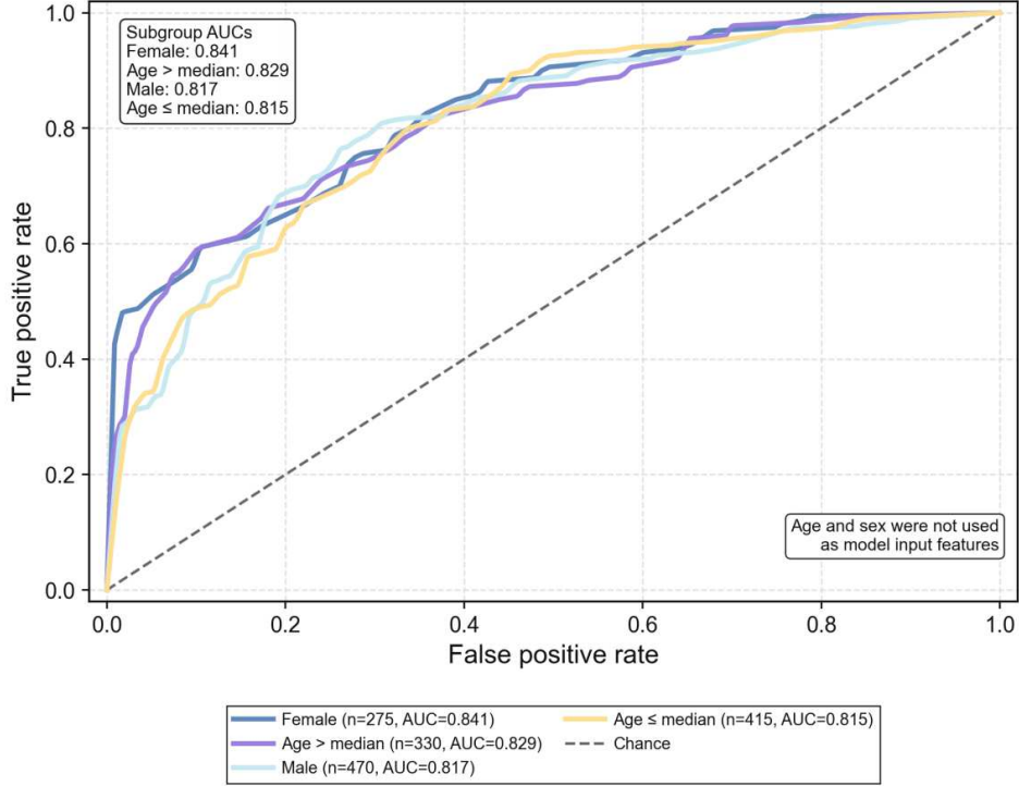
Fig. 8 Supporting demographic sensitivity analysis. ROC curves compare development-cohort performance across sex and age strata; similar subgroup AUCs indicate that the internal discrimination was not obviously concentrated in one tested demographic subgroup.
