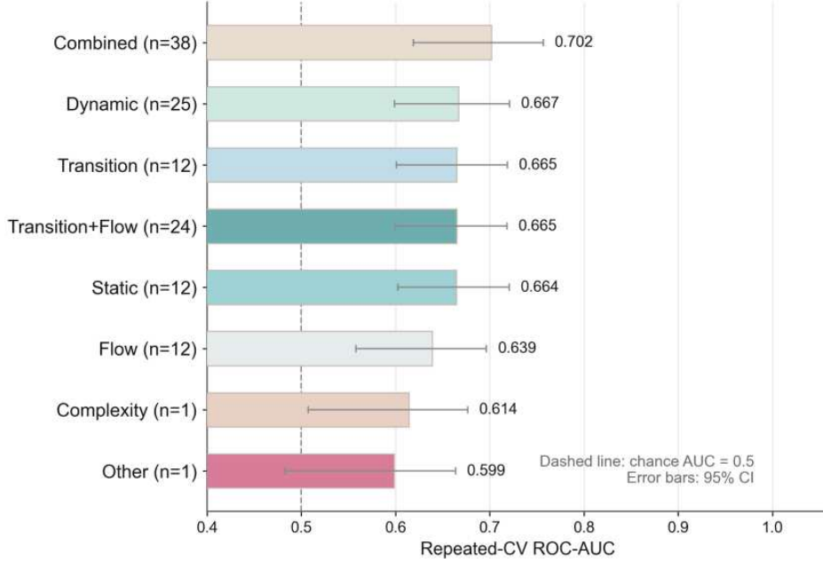
Fig. 6 Feature-family ablation under the dedicated family-comparison configuration. The combined representation retained the highest ROC-AUC among the tested feature families, supporting a distributed contribution across static and dynamic descriptors. Error bars indicate 95% confidence intervals; very small feature families should be interpreted descriptively.
