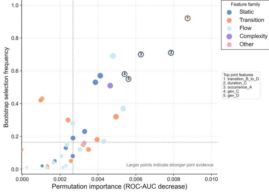
Fig. 7 Joint model-level feature importance and resampling stability. The x-axis shows the decrease in ROC-AUC after feature perturbation, and the y-axis shows bootstrap top-feature selection frequency. Features toward the upper-right contributed more strongly and were selected more consistently, but these quantities do not establish biological causality.
