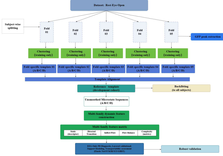
Fig. 3 Fold-aware microstate template estimation, backfitting, and multi-family feature construction. The feature representation combines static, directed-transition, flow, and complexity information before marker evaluation.
