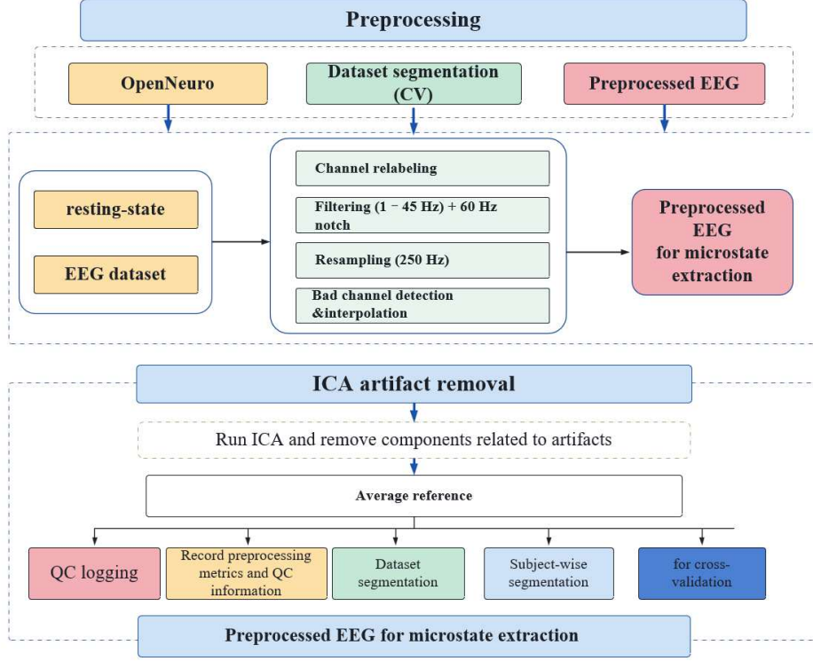
Fig. 2 Preprocessing and participant-level quality-control workflow applied before microstate extraction and feature construction.
