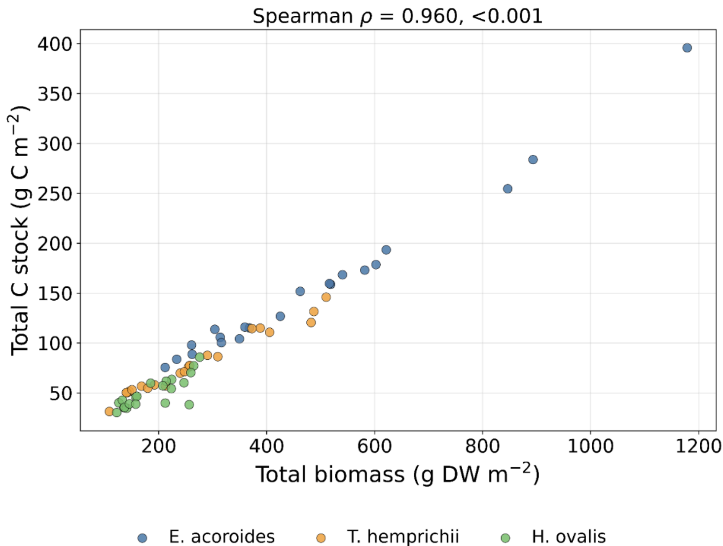
Figure 8 Relationship between total biomass and total biomass-based carbon stock for the three dominant seagrass species. Points are distinguished by species. Complete Spearman correlation coefficients are presented in Table S8.
