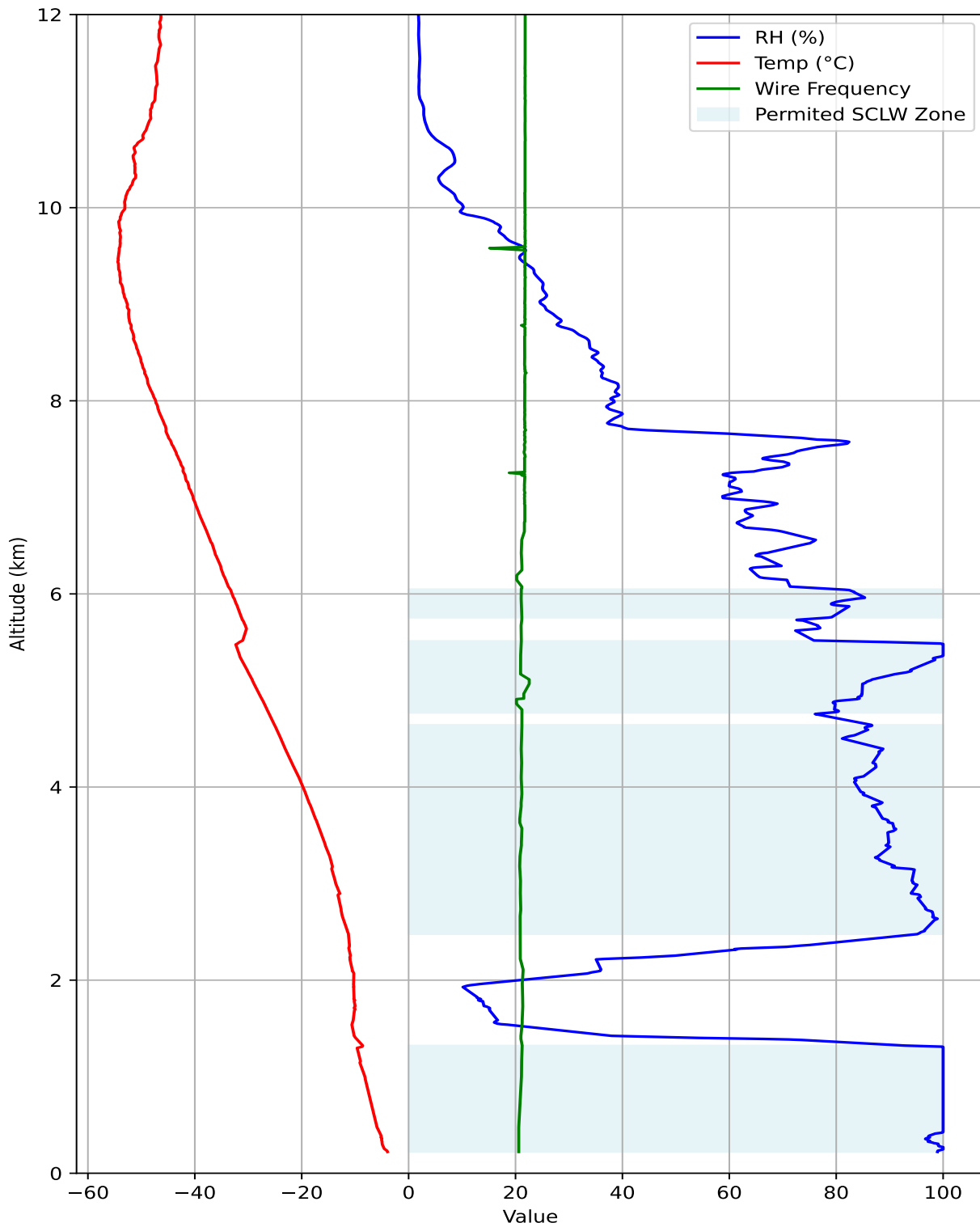
Example of a usable SLWC-probe profile without a plausible non-zero SLWC detection. The vibrating-wire frequency remains sufficiently stable for instrumental screening, but does not show localized perturbations within a thermodynamically favorable SLWC layer. Shading indicates the permitted SLWC zone, defined as in Figure 9.
