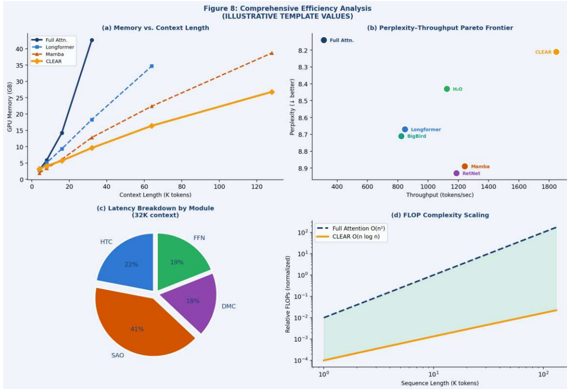
Fig. 8. Comprehensive efficiency analysis: (a) GPU memory vs. context length; (b) perplexity-throughput Pareto frontier showing CLEAR dominates all baselines; (c) latency breakdown by module; (d) theoretical FLOP scaling showing O(n \log n) vs. O(n^2) complexity.
