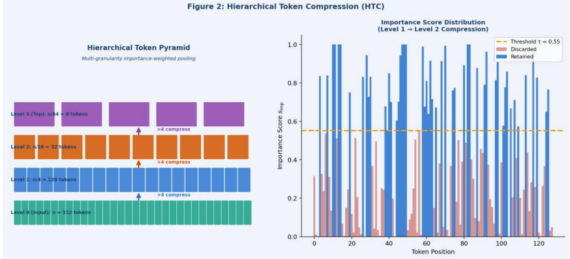
Fig. 2. Hierarchical Token Compressor (HTC): (left) multi-granularity token pyramid with 4x compression at each level; (right) importance score distribution showing retained (blue) vs. discarded (red) tokens at level-1 compression.
