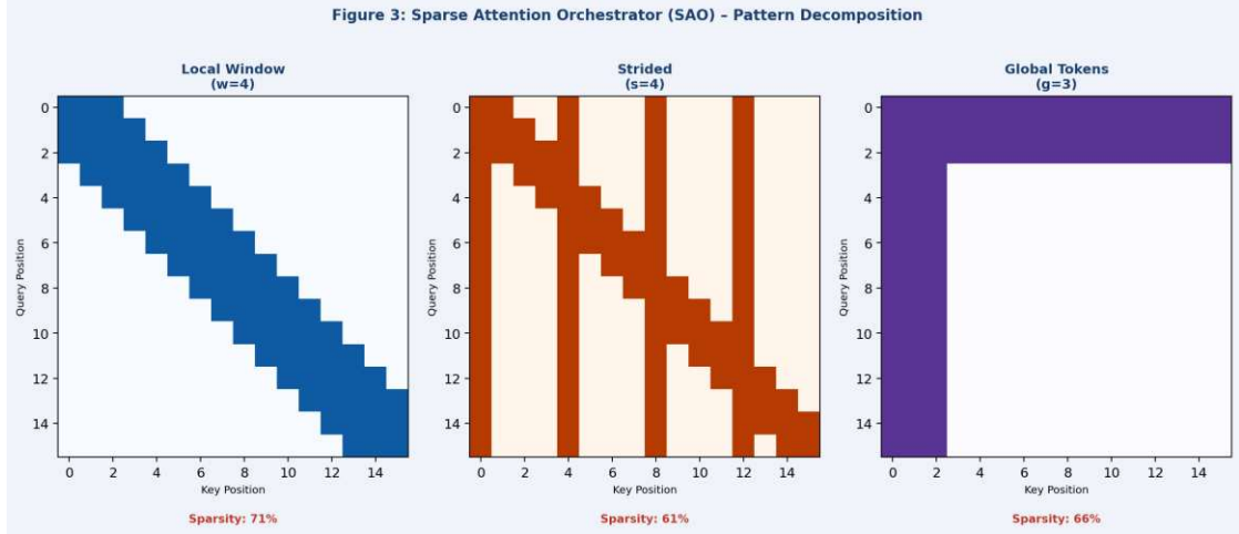
Fig. 3. Sparse Attention Orchestrator (SAO) pattern decomposition: local window attention (left), strided pattern (center), and global token attention (right). Combined sparsity achieves 85% FLOP reduction over full attention at 32K context.
