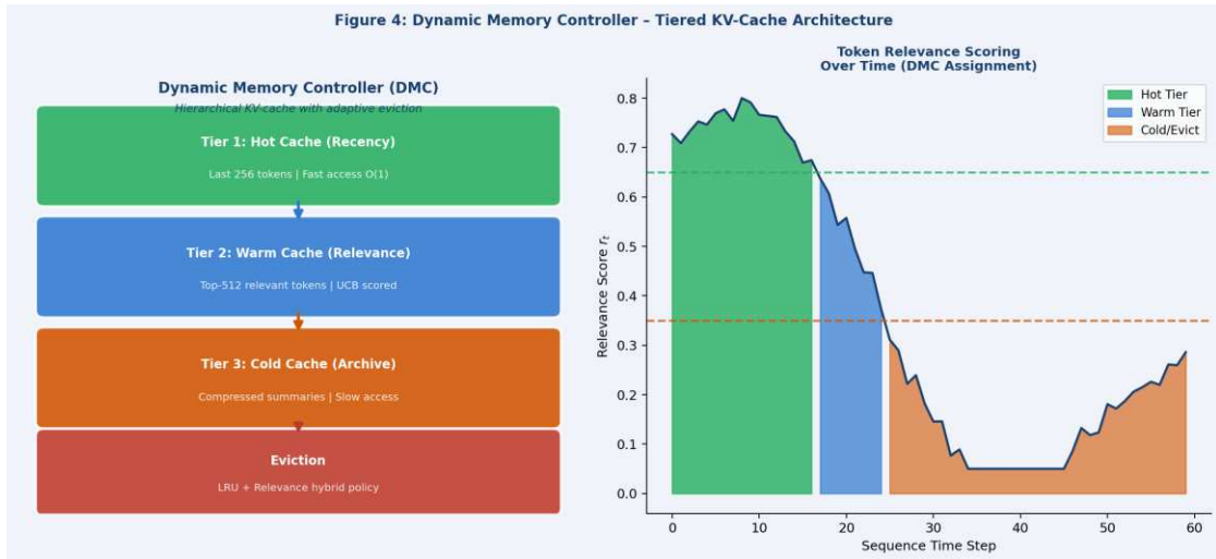
Fig. 4. Dynamic Memory Controller (DMC): (left) three-tier KV-cache architecture with hot (recency), warm (relevance), and cold (archive) tiers; (right) token relevance scoring over time showing tier assignment dynamics.
