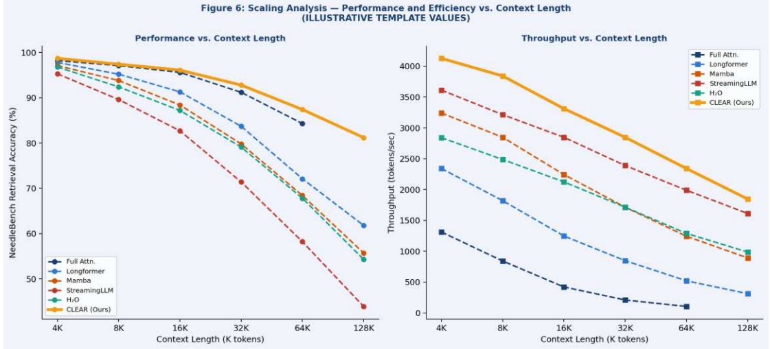
Fig. 6. Scaling analysis with context length (4K–128K tokens): (left) NeedleBench retrieval accuracy showing CLEAR maintaining 81.2% at 128K where full attention runs out of memory; (right) throughput comparison demonstrating super-linear efficiency gains.
