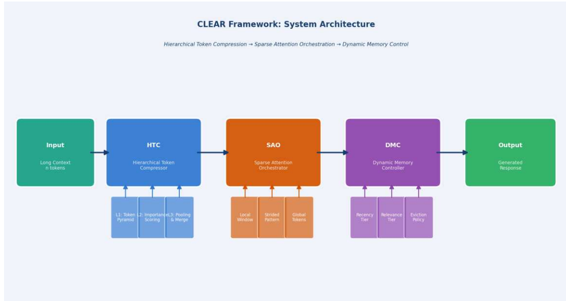
Fig. 1. CLEAR framework system architecture: end-to-end pipeline from long-context input through the Hierarchical Token Compressor (HTC), Sparse Attention Orchestrator (SAO), and Dynamic Memory Controller (DMC) to generated response.
