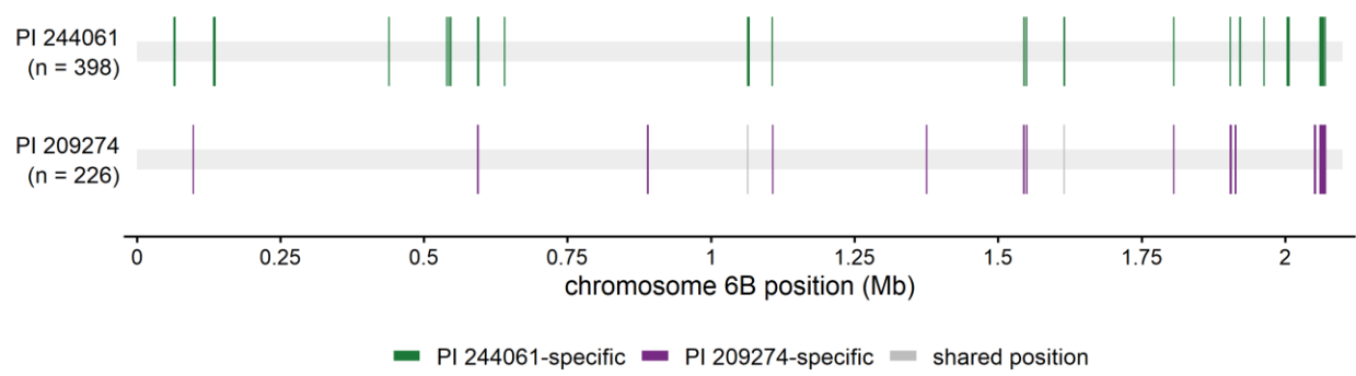
Fig. S1 Comparison of SNP-based haplotypes in the chromosome 6BS resistance interval between PI 244061 and PI 209274. Vertical lines indicate SNP positions
