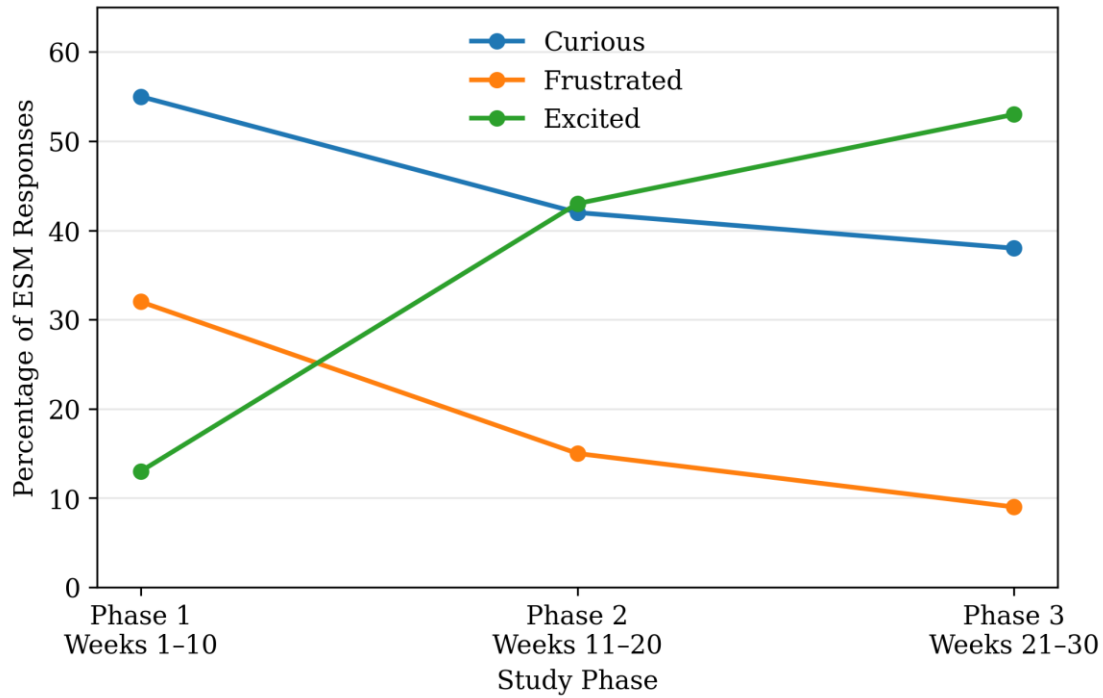
Fig. 8 ESM Affective-State Trends Across Study Phases
