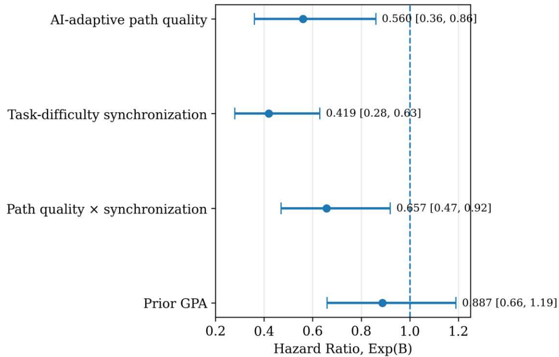
Fig. 3 Cox Regression Hazard Ratios for Student Persistence
