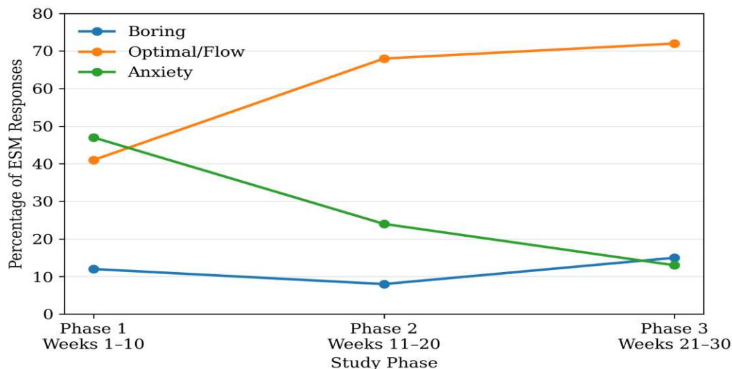
Fig. 7 ESM Difficulty-State Trends Across Study Phases
