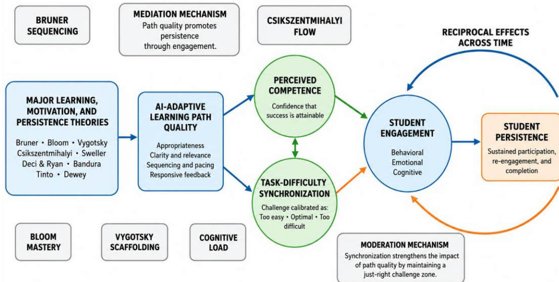
Fig. 1 Conceptual Model of AI-Adaptive Learning Path Quality, Task-Difficulty Synchronization, Student Engagement, and Persistence
