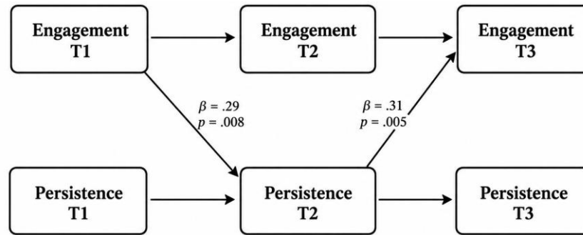
Fig. 6 Longitudinal Feedback Loop Between Engagement and Persistence
