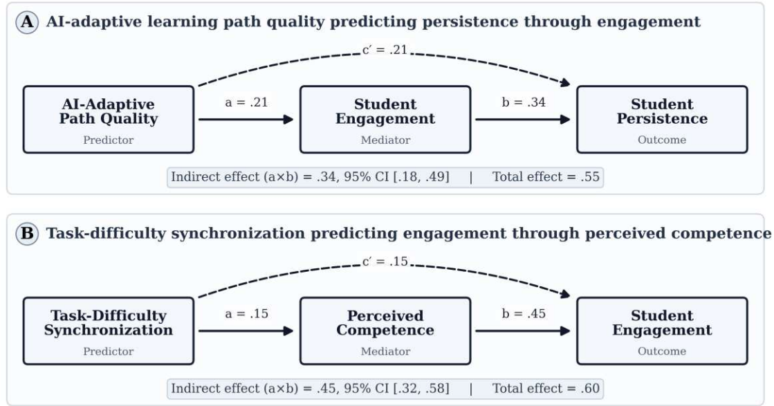
Fig. 5 Path Analysis and Mediation Model
