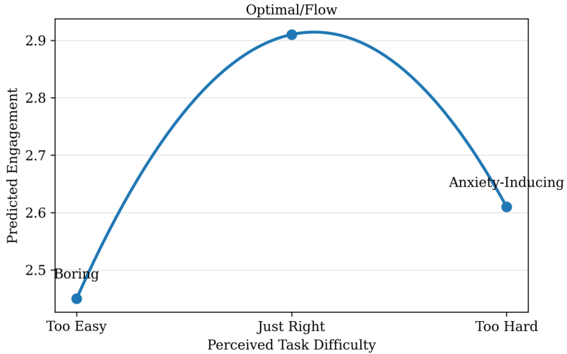
Fig. 4 Curvilinear Flow Arch Between Task Difficulty and Engagement
