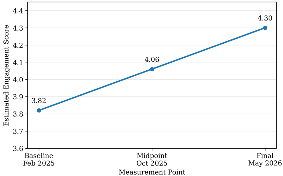
Fig. 2 Latent Growth Trajectory of Student Engagement
