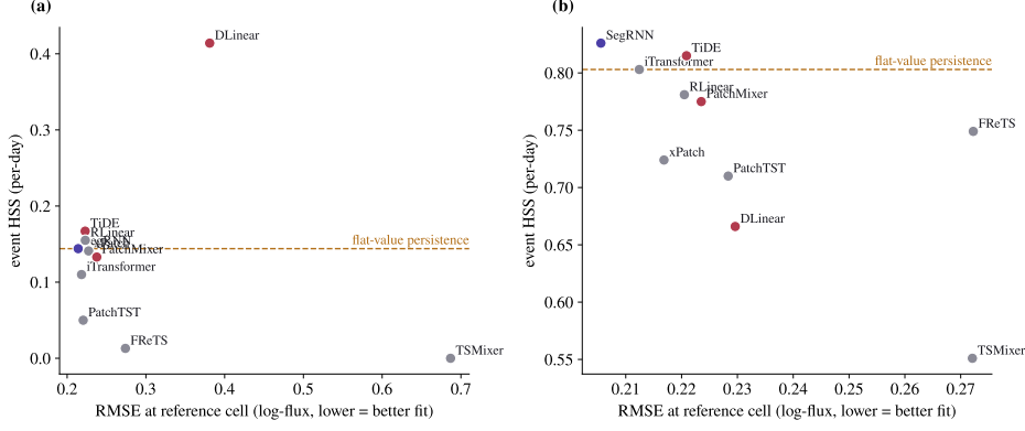
Fig. 4 Accuracy and event skill decouple only for impulsive events. Per-model reference-cell RMSE ( x ) versus per-day event HSS ( y ); the dashed line marks flat-value persistence. (a) On the impulsive SXR target the lowest-RMSE model (SegRNN) sits on the persistence floor while a worse-RMSE model (DLinear) attains higher event skill. (b) On the persistent proton target the two axes re-couple. Reference fold (fold 0); cross-fold intervals are in Supplementary Table S5.
