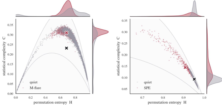
Fig. 1 Two dynamical regimes (complexity–entropy plane). The left panel shows the XRS 1–8 Å target; the right panel the proton \geq 10 MeV target. The \times marker locates the per-regime mean. The central scatter plots permutation entropy H versus statistical complexity C for sliding sequence-length windows (within the theoretical C_{\min}/C_{\max} envelope), with per-axis kernel-density-estimate marginals by regime. Proton quiet windows concentrate in the high- H , low- C noise corner (mean H, C = 0.95, 0.09 ); SPE windows shift to lower entropy and higher complexity (0.91, 0.15). For XRS the two regimes share almost the same entropy (mean H \approx 0.68 ) but M-flare windows sit at markedly higher complexity ( C rising from 0.23 to 0.31).
