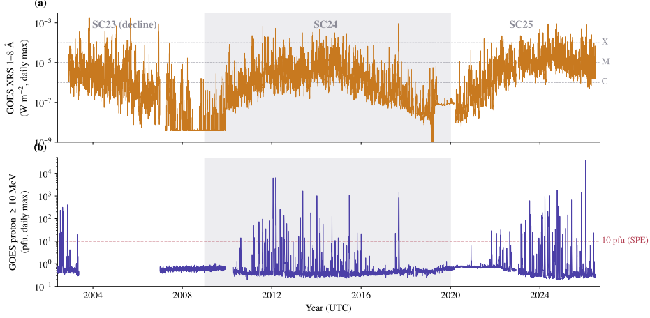
Fig. 5 Data overview. Daily-maximum GOES observations across the benchmark span. (a) The soft X-ray 1–8 Å flux ( xrs_long ), with the C, M, and X flare thresholds marked; (b) the \geq 10 MeV integral proton flux ( p.gt10 ), with the 10 pfu solar-proton-event threshold. Coverage runs from the declining phase of solar cycle 23, through the full cycle 24 (shaded), to the rise of cycle 25.
