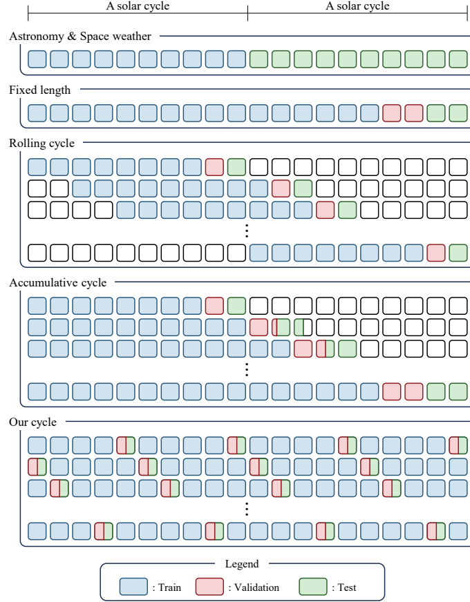
Fig. 6 Evaluation split protocols. Train (blue), validation (red), and test (green) assignment over two solar cycles for five schemes: the chronological astronomy/space-weather holdout, a fixed-length holdout, rolling-origin (walk-forward) cross-validation, expanding-window (accumulative) cross-validation, and the interleaved atomic-term rotation used here (bottom). Only the last keeps every fold’s train, validation, and test sets spanning all cycle phases while remaining leakage-controlled.
