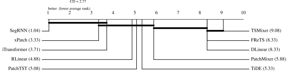
Fig. 2 Critical-difference diagram of the RMSE ranking. Average rank of each model over the N = 24 fold-averaged benchmark configurations spanning the four horizons 3, 6, 12, 24 h (Friedman \chi^2_9 = 150.3 , p < 10^{-27} ); lower is better, and models joined by a bar differ by less than the Nemenyi critical difference ( CD = 2.77 , \alpha = 0.05 ). SegRNN holds rank 1.04, first in 23 of the 24 configurations; it joins the top cluster of xPatch and iTransformer within the critical difference and is separated by more than the critical difference from the remaining models. xPatch, divergent at the longest (7-day) historical horizon, is ranked on the fully populated historical horizons.
