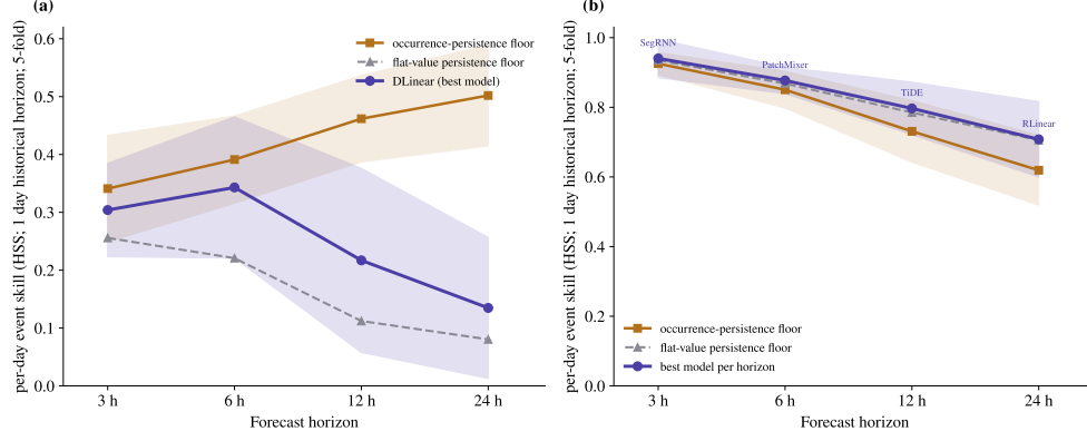
Fig. 3 Event skill versus forecast horizon. Best-model per-day M-class HSS (5-fold mean, 95% CI band) against the occurrence-persistence and flat-value persistence floors, at the 1-day (reference) historical horizon, for (a) soft X-ray and (b) proton. On soft X-ray the shortfall to occurrence-persistence closes as the horizon shortens, reaching parity at 3–6 h, and the best event-skill model is DLinear at every horizon; on proton the model tracks both floors at every horizon. Per-day granularity (the operational contingency unit), not the per-point aggregate of Supplementary Fig. S4.
