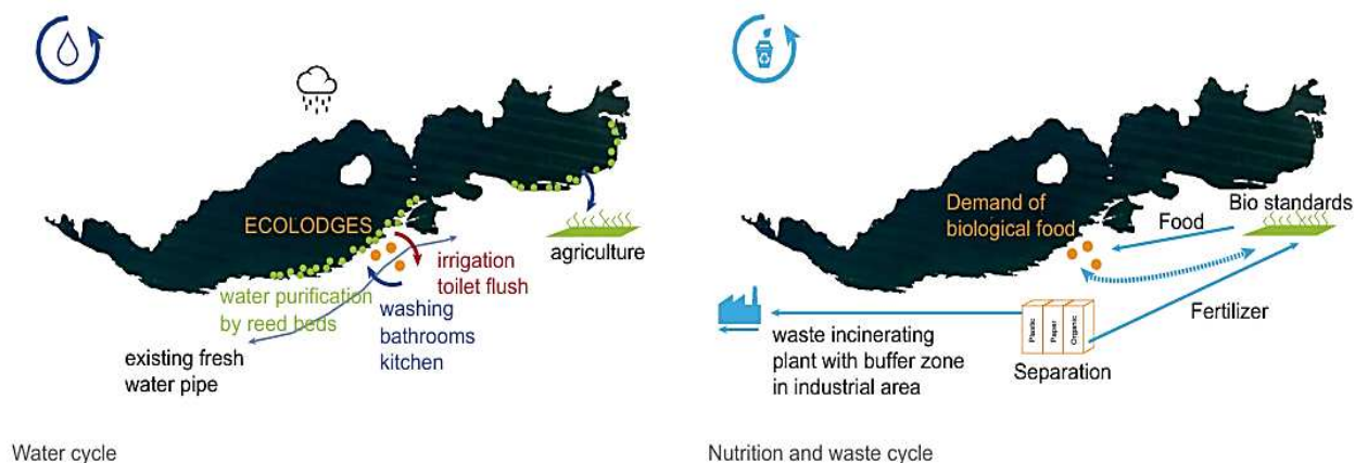
Fig.3 (a ,b) : Showing a satellite image of the Fayoum Oasis area
